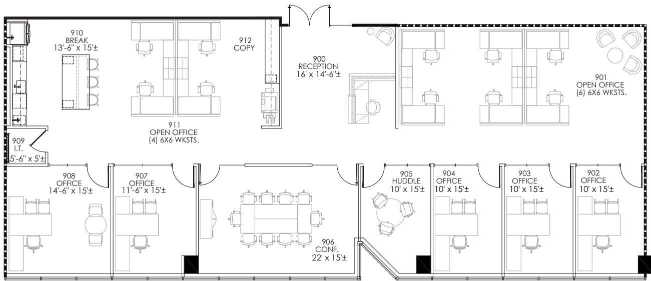
KEY PLAN
