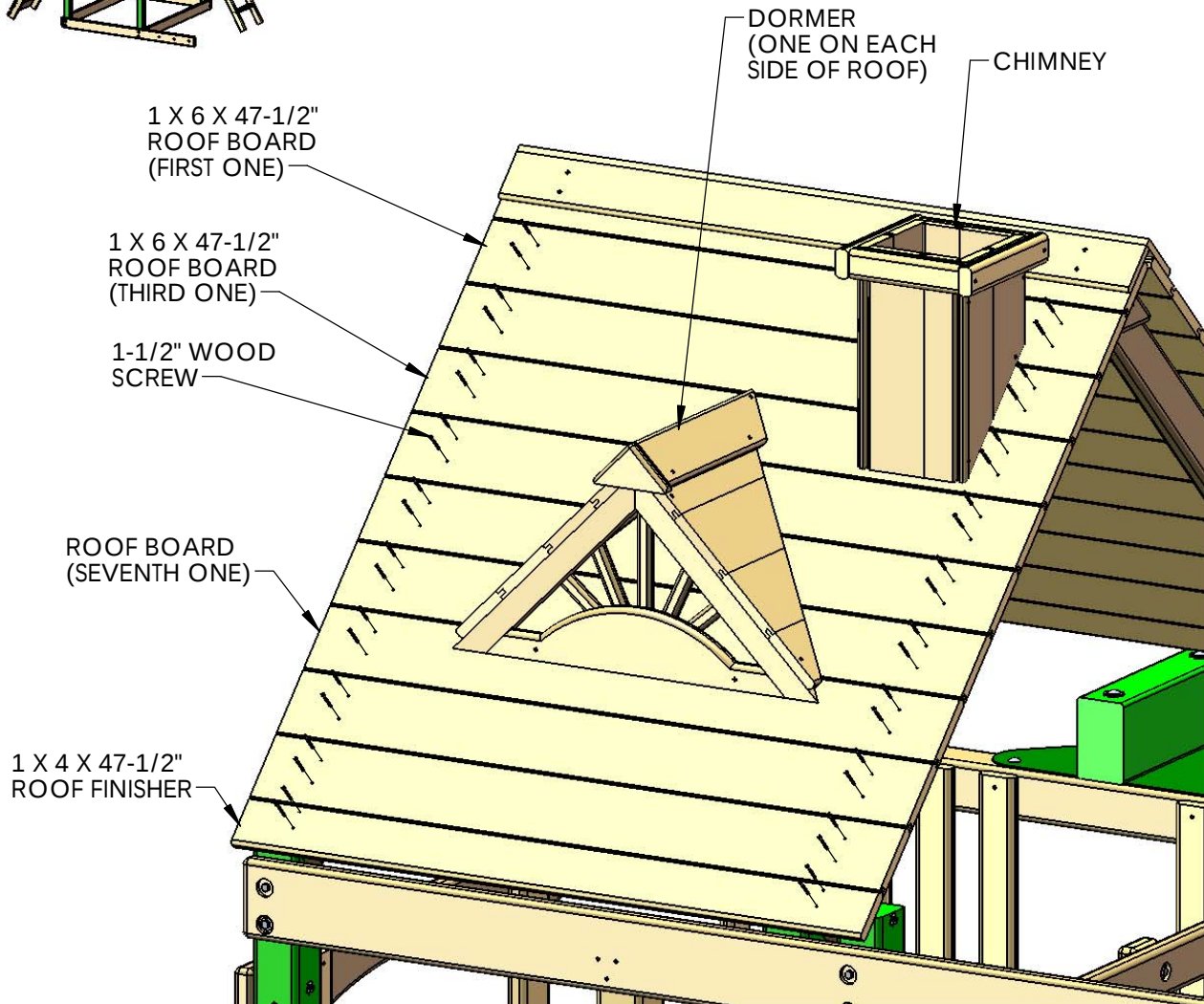
DETAIL C SCALE 1 : 12
