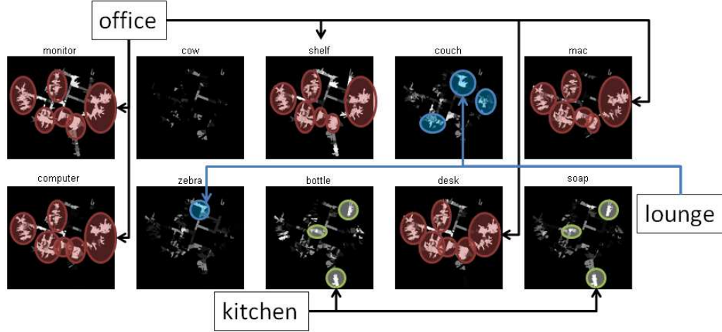
Figure 3-4: The above image shows probability maps for ten different unknown object categories: monitor, cow, shelf, couch, mac, computer, zebra, bottle, desk and soap. White is higher probability, darker is lower probability for each of these objects. For each of the objects, we have highlighted the locations where the algorithm correctly predicted these objects for office, lounge and kitchen areas. For example, we can see that the algorithm properly locates the soap in the kitchen (we did not map bathrooms) and that computers are correctly located in office areas.
