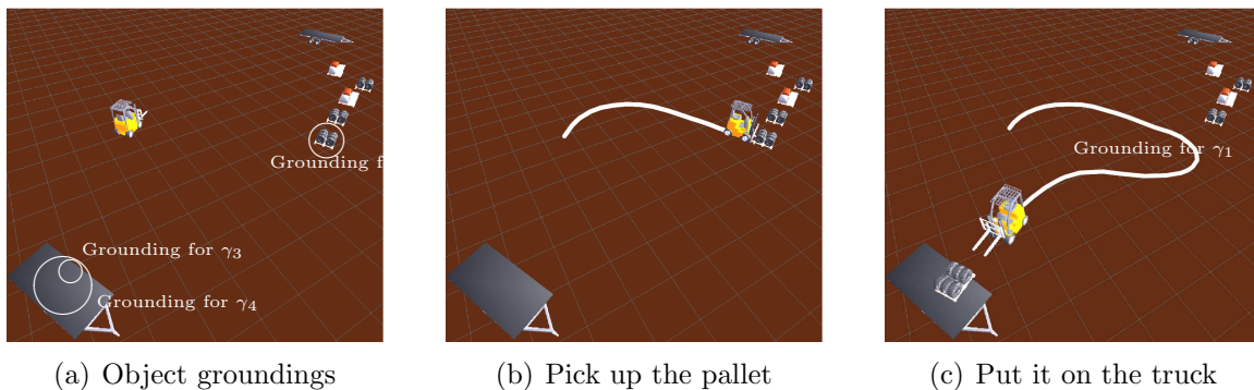
Figure 5-7: A sequence of the actions that the forklift takes in response to the command, “Put the tire pallet on the truck.” In (a) the search grounds objects and places in the world based on their initial positions. In (b) the forklift executes the first action, and picks up the pallet. In (c) the forklift puts the pallet on the trailer.
