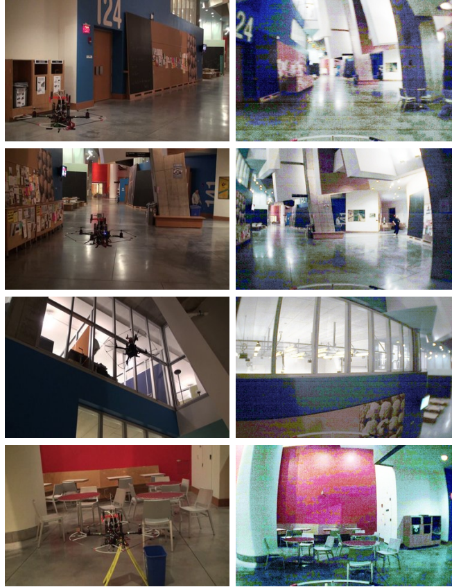
Figure 4-12: (left) Photographs of the MAV executing an interactive series of instructions. (right) Imagery from the on-board camera, transmitted to the operator as the MAV flies. The commands issued to the MAV are given in the text.
