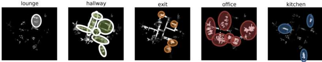
Figure 3-5: The above image shows probability maps for five different unknown place categories: lounge, hallway, exit, office and kitchen. White is higher probability, darker is lower probability for each of these places. For each of the places, we have highlighted the locations where the algorithm correctly predicted these objects for each place category. For example, we can see that the algorithm properly locates kitchens and offices, but is unable to locate the exits.
