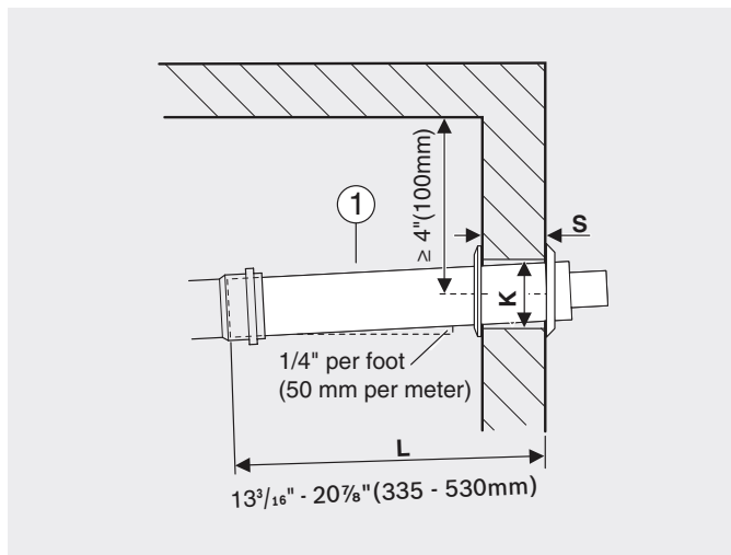
Fig. 6 Penetration through the outside wall
