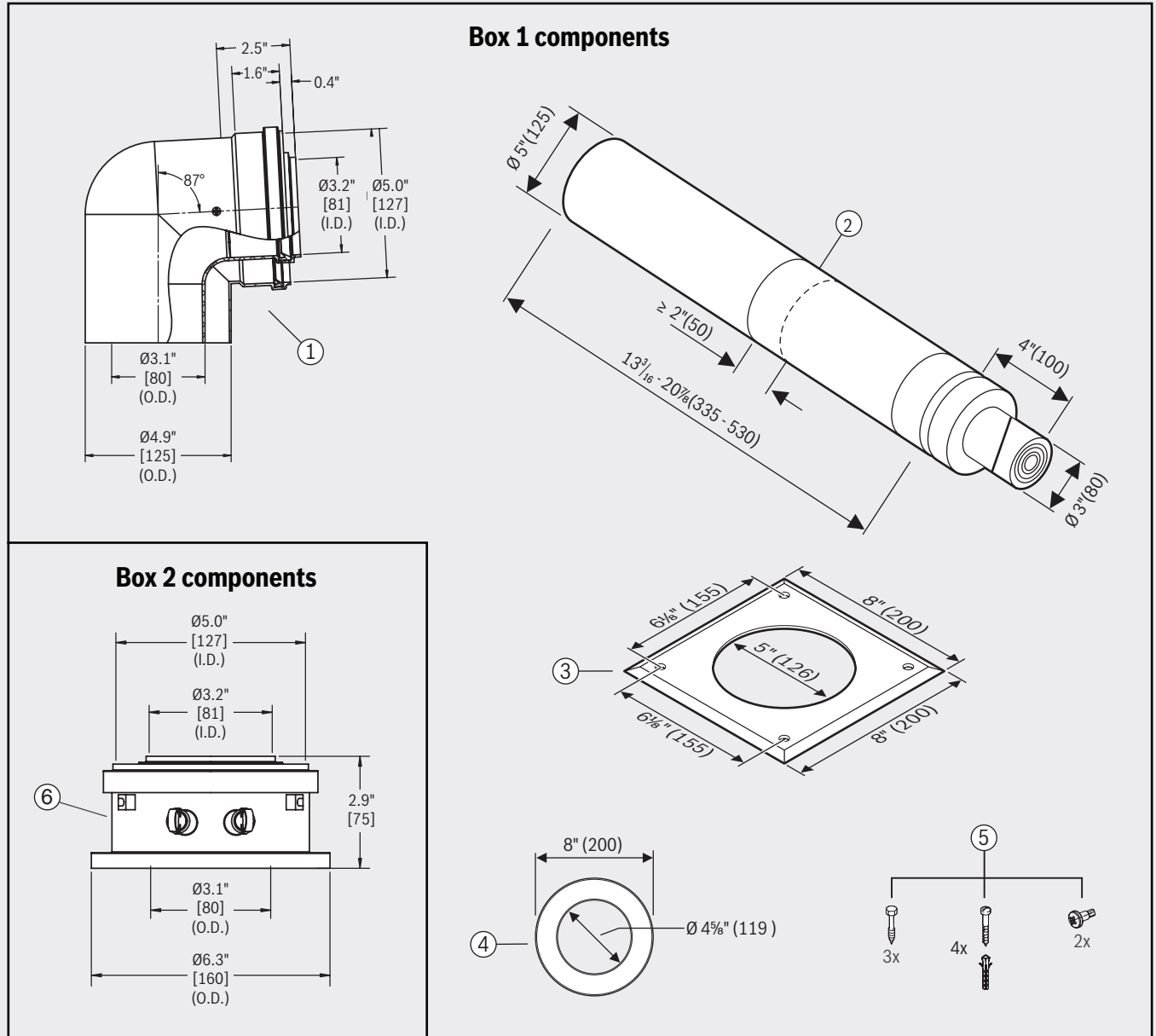
Fig. 1 Scope of delivery - dimensions in inches (mm)
