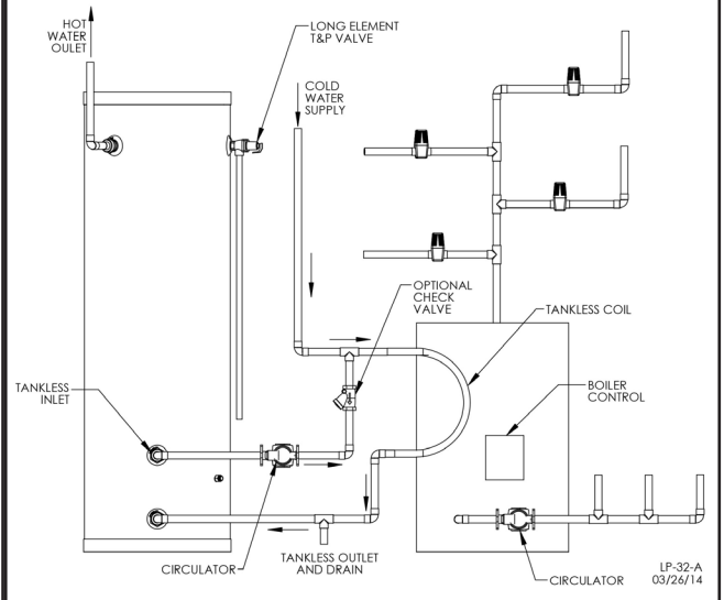
Figure 4 - Typical Storage Tank Installation - SSU-80CB and SSU-119CB Models
