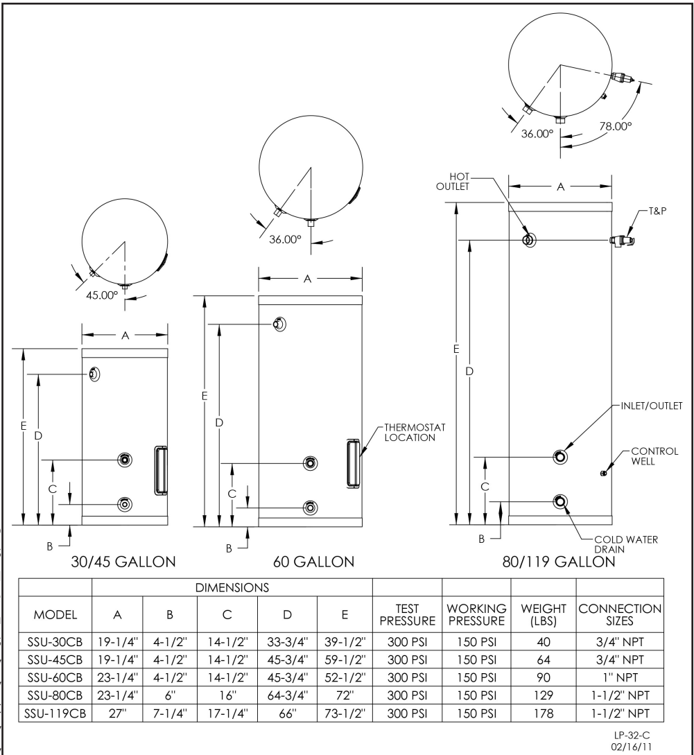
Figure 2 - Specifications and Dimensions
