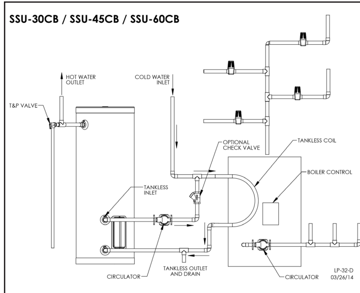
Figure 3 - Typical Storage Tank Installation - SSU-30CB - SSU-60CB Models
