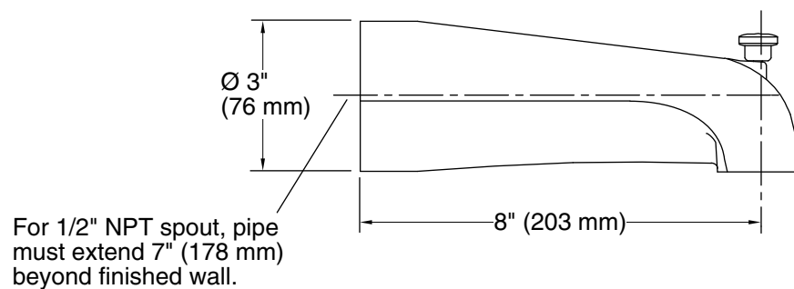
Product Diagram
