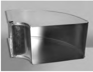
#120 Flat 90° Elbow
