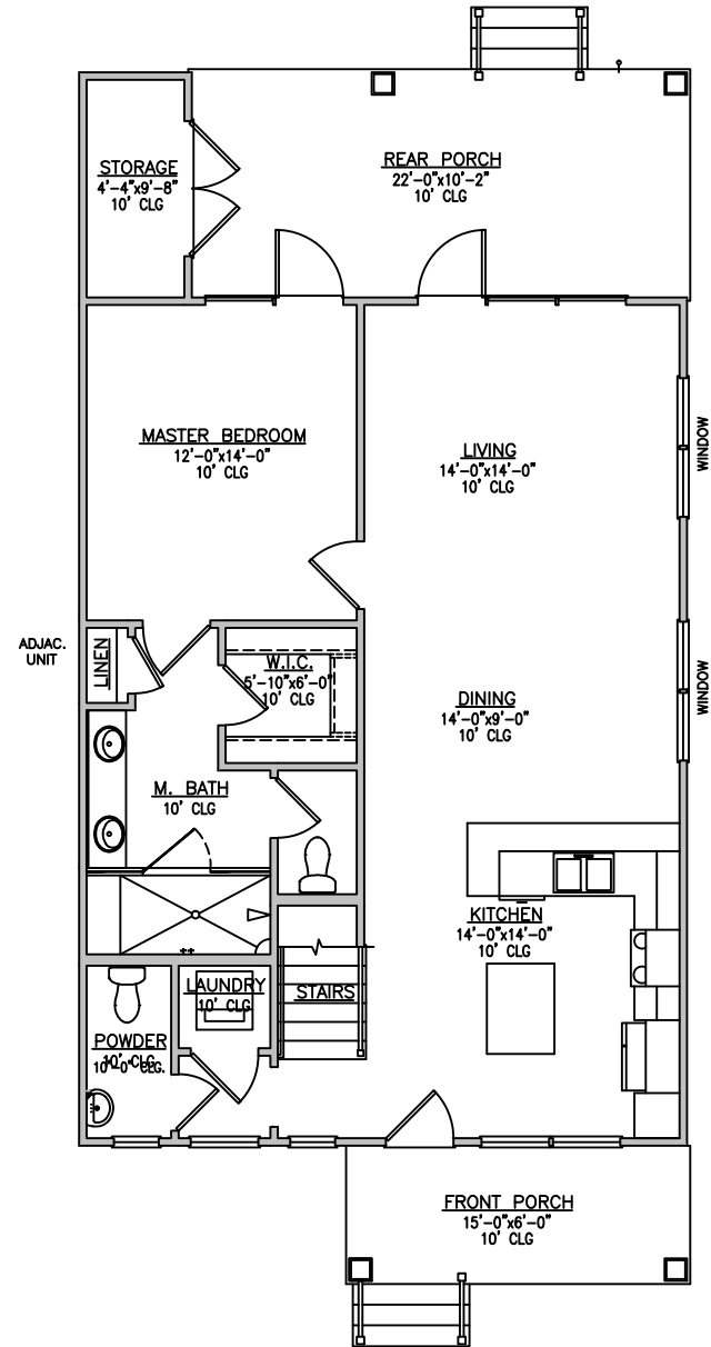
HERON - 1st FLOOR RIGHT END UNIT
