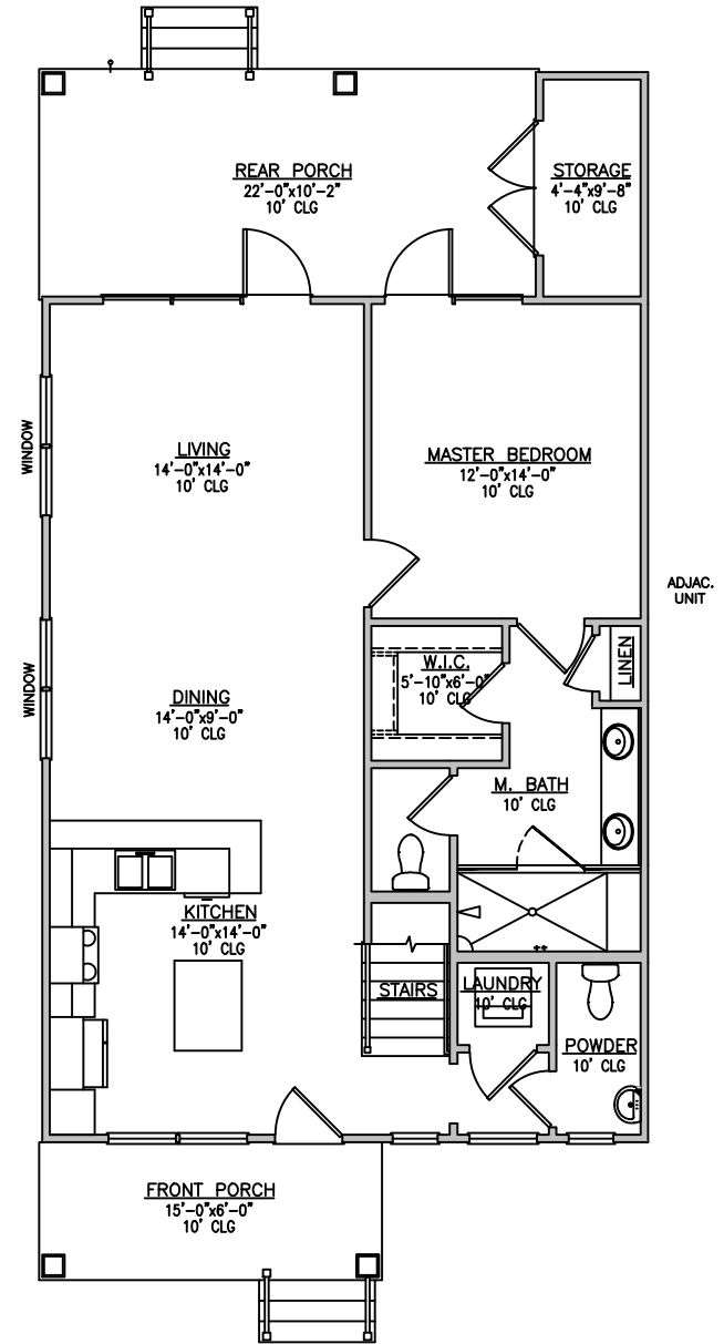
HERON - 1st FLOOR LEFT END UNIT
