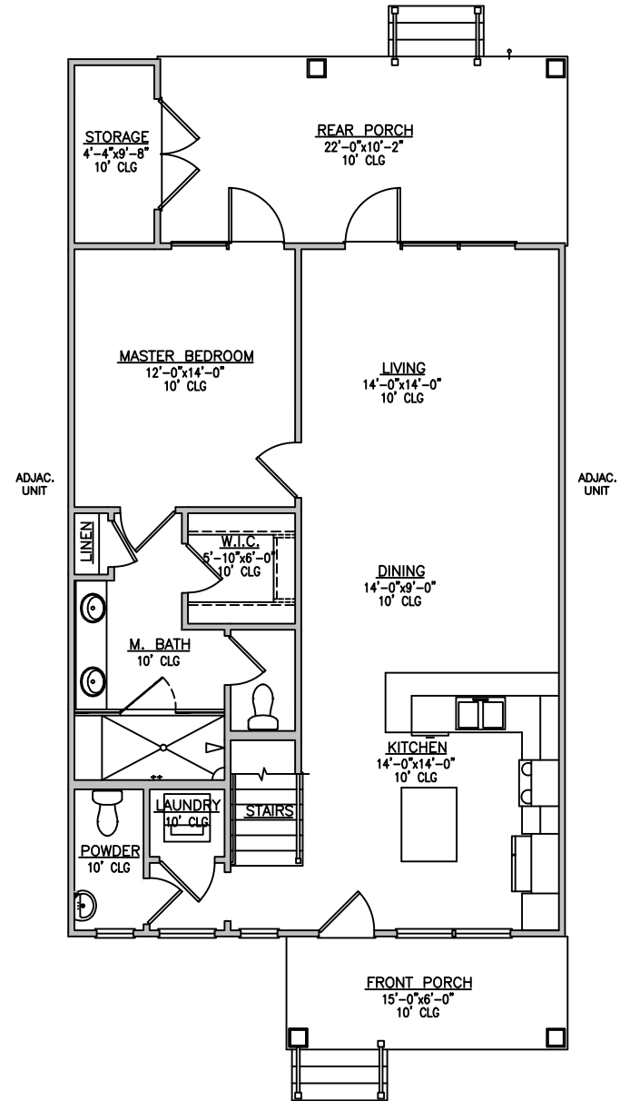
HERON - 1st FLOOR INTERIOR UNIT
