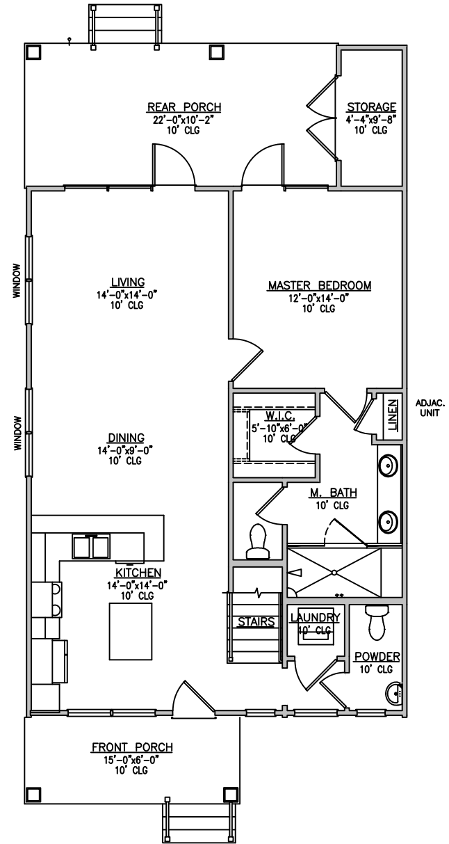
HERON - 1st FLOOR LEFT END UNIT
