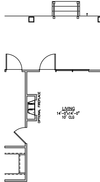
HERON - 1st FLOOR FIREPLACE OPTION 2
