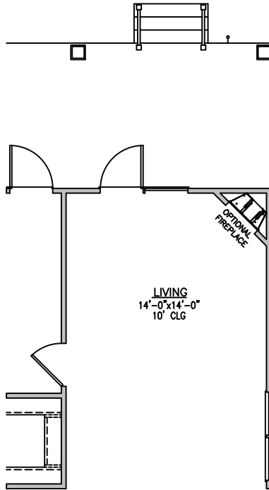
HERON - 1st FLOOR FIREPLACE OPTION 1
