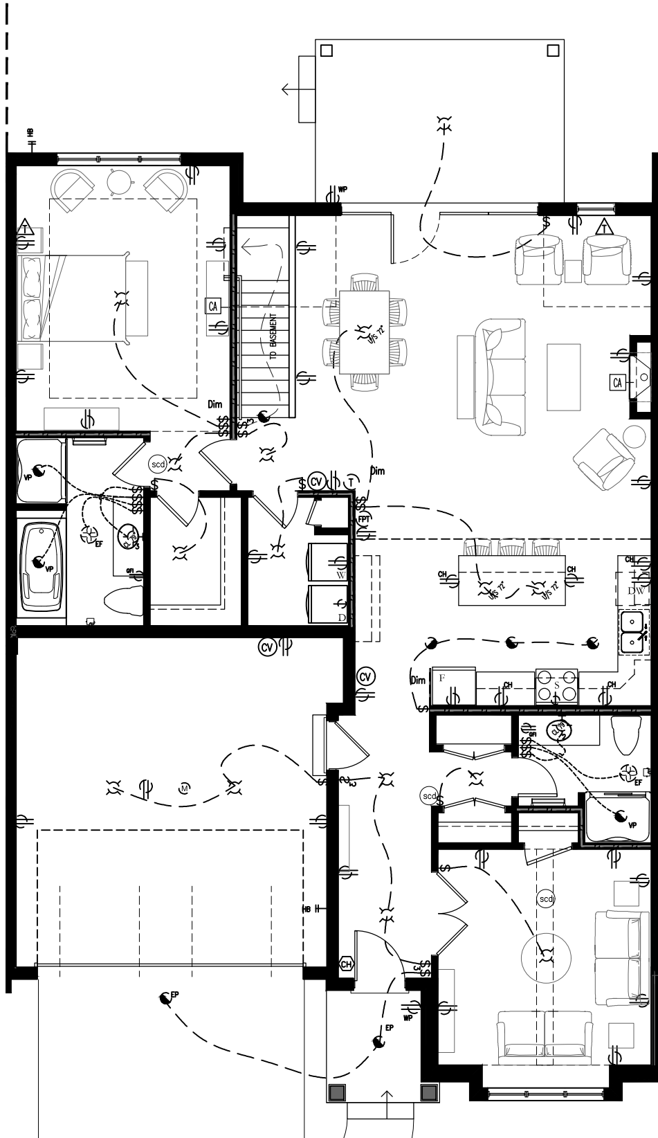
Linden (interior) Main Floor Plan Electrical Layout scale: 1/8" = 1'-0"
