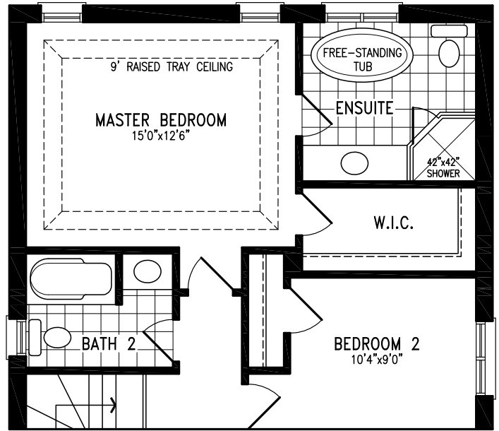
PART. OPT. SECOND FLOOR W/3RD BATH
