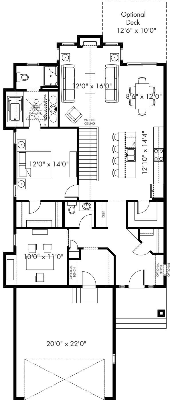
main floor 1402 SQ FT
