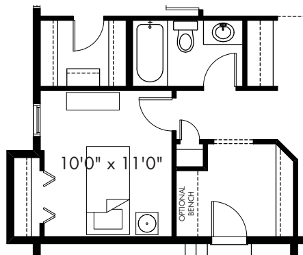
PARTIAL MAIN FLOOR PLAN WITH OPTIONAL SECOND BEDROOM & 3 PIECE BATHROOM (Adds 0 Sq. Ft. to Main Floor)
