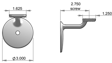
HB-1 – Handrail bracket complete w/lag cover. – Shown w/Lag-1.
