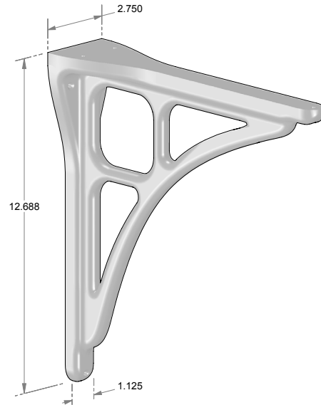
BKT-12 – Corner bracket.
