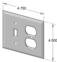
EC-600 – Switchplate/outlet combination plate.
