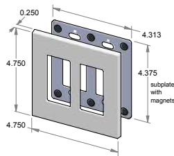
EC-9302M – Magnetic 2-gang decora cover.
