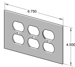
EC-9203 – Three gang outlet cover.
