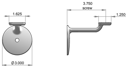
HB-4 – Handrail bracket complete w/lag cover. – Shown w/Lag-1.
