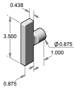
GK-9-1 – Contemporary gas key w/escutcheon.
