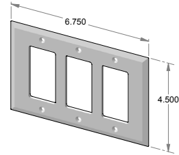
EC-303 – Three gang decora cover.
