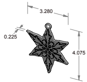
ORN-2011 – Snowflake ornament, 2011
