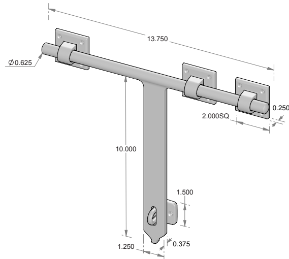
SLBT-14 – T-shaped slide bolt w/3guides.
