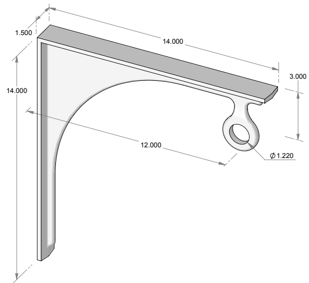
CLST-15BK – Closet bracket.
