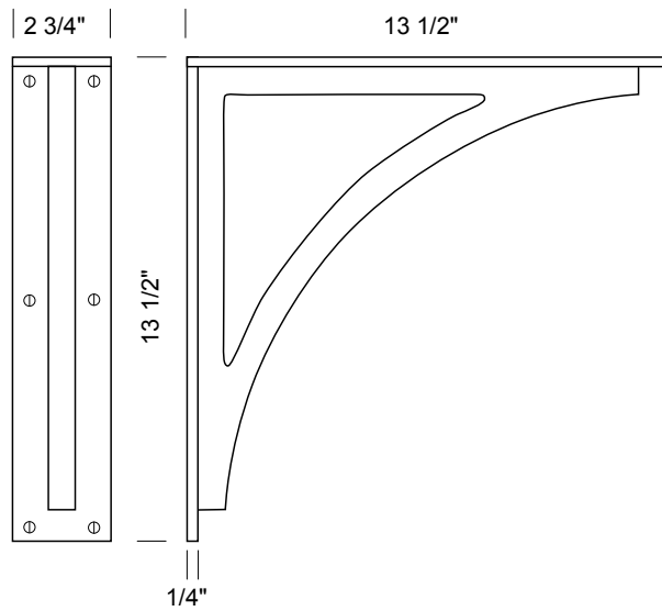
BKT-912 – Corner bracket
