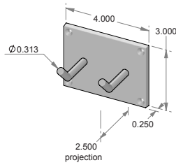
BDL-923 – Double prong hook.
