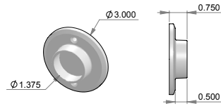
CLST-3WM – Closet rod wall mount pipe end.
