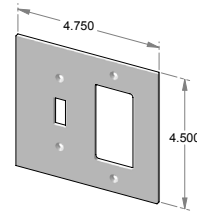
EC-9500 – Switchplate/decora combination cover.
