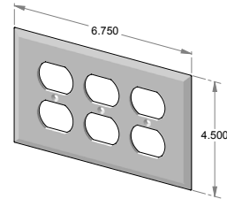
EC-203 – Three gang outlet cover.
