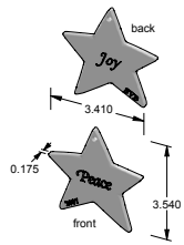
ORN-2007 – Star ornament, 2007
