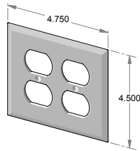
EC-202 – Two gang outlet cover.
