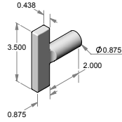
GK-9-2 – Contemporary gas key w/escutcheon.
