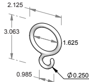
DRP-100 – Drapery bracket. – Shown w/RP-926. – Machined for 1.375" rod.
