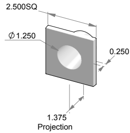
GK-9-ESC – Contemporary square gas key escutcheon.
