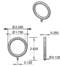
DRP-RING-2 – Drapery ring.
