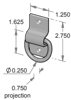
CT-100 – Two piece cross tie.
