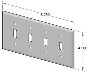
EC-104 – Four gang switchplate cover.
