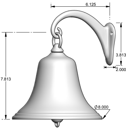
FPB-8 – 8" dia. solid bronze bell. – Available w/C-1 wall mount bracket.
