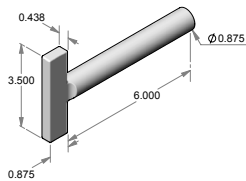
GK-9-6 – Contemporary gas key w/escutcheon.
