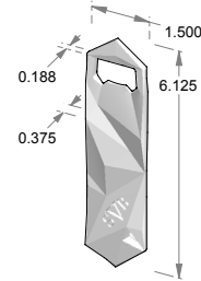
ORN-2023 – Hipster Bottle Opener ornament, 2023
