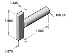
GK-9-4 – Contemporary gas key w/escutcheon.
