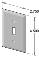
EC-101 – Single switchplate cover.
