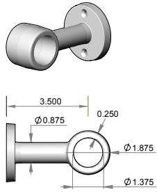
DRP-100 – Drapery bracket. – Shown w/RP-926. – Machined for 1.375" rod.
