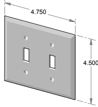
EC-102 – Two gang switchplate cover.
