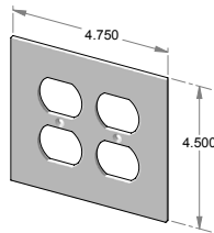
EC-9202 – Two gang outlet cover.
