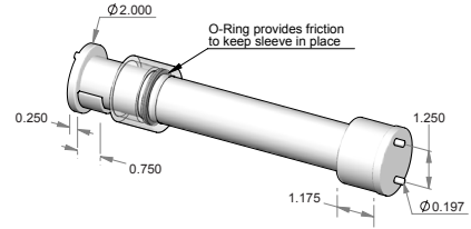
CLST-6PM – Peg mount closet end set w/sleeves.
