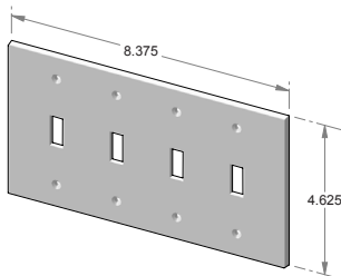
EC-9104 – Four gang switchplate cover.
