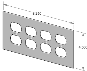
EC-9204 – Four gang outlet cover.
