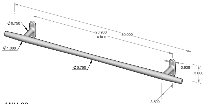
ANV-30 – Boat cleat.
