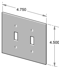
EC-9102 – Two gang switchplate cover.
