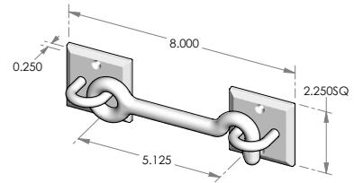
HE-100 – Large hook & eye. – 2.250" square plates.
