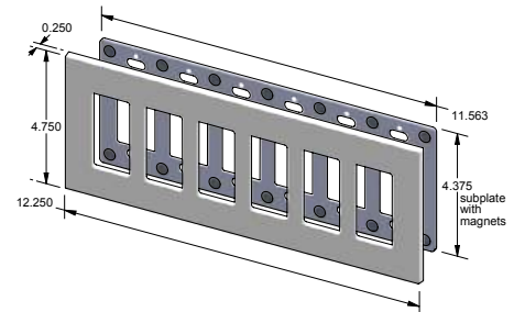
EC-9306M – Magnetic 6-gang decora cover.
