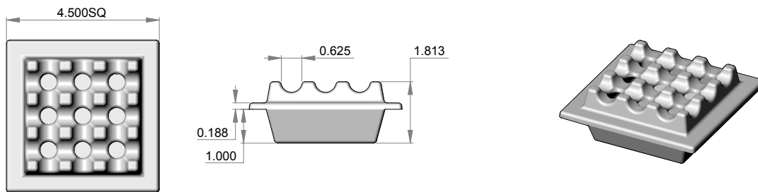
CIG-MC – Cigar tray.
