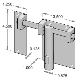
SLBT-6 – T-shaped slide bolt w/back plate & receiver. – Right hand shown. – Specify handing. – Available w/padlock hasp hole 0.4375 (specify).
