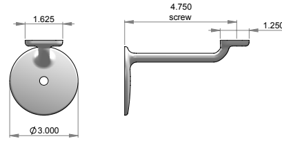
HB-2 – Handrail bracket complete w/lag cover. – Shown w/Lag-1.
