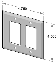
EC-302 – Two gang decora cover.
