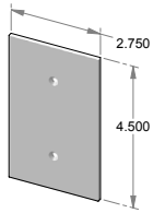
EC-9400 – Single blank cover.
