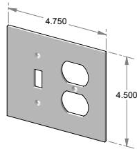
EC-9600 – Switchplate/outlet combination cover.
