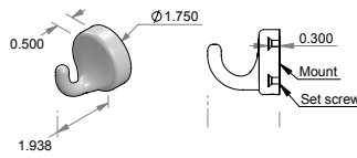
CLST-F2 – Closet rod finial w/hook.
