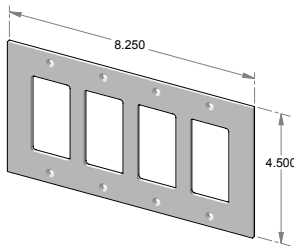
EC-9304 – Four gang decora cover.
