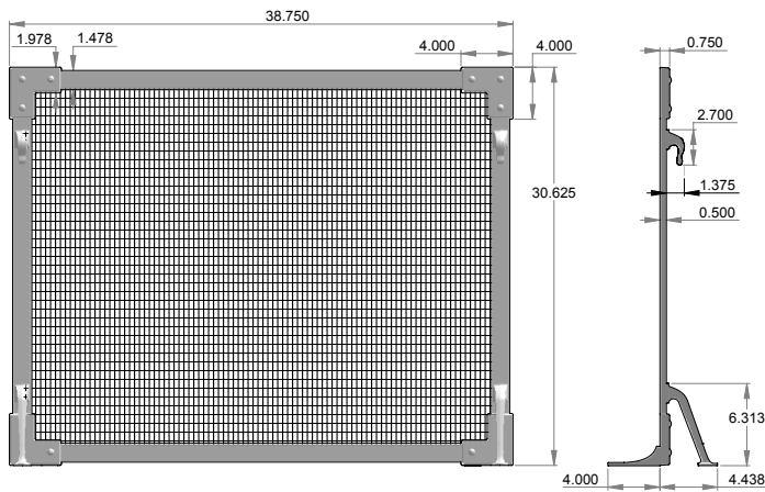
FS-100 – Fire screen.
