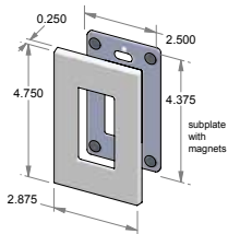
EC-9301M – Magnetic single decora cover.
