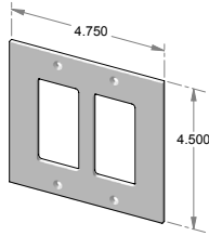
EC-9302 – Two gang decora cover.
