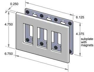
EC-9303M – Magnetic 3-gang decora cover.
