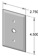
EC-401 – Cable cover.
