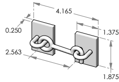
HE-50 – Small hook & eye. – 1.375" x 1.875" plates.
