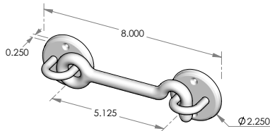
HE-200 – Large hook & eye. – 2.250" round plates.
