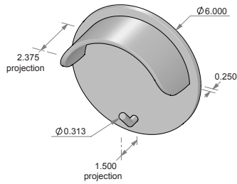
BDL-901 – Round bridle hook.
