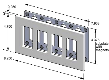
EC-9304M – Magnetic 4-gang decora cover.
