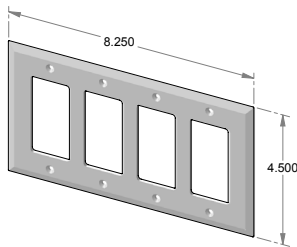
EC-304 – Four gang decora cover.
