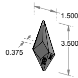
ORN-2017 – Hipster ornament, 2017
