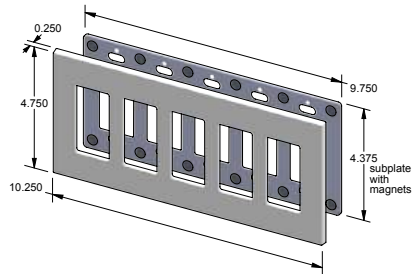
EC-9305M – Magnetic 5-gang decora cover.
