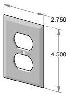
EC-201 – Single outlet cover.
