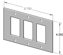
EC-9303 – Three gang decora cover.
