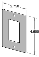
EC-9301 – Single decora cover.
