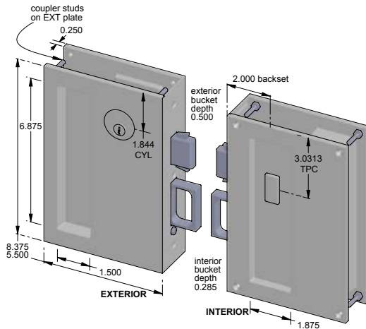
CS-SFP-58-2002ML-LH – Keyed set. – Left hand.
