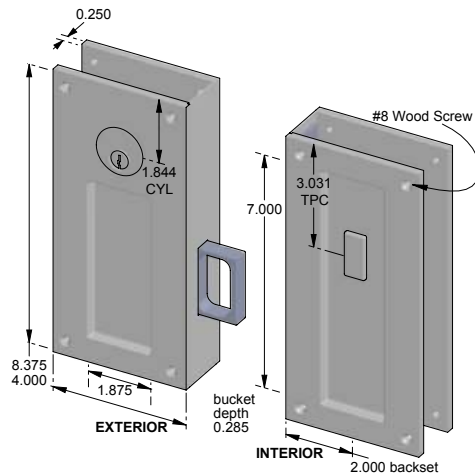
CS-SFP-48-2002ML-LH – Keyed set. – Left hand.
