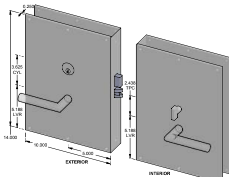
CS-N2500ML - Complete set with mortise lock, cylinder and spindle. - Single cylinder. - No key cover.
