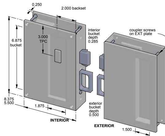
CS-SFP-58-2002ML-PF-RH – Patio function. – Right hand.
