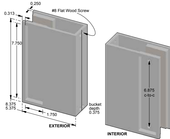
TS-SFP-58-138 – Saddle flush pull passage set. – Bucket depth 0.375”.
