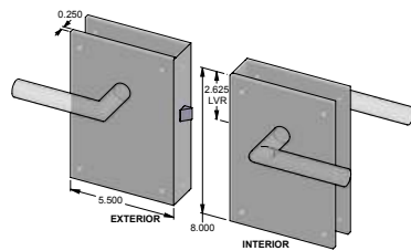
CS-F-N2085-8IML — Complete passage set w/interior mortise lock, 2.750" backset & spindle.
