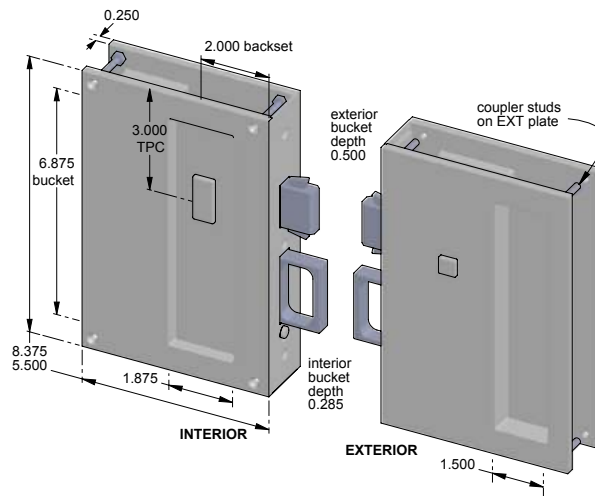
CS-SFP-58-2002IML-PR-RH – Complete privacy set. – Right hand.
