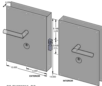
CS-FN2500ML-DC – Complete set with mortise lock, cylinder and spindle. – Double cylinder. – No key cover.
