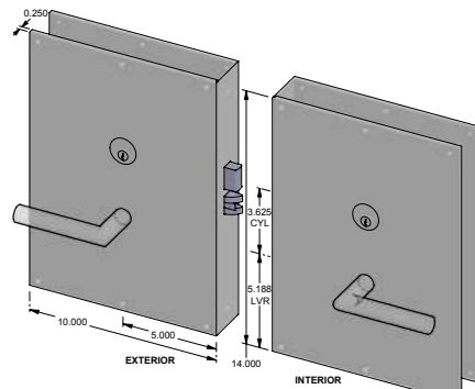
CS-N2500ML-DC - Complete set with mortise lock, cylinder and spindle. - Double cylinder. - No key cover.
