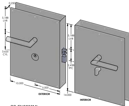
CS-FN2500ML – Complete set with mortise lock, cylinder and spindle. – Single cylinder. – No key cover.
