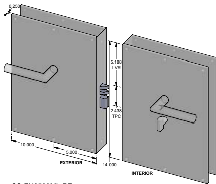
CS-FN2500ML-PF – Complete patio function set with mortise lock and spindle. – Patio function.
