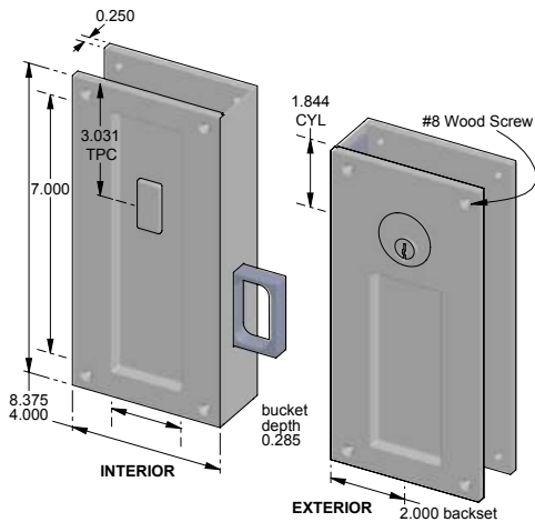
CS-SFP-48-2002ML-RH – Keyed set. – Right hand.
