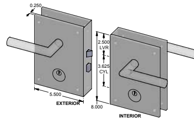
CS-FN2085.5ML-DC – Complete set with mortise lock, cylinder and spindle. – Double cylinder. – No key cover.
