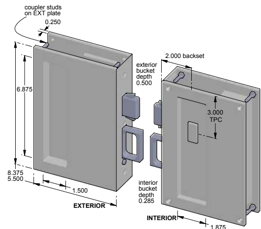
CS-SFP-58-2002ML-PF-LH – Patio function. – Left hand.
