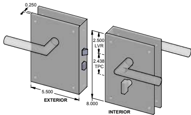
CS-FN2085.5ML-PF – Complete patio function set with mortise lock and spindle. – Patio function.
