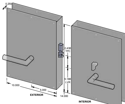
CS-N2500ML-PF - Complete patio function set with mortise lock and spindle. - Patio function.
