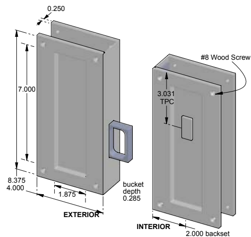
CS-SFP-48-2002ML-PF-LH – Patio function. – Left hand.
