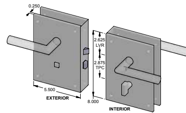
CS-F-N2085-8IML-PR — Complete privacy set w/interior mortise lock, 2.750" backset & spindle.
