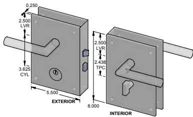
CS-FN2085.5ML – Complete set with mortise lock, cylinder and spindle. – Single cylinder. – No key cover.
