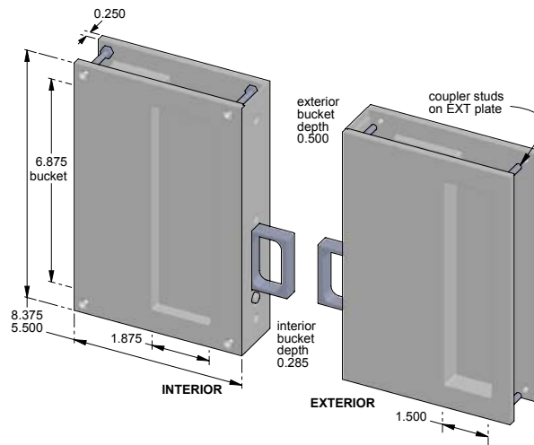
CS-SFP-58-2002IML-RH – Complete passage set. – Right hand.
