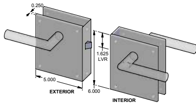
CS-F-N2065-8IML – Complete passage set w/interior mortise lock, 2.500" backset & spindle.
