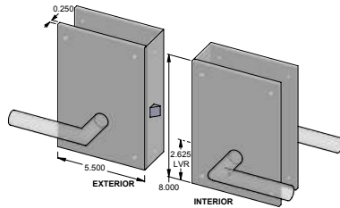
CS-N2085.5-8IML — Complete passage set w/interior mortise lock, 2.750" backset & spindle.
