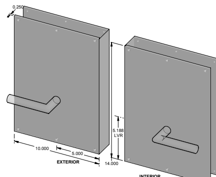
TS-N2500ML-FD - Trim set only. - Full dummy.
