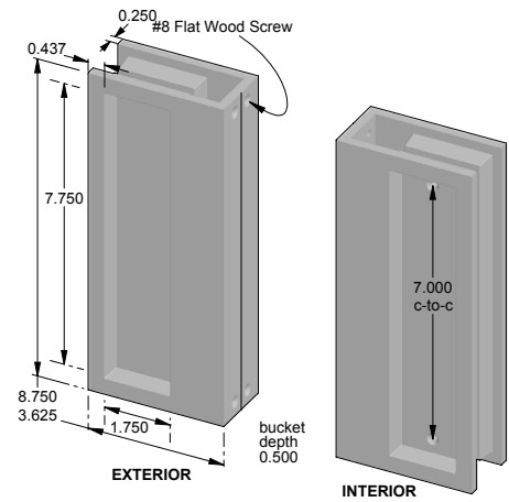
TS-SFP-38-134 – Saddle flush pull passage set.
