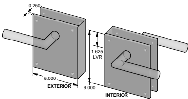
TS-F-N2065IML-FD – Full dummy. – Trim set only.
