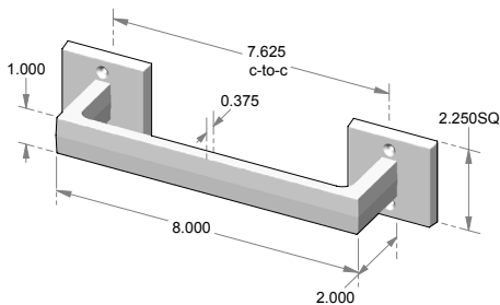
STB-983 – 8.000" Solid towel bar. – Shown w/P-N925
