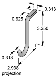
CH-14UM – J-coat hook w/undermount return. – Top of return is flat.
