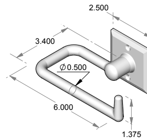
AW-100RH – Toilet paper holder. – Shown w/P-402. – Points right.
