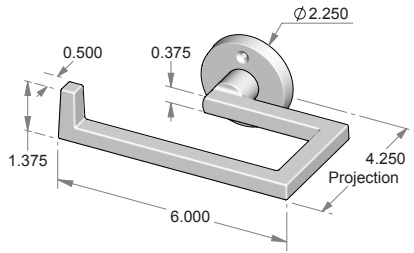
AW-9100LH – Toilet paper holder. – Shown w/RP-925. – Points left.
