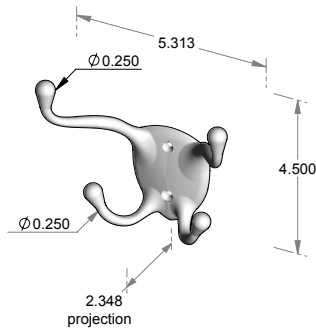
CH-4 – Four prong coat hook.
