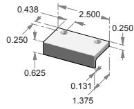
CK-500 – Edge mount cabinet pull.
