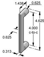
CK-1104 – Contemporary cabinet pull w/round feet. – 4.000" center-to-center. – 0.3125" face width.
