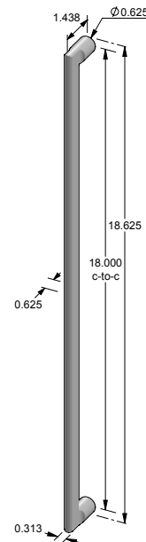
CK-1118 – Contemporary cabinet pull w/round feet. – 18.000" center-to-center. – 0.3125" face width.
