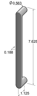
CK-912 – Contemporary cabinet pull. – 6.937" center-to-center.
