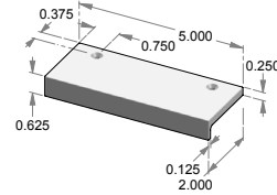
CK-498-5 – Edge mount cabinet pull.
