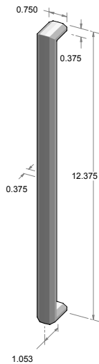
CK-9413 – Contemporary cabinet pull. – 12.000" center-to-center.
