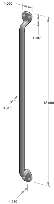
SP-18 – Surface mount sash pull. – 17.250" center-to-center. – 0.500" face width.
