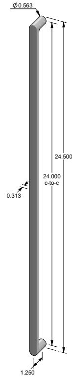
CK-912-24 – Contemporary cabinet pull. – 24.000" center-to-center.
