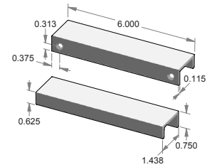
CK-502-6 – Edge mount cabinet pull.
