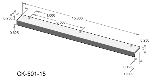
CK-501-15 – Edge mount cabinet pull.
