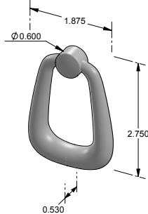
CK-523 – Cabinet ring pull.
