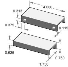
CK-505-4 – Edge mount cabinet pull.
