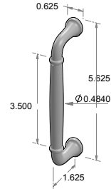
CK-144 – Ridge cabinet pull. – 4.875" center-to-center. – 0.562" round.
