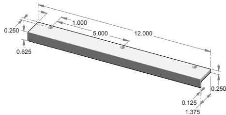
CK-501-12 – Edge mount cabinet pull.
