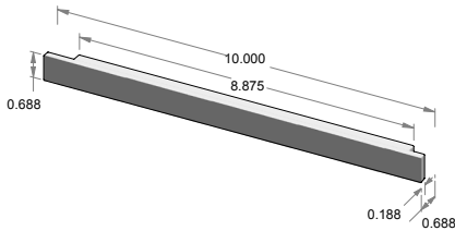
CK-1910 – Cabinet pull. – 8.000" center-to-center.
