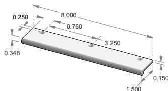
CK-499R-8 – Rolled edge mount cabinet pull.
