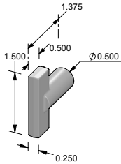
CK-9101 – Contemporary cabinet knob.
