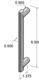
CK-9106 – Contemporary cabinet pull w/round feet. – 5.000" center-to-center. – 0.250" face width.
