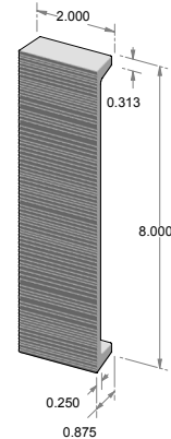
CK-9208CDRY – Corduroy cabinet pull. – 7.687" center-to-center.
