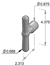
CK-229T – T-handle cabinet knob.
