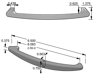
CK-860 – Swept cabinet pull. – 8.063" center-to-center.
