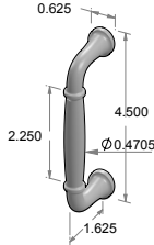
CK-143 – Ridge cabinet pull. – 3.750" center-to-center. – 0.500" round.
