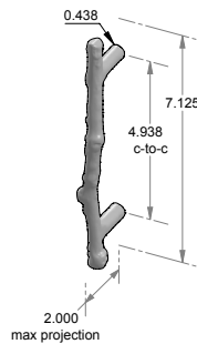
CK-721 – Twig cabinet pull – 4.938" center-to-center. – 0.438" round.
