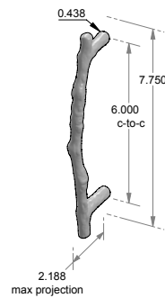
CK-722 – Twig cabinet pull – 6.000" center-to-center. – 0.438" round.
