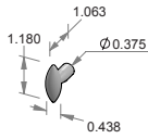
CK-460 – Contemporary Aero cabinet knob.
