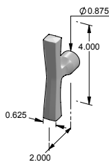
CK-228T – T-handle cabinet knob.
