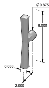
CK-228T-6 – T-handle cabinet knob.
