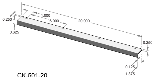
CK-501-20 – Edge mount cabinet pull.
