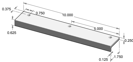
CK-497-10 – Edge mount cabinet pull.
