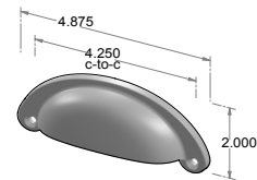
CK-508 – Surface mount bin pull. – 4.250" center-to-center.
