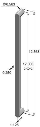
CK-913 – Contemporary cabinet pull. – 12.000" center-to-center.
