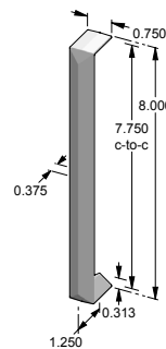
CK-9608 – Contemporary cabinet pull. – 7.750" center-to-center. – Top & underside of pull are V-shaped.
