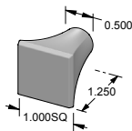
CK-233 – Pawn base cabinet knob.
