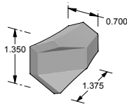
CK-235 – King cabinet knob.
