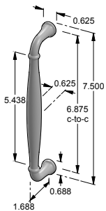
CK-145 – Ridge cabinet pull. – 6.875" center-to-center. – 0.625" round.
