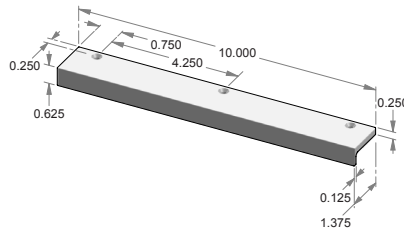
CK-501-10 – Edge mount cabinet pull.
