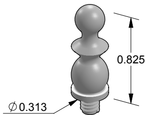
BHCf-FREN French cabinet finial.
