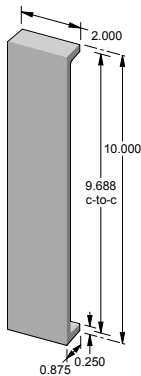
CK-9210 – Contemporary cabinet pull. – 9.688" center-to-center.
