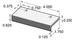
CK-497-4 – Edge mount cabinet pull.
