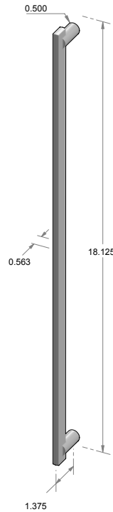
CK-9118 – Contemporary cabinet pull w/round feet. – 17.125" center-to-center. – 0.250" face width.
