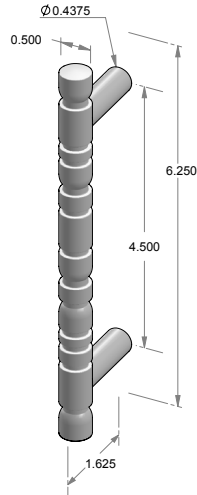
CK-195-6 – Assemblage cabinet pull – 4.500" center-to-center. – 0.500" round.
