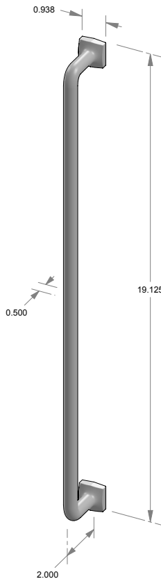
CK-587 – Square foot cabinet pull. – 18.125" center-to-center. – 0.500" round.
