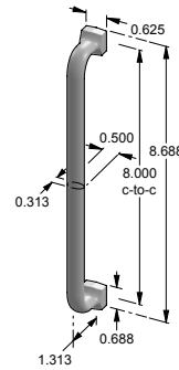
CK-514-8 – Square foot cabinet pull. – 8.000" center-to-center. – 0.500" face width.
