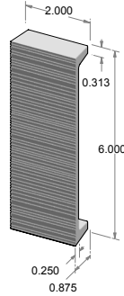
CK-9206CDRY – Corduroy cabinet pull. – 5.687" center-to-center.
