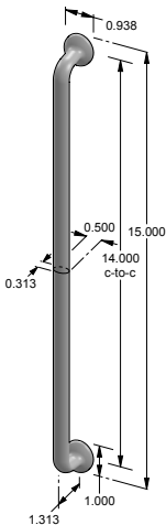
CK-510-14 – Organic round foot cabinet pull. – 14.000" center-to-center. – 0.500" face width.
