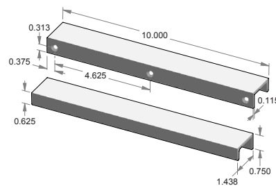
CK-502-10 – Edge mount cabinet pull.
