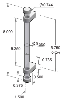
CK-ACR-DWL-CAP-8 – Acrylic cabinet pull w/caps. – 5.750" center-to-center. – Dowel available in acrylic, white oak or white oak w/black stain.
