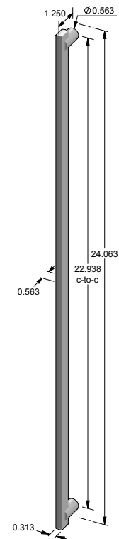
CK-9124 – Contemporary cabinet pull w/round feet. – 22.938" center-to-center. – 0.312" face width.
