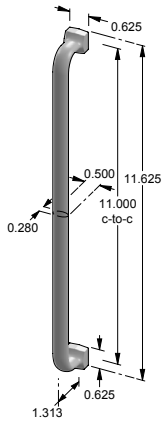
CK-514-11 – Square foot cabinet pull. – 11.000" center-to-center. – 0.500" face width.
