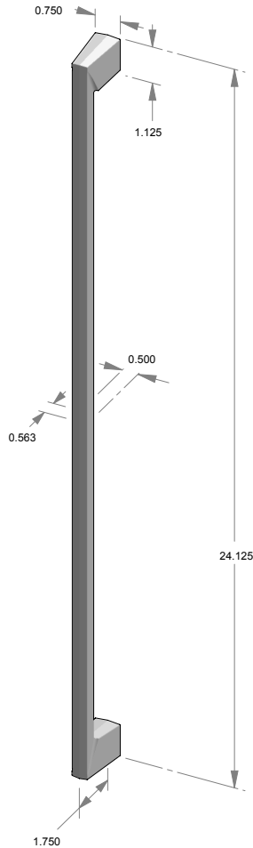
CK-805-24 – Swedge cabinet pull. – 23.000" center-to-center. – 0.500" face width.
