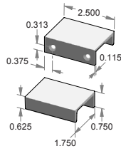
CK-505-25 – Edge mount cabinet pull.
