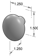
CK-303 – Oval cabinet knob.
