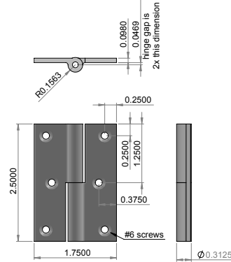
BHC-25175 – 2.5000" x 1.7500" cabinet hinge. – Shown w/flat finial. – Leaf thickness 0.0980". – Hinge gap when closed 0.0938".
