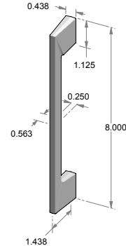
CK-805 – Swedge cabinet pull. – 6.875" center-to-center. – 0.250" face width.
