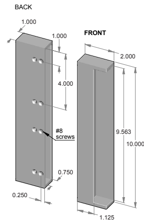
FEP-110-CAP – Flush cabinet pull w/cap. – Flush mount at top edge of cabinet door.
