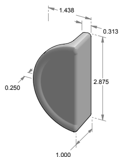
CK-HRB150 – Half-round banded cabinet pull. – 2.000" center-to-center.
