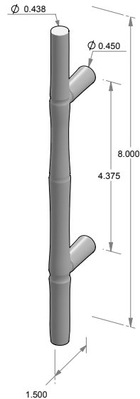
CK-1307 – Bamboo cabinet pull – 4.375" center-to-center. – 0.438" round.
