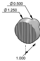
CK-420 – Corduroy round flat cabinet knob.
