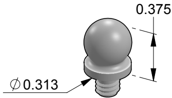
BHCf-BALL Ball cabinet finial.
