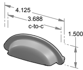
CK-506 – Blind mount bin pull without screw holes. – 3.688" center-to-center.
