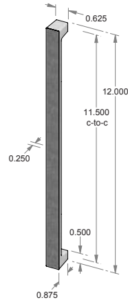
CK-2250-12 – Burlap cabinet pull. – 11.500" center-to-center.
