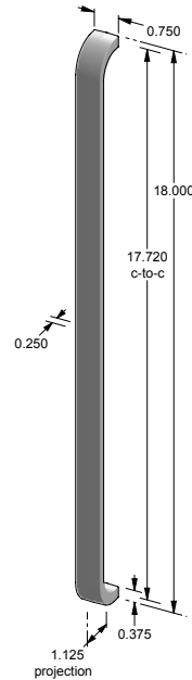
CK-9718 – Contemporary cabinet pull. – 17.720" center-to-center. – 0.750" face width.
