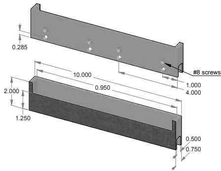
FEP-B210 – Flush cabinet pull.
