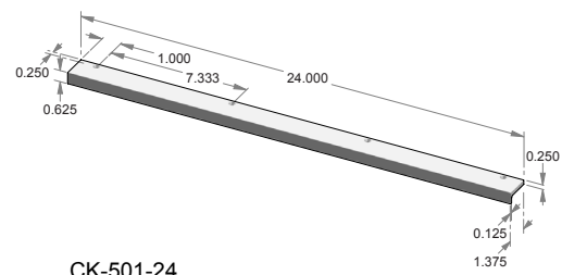
CK-501-24 – Edge mount cabinet pull.
