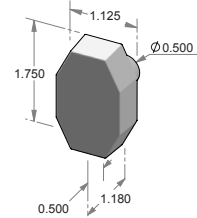
CK-419 – Contemporary octagonal cabinet knob.
