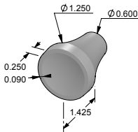
CK-GOLFTEE-2 – Golf Tee cabinet knob.
