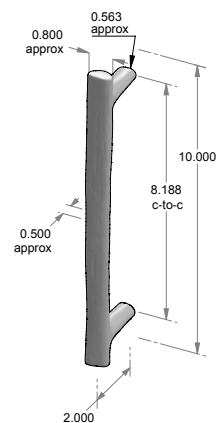
CK-729 – Cactus cabinet pull. – 8.188" center-to-center. – 0.800" face width.
