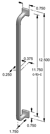
CK-535-12 – Square handle cabinet pull. – 11.750" center-to-center. – 0.375" face width.
