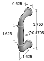
CK-142 – Ridge cabinet pull. – 3.000" center-to-center. – 0.500" round.
