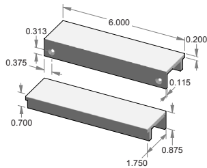
CK-503T-6 – Edge mount cabinet pull.
