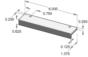
CK-501-6 – Edge mount cabinet pull.
