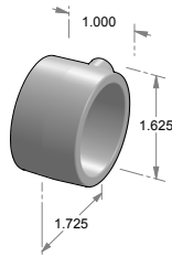
CK-CR158 – Hoop cabinet pull.
