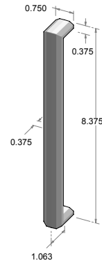
CK-9409 – Contemporary cabinet pull. – 8.000" center-to-center.
