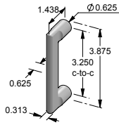
CK-1103.25 – Contemporary cabinet pull w/round feet. – 3.250" center-to-center. – 0.3125" face width.
