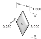
CKE-300DI-SOFT – Diamond w/soft bevel cabinet knob escutcheon. – 0.188" Thick.
