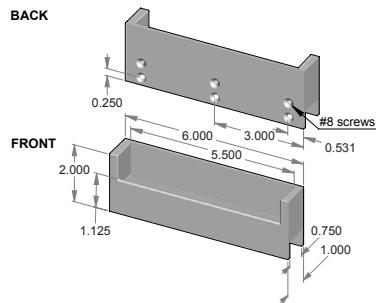
FEP-110-6 – Flush cabinet pull.
