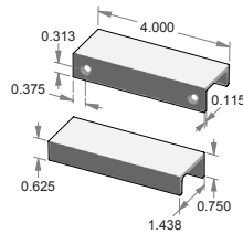
CK-502-4 – Edge mount cabinet pull.
