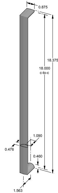
CK-969-18 – Ergonomic cabinet pull. – 18.000" center-to-center. – Underside 0.476" round.
