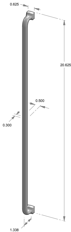
CK-514-20 – Square foot cabinet pull. – 20.000" center-to-center. – 0.500" face width.
