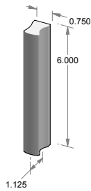
CK-980-6 – Contemporary cabinet pull. – 4.500" center-to-center.
