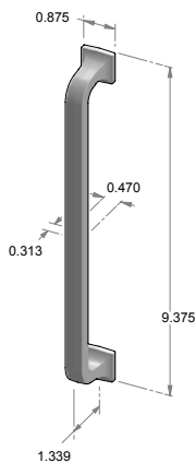
CK-548 – Square handle cabinet pull. – 8.500" center-to-center. – 0.437" face width.
