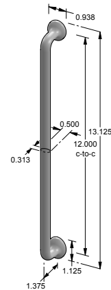
CK-510-12 – Organic round foot cabinet pull. – 12.000" center-to-center. – 0.500" face width.
