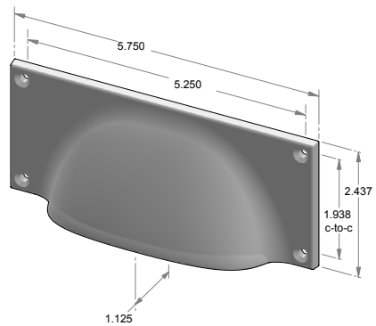
CK-606 – Surface mount bin pull. – 5.250" center-to-center.
