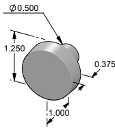
CK-417 – Contemporary round flat cabinet knob.
