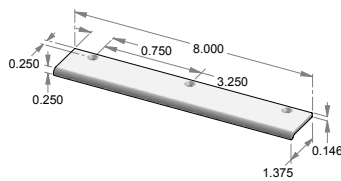
CK-501R-8 – Rolled edge mount cabinet pull.
