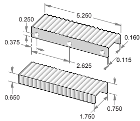
CK-1605-RETURN – Scalloped edge mount cabinet pull w/return.
