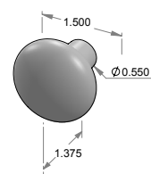
CK-405 – Mushroom cabinet knob.
