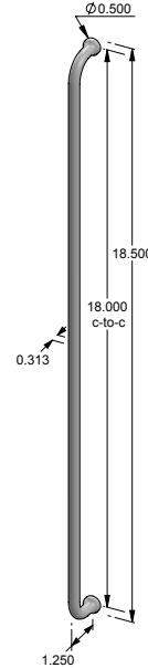
CK-569-18 – 18.500" Cabinet pull. – 18.000" center-to-center. – 0.313" round.
