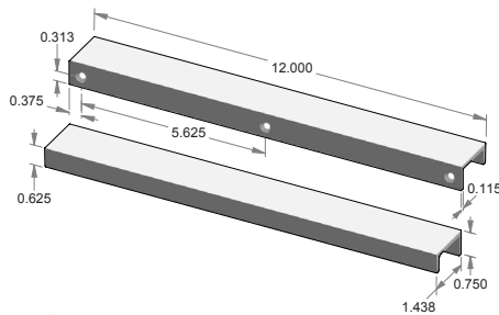
CK-502-12 – Edge mount cabinet pull.
