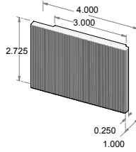
CK-1904CDRY – Corduroy cabinet pull. – 1.500" center-to-center.
