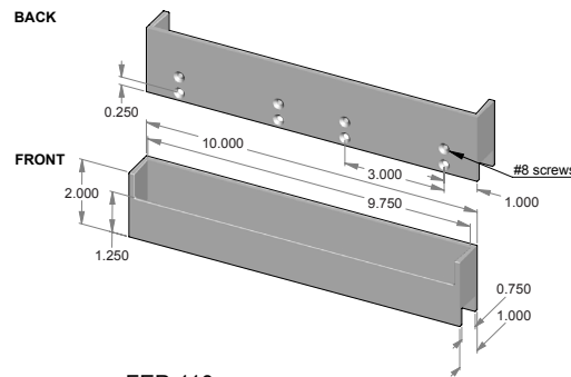
FEP-110 – Flush cabinet pull.
