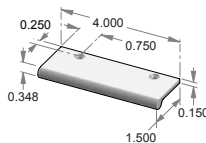
CK-499R-4 – Rolled edge mount cabinet pull.
