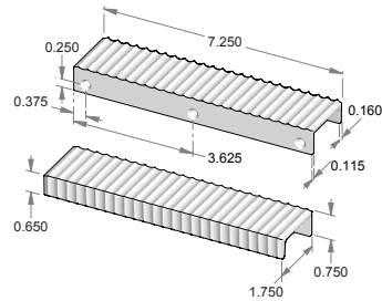
CK-1607-RETURN – Scalloped edge mount cabinet pull w/return.
