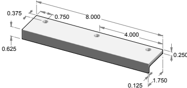
CK-497-8 – Edge mount cabinet pull.
