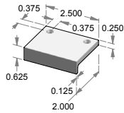
CK-498-2.5 – Edge mount cabinet pull.
