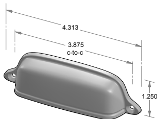
CK-603 – Ridge surface mount bin pull. – 3.875" center-to-center.
