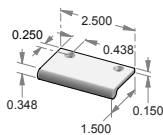
CK-499R-2.5 – Rolled edge mount cabinet pull.
