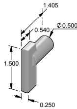
CK-9102 – Contemporary cabinet knob.
