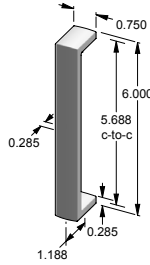
CK-951 – Contemporary cabinet pull. – 5.688" center-to-center.
