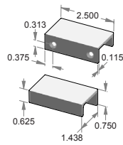
CK-502 – Edge mount cabinet pull.
