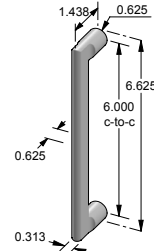
CK-1106 – Contemporary cabinet pull w/round feet. – 6.000" center-to-center. – 0.3125" face width.
