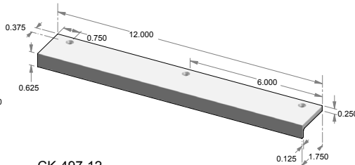
CK-497-12 – Edge mount cabinet pull.
