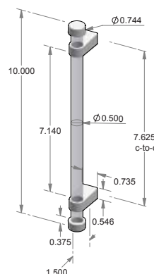
CK-ACR-DWL-CAP-10 – Acrylic cabinet pull w/caps. – 7.625" center-to-center. – Dowel available in acrylic, white oak or white oak w/black stain.
