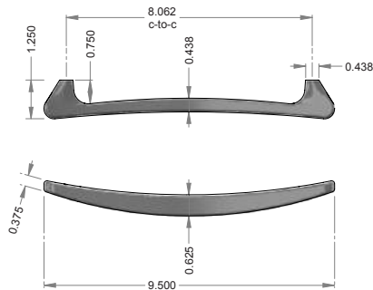
CK-850 – Swept cabinet pull. – 8.062" center-to-center.
