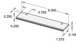
CK-501R-6 – Rolled edge mount cabinet pull.
