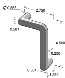
CK-998LH – L-shaped cabinet pull.
