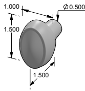
CK-306 – Ridge oval cabinet knob.
