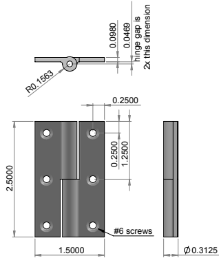
BHC-25150 – 2.5000" x 1.5000" cabinet hinge. – Shown w/flat finial. – Leaf thickness 0.0980". – Hinge gap when closed 0.0938".
