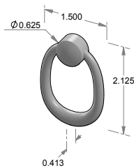
CK-519 – Cabinet ring pull.
