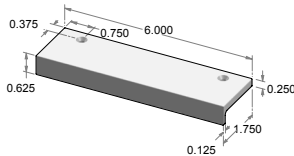
CK-497-6 – Edge mount cabinet pull.
