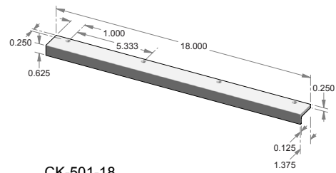
CK-501-18 – Edge mount cabinet pull.
