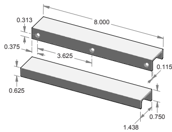
CK-502-8 – Edge mount cabinet pull.
