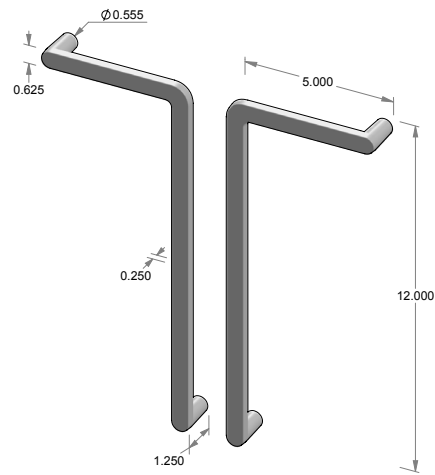
CK-998-512LH & CK-998-512RH – L-shaped cabinet pull.
