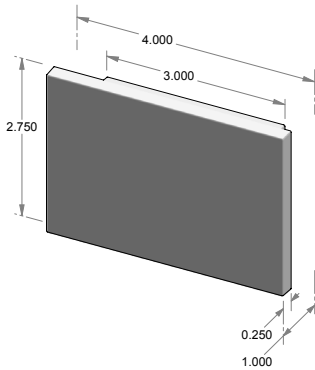
CK-1904 – Cabinet pull. – 1.500" center-to-center.
