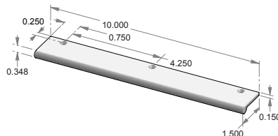
CK-499R-10 – Rolled edge mount cabinet pull.
