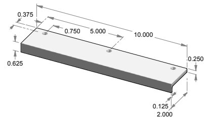
CK-498-10 – Edge mount cabinet pull.
