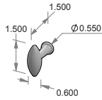
CK-461 – Contemporary Medium Aero cabinet knob.
