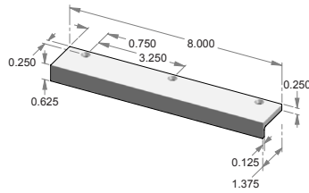
CK-501-8 – Edge mount cabinet pull.
