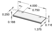
CK-501R – Rolled edge mount cabinet pull.
