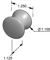
CK-451 – Flared cabinet knob.
