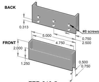
FEP-210-5 – Flush cabinet pull.
