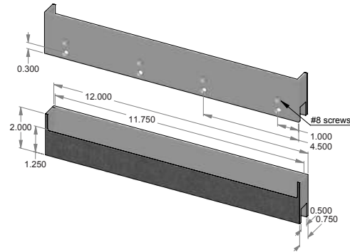
FEP-B212 – Flush cabinet pull.
