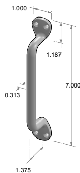
SP-700 – Surface mount sash pull. – 6.125" center-to-center. – 0.500" face width.
