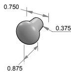
CK-400 – Mushroom knob.
