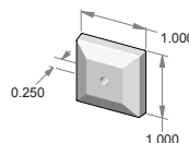
CKE-1 – Bevel Edge cabinet knob escutcheon. – 0.250" Thick.
