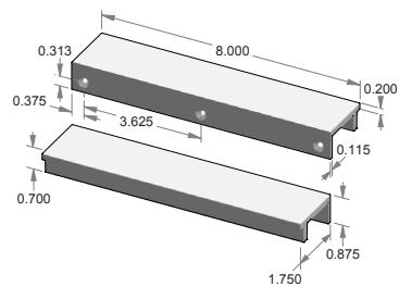
CK-503T-8 – Edge mount cabinet pull.
