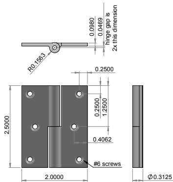
BHC-25200 – 2.5000" x 2.0000" cabinet hinge. – Shown w/flat finial. – Leaf thickness 0.0980". – Hinge gap when closed 0.0938".
