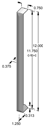
CK-9612 – Contemporary cabinet pull. – 11.750" center-to-center. – Top & underside of pull are V-shaped.
