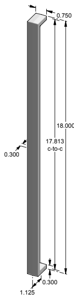
CK-955 – Contemporary cabinet pull. – 17.813" center-to-center.
