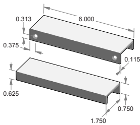
CK-505-6 – Edge mount cabinet pull.
