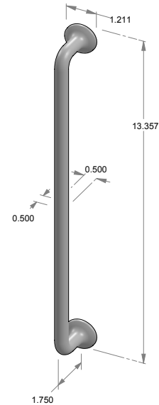
CK-578 – Round foot cabinet pull. – 12.125" center-to-center. – 0.500" round.
