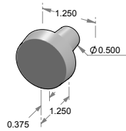
CK-417LS – Contemporary round flat cabinet knob.
