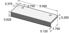
CK-497-5 – Edge mount cabinet pull.
