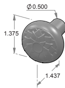
CK-230 – Artichoke round cabinet knob.
