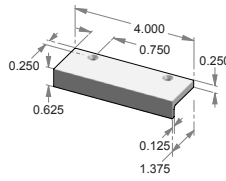
CK-501 – Edge mount cabinet pull.
