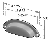
CK-507 – Surface mount bin pull. – 3.688" center-to-center.
