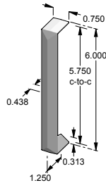
CK-9606 – Contemporary cabinet pull. – 5.750" center-to-center. – Top & underside of pull are V-shaped.
