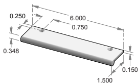
CK-499R-6 – Rolled edge mount cabinet pull.
