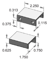
CK-505-225 – Edge mount cabinet pull.
