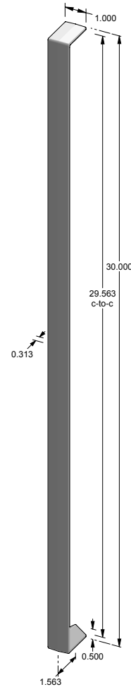
CK-9530 – Contemporary cabinet pull. – 29.563" center-to-center. – Underside of pull is V-shaped.
