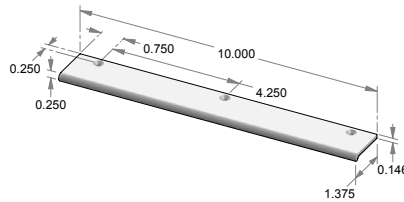
CK-501R-10 – Rolled edge mount cabinet pull.
