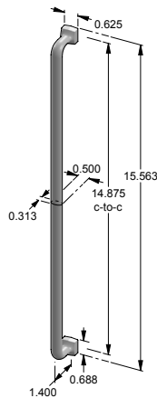
CK-514-15 – Square foot cabinet pull. – 14.875" center-to-center. – 0.500" face width.
