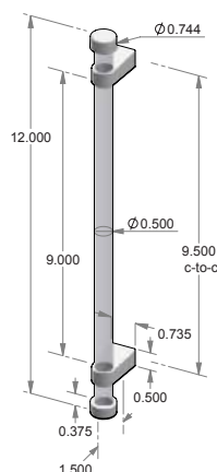
CK-ACR-DWL-CAP-12 – Acrylic cabinet pull w/caps. – 9.500" center-to-center. – Dowel available in acrylic, white oak or white oak w/black stain.
