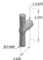
CK-230T – T-handle cabinet knob.
