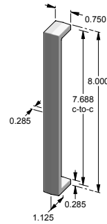
CK-952 – Contemporary cabinet pull. – 7.688" center-to-center.
