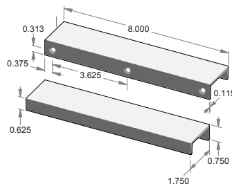
CK-505-8 – Edge mount cabinet pull.
