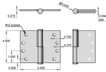
BH-4050 – 4.000" x 5.000" wide throw hinge. – Shown w/flat finial. – Leaf thickness 0.210". – Hinge gap when closed 0.0940".
