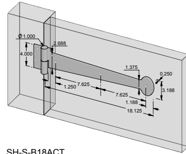
SH-S-B18ACT – 18.125" Active Bean mortise mount strap hinge. – Shown w/button finial. – 2.688" Heel. – Right hand shown.
