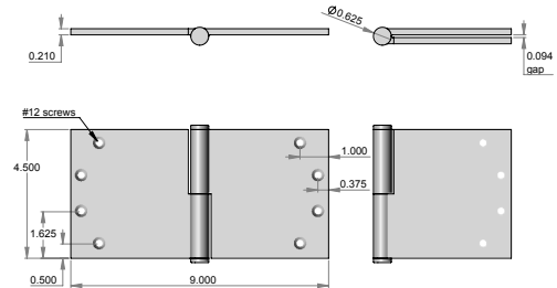
BH-4590 – 4.500" x 9.000" wide throw hinge. – Shown w/flat finial. – Leaf thickness 0.210". – Hinge gap when closed 0.0940".
