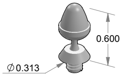
BHCf-ACRN Acorn cabinet finial.
