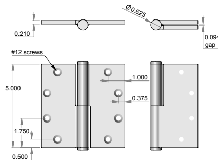
BH-5050 – 5.000" x 5.000" hinge. – Shown w/flat finial. – Leaf thickness 0.210". – Hinge gap when closed 0.0940".
