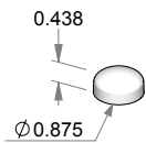
LAG-1 – 0.875" x 0.438" Dome.
