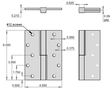
BH-SQ6045 – 6.000" x 4.500" square knuckle hinge. – No finial. – Leaf thickness 0.210". – Hinge gap when closed 0.0940".
