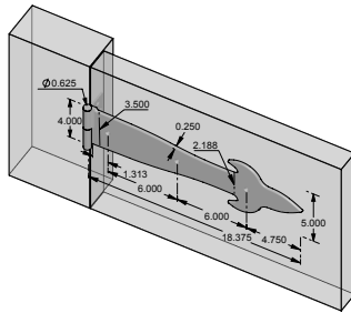
SH-M-FDL18-ACT – 18.000" Active Fleur de Lis mortise mount strap hinge. – Shown w/flat finial. – 3.500" heel. – Right hand shown.
