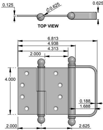
BH-4040BFP – Bi-fold door hinge. – Shown w/ball finial.
