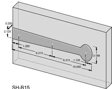
SH-B15 – 15.000" Dummy Bean strap hinge.
