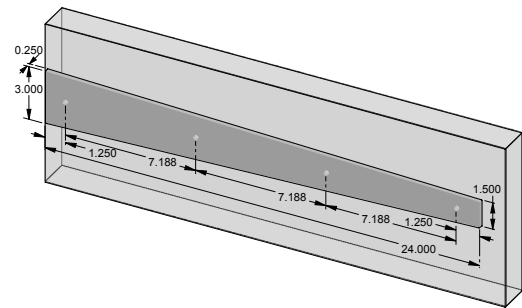
SH-SQ24 – 24.000" Dummy Square strap hinge.
