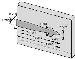
SH-FDL-S12 – 12.000" Dummy Small Fleur de Lis strap hinge.
