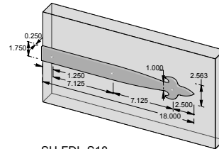
SH-FDL-S18 – 18.000" Dummy Small Fleur de Lis strap hinge.
