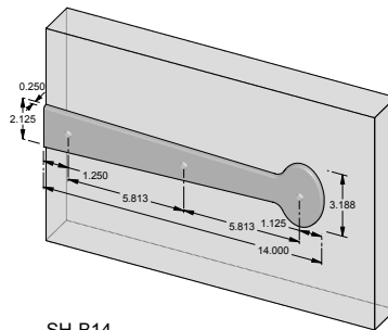
SH-B14 – 14.000" Dummy Bean strap hinge.
