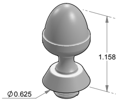
BHF-ACRN Acorn finial.
