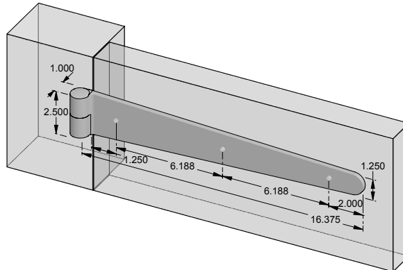
SH-160ACT – 16.500" Active strap hinge. – Right hand shown.
