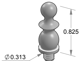
BHCf-FREN French cabinet finial.
