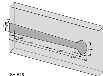
SH-B18 – 18.000" Dummy Bean strap hinge.
