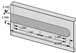
SH-RT18 – 18.000" Dummy strap hinge.
