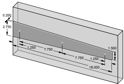
SH-SQ18 – 18.000" Dummy Square strap hinge.
