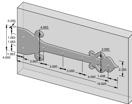
SH-G16 – 15.625" Dummy decorative strap hinge.
