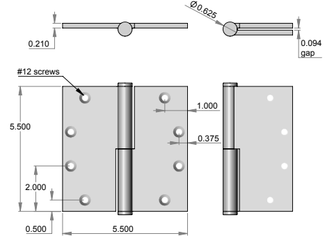
BH-5555 – 5.500" x 5.500" hinge. – Shown w/flat finial. – Leaf thickness 0.210". – Hinge gap when closed 0.0940".
