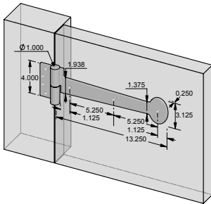
SH-S-B13ACT – 13.250" Active Bean mortise mount strap hinge. – Shown w/button finial. – 1.313" Heel. – Right hand shown.
