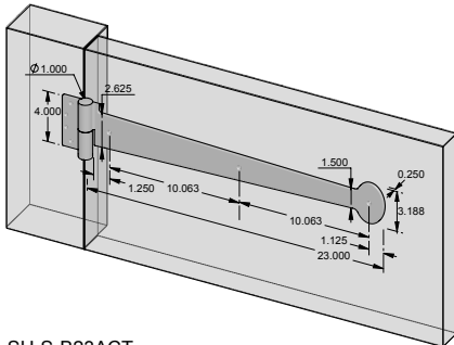
SH-S-B23ACT – 23.000" Active Bean mortise mount strap hinge. – Shown w/button finial. – 2.625" Heel. – Right hand shown.
