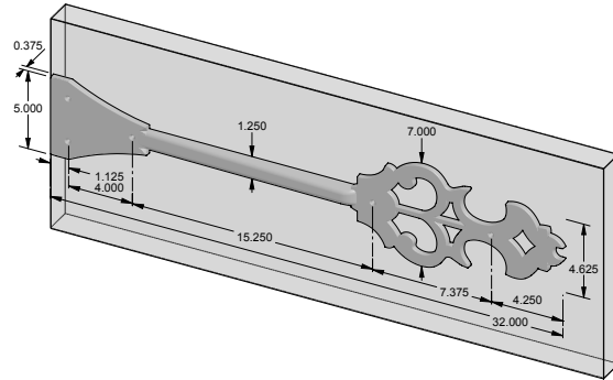
SH-OD32 – 32.000" Dummy Ornate strap hinge. – Left shown.
