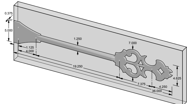
SH-OD36 – 36.000" Dummy Ornate strap hinge. – Left shown.
