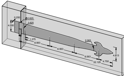
SH-S-FDL32-ACT - 32.125" Active Fleur de Lis surface mount strap hinge. - Shown w/flat finial. - 3.625" heel. - Right hand shown.
