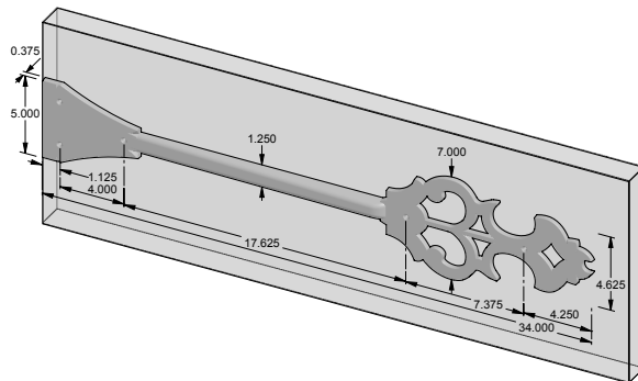
SH-OD34 – 34.000" Dummy Ornate strap hinge. – Left shown.
