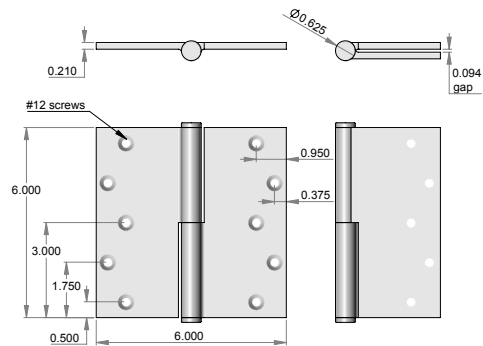
BH-6060 – 6.000" x 6.000" hinge. – Shown w/flat finial. – Leaf thickness 0.210". – Hinge gap when closed 0.0940".
