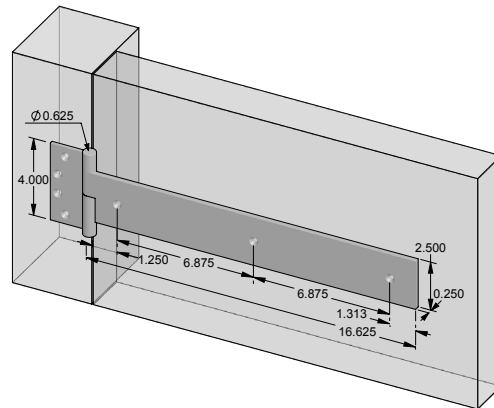
SH-S-F16ACT – 16.625" Active Square surface mount strap hinge. – Shown w/flat finial. – Right hand shown.
