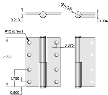
BH-5035 – 5.000" x 3.500" hinge. – Shown w/flat finial. – Leaf thickness 0.210". – Hinge gap when closed 0.0940".
