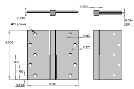
BH-SQ6060 – 6.000" x 6.000" square knuckle hinge. – No finial. – Leaf thickness 0.210". – Hinge gap when closed 0.0940".
