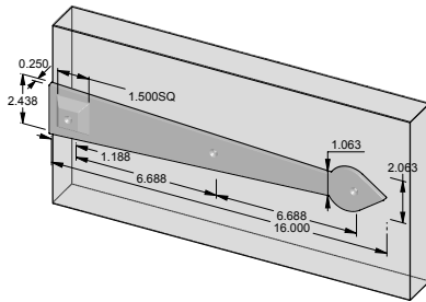
SH-D16 – 16.000" Dummy Spade strap hinge.
