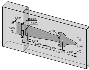
SH-S-FDL18-ACT - 18.000" Active Fleur de Lis surface mount strap hinge. - Shown w/flat finial. - 3.500" heel. - Right hand shown.
