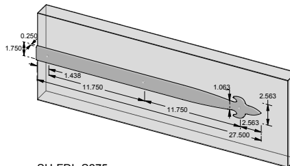
SH-FDL-S275 – 27.500" Dummy Small Fleur de Lis strap hinge.
