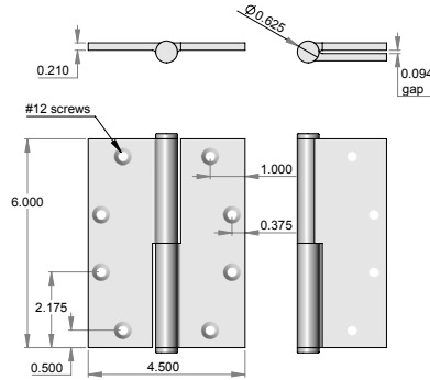
BH-6045 – 6.000" x 4.500" hinge. – Shown w/flat finial. – Leaf thickness 0.210". – Hinge gap when closed 0.0940".
