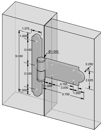
SH-S-ARCH6-ACT – 6.375" Active Arch surface mount strap hinge. – Provided w/button finial. – Right hand shown.
