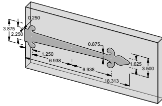
SH-FDL2-18 – 18.3125" Dummy Fleur de Lis strap hinge. – Provided w/#8 x 1 1/4" oval wood screws.
