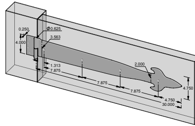
SH-S-FDL30-ACT - 30.000" Active Fleur de Lis surface mount strap hinge. - Shown w/flat finial. - 3.563" heel. - Right hand shown.
