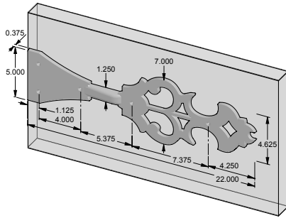
SH-OD22 – 22.000" Dummy Ornate strap hinge. – Left shown.
