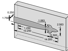
SH-FDL-S14 – 14.000" Dummy Small Fleur de Lis strap hinge.
