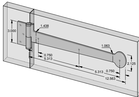
SH-B-12-ACT-CK – 12.563" Active cabinet strap hinge. – 1.438" Heel. – Left shown.
