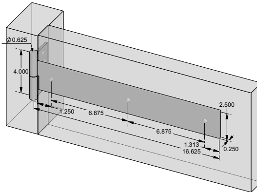
SH-M-F16ACT – 16.625" Active Square mortise mount strap hinge. – Shown w/flat finial. – Right hand shown.
