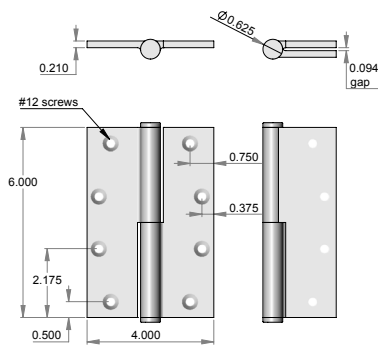
BH-6040 – 6.000" x 4.000" hinge. – Shown w/flat finial. – Leaf thickness 0.210". – Hinge gap when closed 0.0940".
