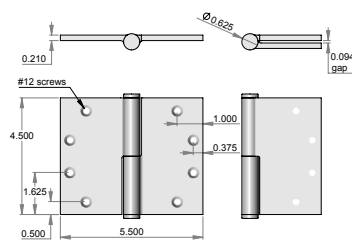
BH-4555 – 4.500" x 5.500" wide throw hinge. – Shown w/flat finial. – Leaf thickness 0.210". – Hinge gap when closed 0.0940".
