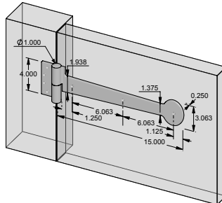
SH-S-B15ACT – 15.000" Active Bean mortise mount strap hinge. – Shown w/button finial. – 2.000" Heel. – Right hand shown.
