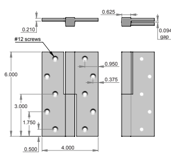
BH-SQ6040 – 6.000" x 4.000" square knuckle hinge. – No finial. – Leaf thickness 0.210". – Hinge gap when closed 0.0940".
