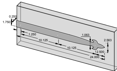
SH-FDL-S24 – 24.000" Dummy Small Fleur de Lis strap hinge.
