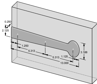
SH-B13 – 13.000" Dummy Bean strap hinge.
