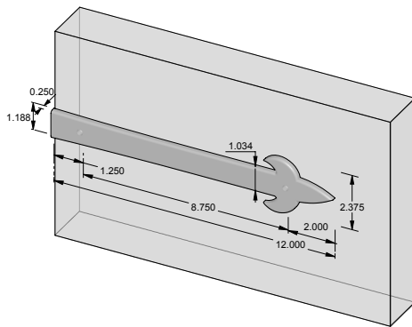
SH-FDL-N12 – 12.000" Dummy Narrow Fleur de Lis strap hinge.
