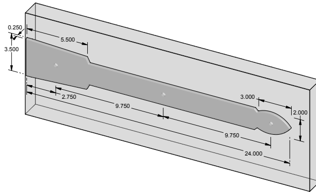
SH-ARW-24 – 24.000" Dummy Arrow strap hinge.
