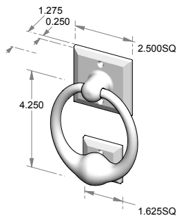
DKS-4 – Door knocker w/strike plate.
