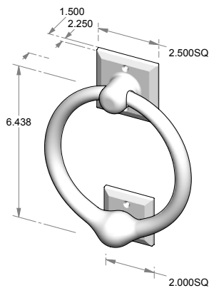
DKS-6 – Door knocker w/strike plate.
