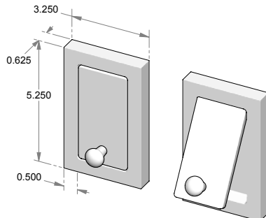
DK-J2 – Surface mount door knocker w/attached strike plate.
