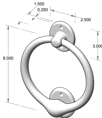
DK-8 – Door knocker w/strike plate.
