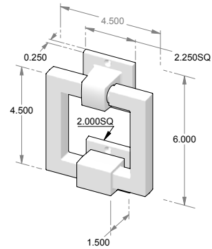
DK-94 – Square door knocker w/strike plate.
