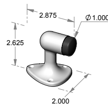
DS-2 – Floor mount door stop. – Includes mounting hardware for wood & masonry floors.
