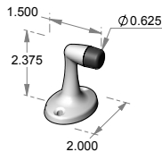
DS-7 – Floor mount door stop. – Includes mounting hardware for wood & masonry floors.
