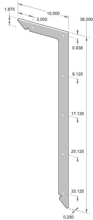
SH-C-36 – Decorative corner bracket. – Right hand shown.
