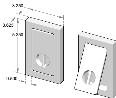
DK-J1 – Surface mount door knocker w/attached strike plate.
