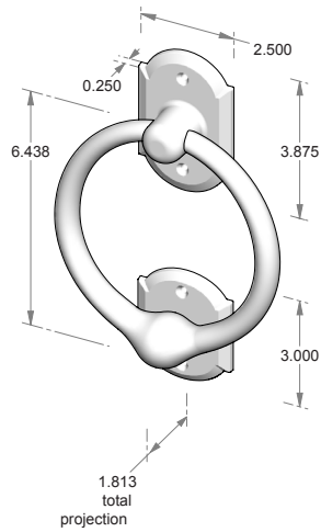
DKA-6 – Door knocker w/strike plate.
