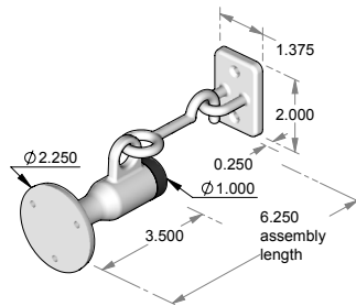
DS-5HE – Base/wall mount door stop w/hook & eye. – Includes wood mounting hardware only.
