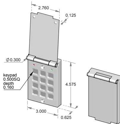
CS-KEKP-900 – Complete keyless entry keypad w/lift up cover.
