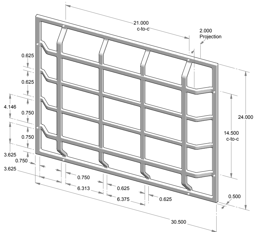
SEG-30524 – Speak easy grill. – 0.750" Wide grill on 2 outside bars. – 0.625" Wide grill on 2 inside bars.
