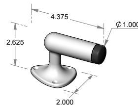
DS-2 – Floor mount door stop. – Includes mounting hardware for wood & masonry floors.
