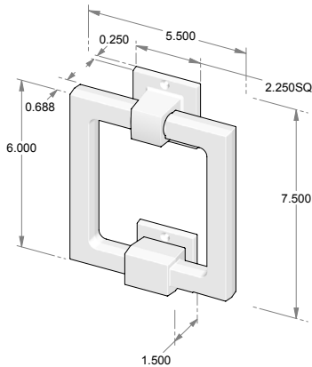
DK-96 – Square door knocker w/strike plate.
