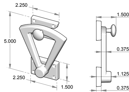
DDQ-1 – Dutch door quadrant.
