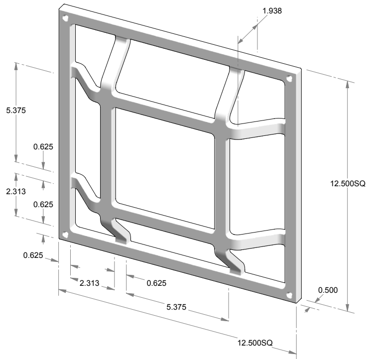
SEG-125125 – Speak easy grill. – Available 5/8" wide flat grill only.
