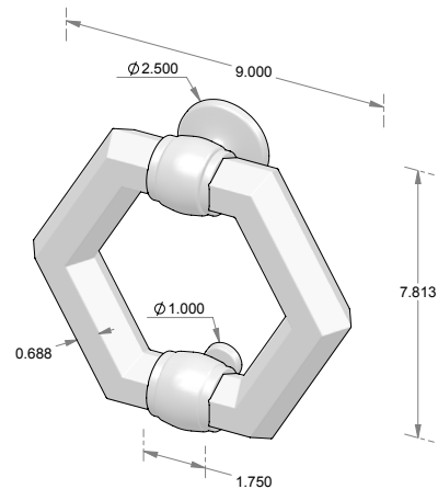
DK-2308 – Gem door knocker w/strike plate.
