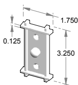
DRB-751 – Trellis door bell plate. – Matching solid bronze button.
