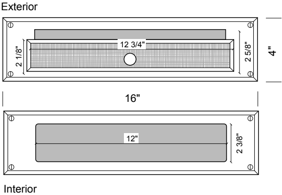
CS-MLST-2216 – Mail slot with Burlap door. – Includes interior trim.
