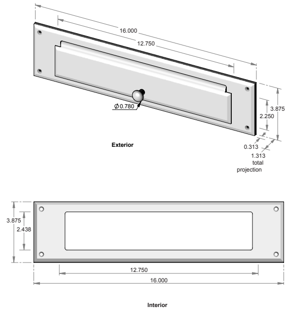
CS-MLST-16 – Mail slot with door. – Includes interior trim.
