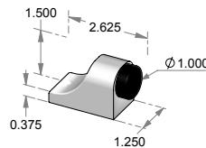
DS-10 – Floor mount door stop. – Includes mounting hardware for wood & masonry floors.
