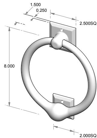
DKS-8 – Door knocker w/strike plate.
