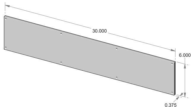
KP-9306 – Contemporary kick plate.
