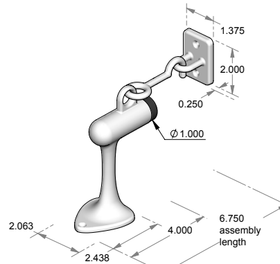
DS-9HE – Floor mount door stop. – Includes mounting hardware for wood and masonry floors.
