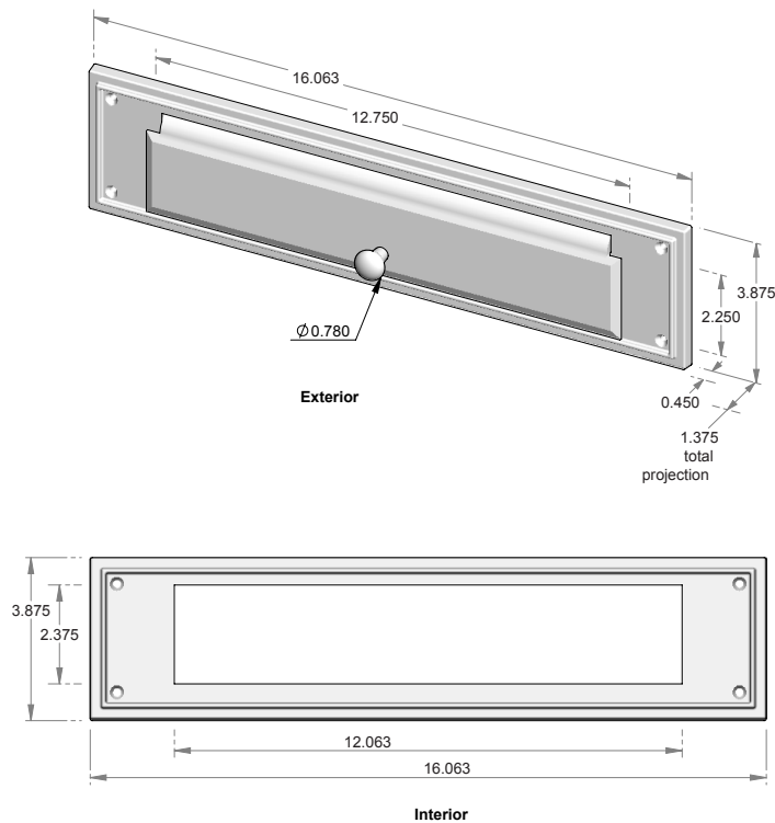
CS-MLST-R16 – Ridge mail slot with door. – Includes interior trim.
