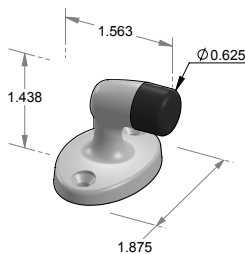
DS-1 – Floor mount door stop. – Includes mounting hardware for wood & masonry floors.
