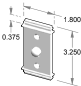
DRB-741 – Hampton door bell plate. – Matching solid bronze button.
