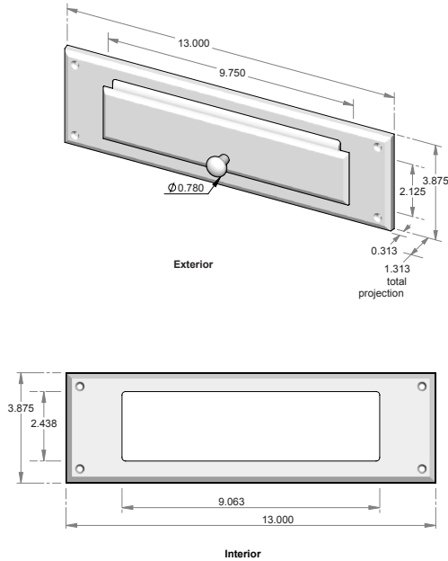
CS-MLST-13 – Mail slot with door. – Includes interior trim.
