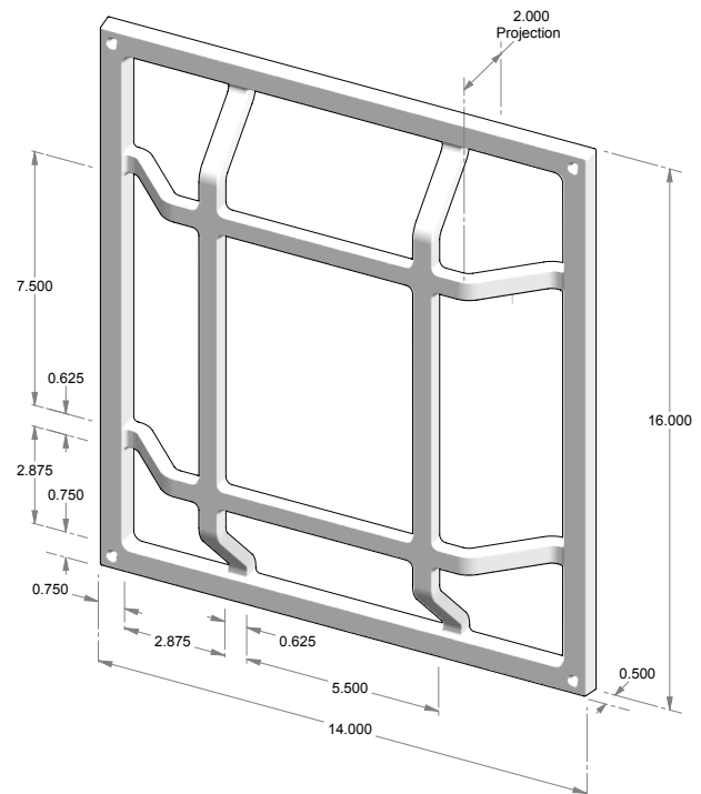
SEG-1014 – Speak easy grill. – Available 0.625" wide flat grill only.
