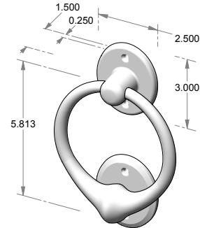
DK-5 – Door knocker w/strike plate.
