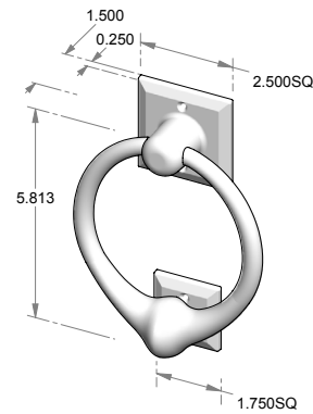
DKS-5 – Door knocker w/strike plate.
