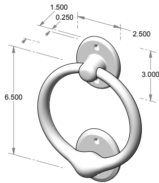
DK-3 – Door knocker w/strike plate.
