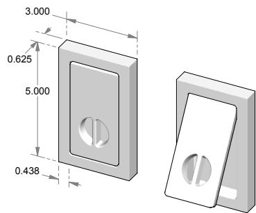
DK-J1FM – Flush mount door knocker w/attached strike plate.
