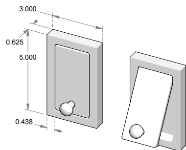
DK-J2FM – Flush mount door knocker w/attached strike plate.
