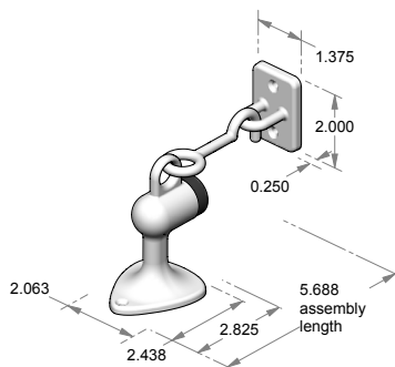
DS-2HE – Floor mount door stop w/hook & eye. – Includes mounting hardware for wood & masonry floors.
