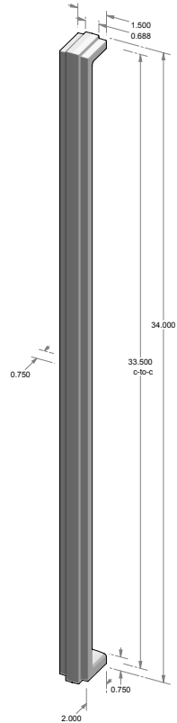
GH-961-34 - 33.500" center-to-center. - 1.500" handle width.
