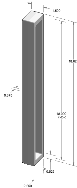
GH-2000-18* – 18.000" center-to-center. – 1.500" handle width. – *AVAILABLE BACK-TO-BACK. – *AVAILABLE BLIND MOUNT.
