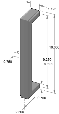
GH-2110* – 9.250" center-to-center. – 1.125" handle width. – 0.125" Handle step. – *AVAILABLE BACK-TO-BACK. – *AVAILABLE BLIND MOUNT.
