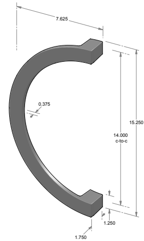
GH-R15* – 14.000" center-to-center. – 1.250" handle width. – *AVAILABLE BACK-TO-BACK. – *AVAILABLE BLIND MOUNT.
