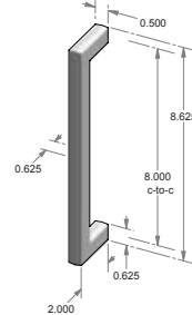
GH-1008* – Square grip handle. – 8.000" center-to-center. – 0.500" face width. – *AVAILABLE BACK-TO-BACK. – *AVAILABLE BLIND MOUNT.
