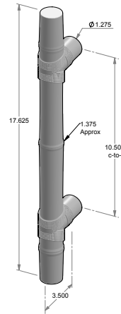
GH-1317R* – 10.500" center-to-center. – 1.275" handle width. – *AVAILABLE BACK-TO-BACK. – *AVAILABLE GLASS BACK-TO-BACK. – *AVAILABLE BLIND MOUNT.
