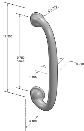
GH-345 - 9.7500" center-to-center. - 0.918" handle width.
