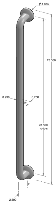
GH-525* – 23.500" center-to-center. – 0.938" handle width. – *AVAILABLE BACK-TO-BACK. – *AVAILABLE GLASS BACK-TO-BACK. – *AVAILABLE BLIND MOUNT.
