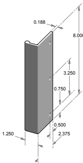
GH-B501-8R – Rolled edge mount grip handle.
