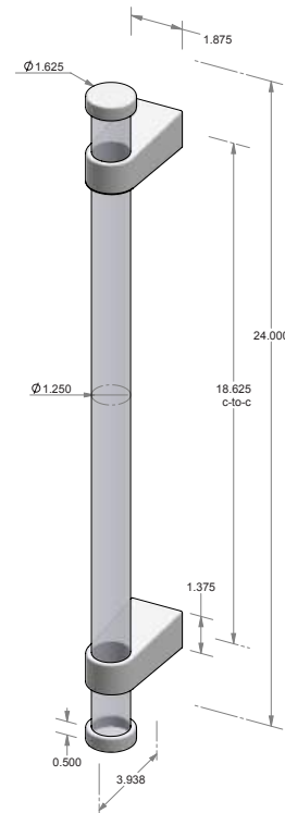
GH-ACR-DWL-CAP-24 – Acrylic grip handle w/caps. – 18.625" center-to-center. – Dowel available in acrylic, white oak or white oak w/black stain. – *AVAILABLE BLIND MOUNT.
