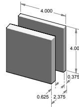
GH-KP225* – 4.000" Step knob pull. – 4.000" Square escutcheon included. – *AVAILABLE BACK-TO-BACK. – *AVAILABLE BLIND MOUNT.
