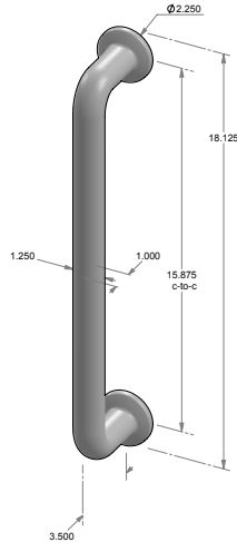
GH-552* – 15.875" center-to-center. – 1.250" handle width. – *AVAILABLE BACK-TO-BACK. – *AVAILABLE GLASS BACK-TO-BACK. – *AVAILABLE BLIND MOUNT.
