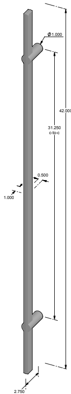
GH-RFH9142* – 31.250" center-to-center. – 0.500" face width. – *AVAILABLE BACK-TO-BACK. – *AVAILABLE GLASS BACK-TO-BACK. – *AVAILABLE BLIND MOUNT.
