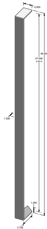
GH-9548* - 47.000" Center-to-center. - 2.000" handle width. - *AVAILABLE BACK-TO-BACK. - *AVAILABLE GLASS BACK-TO-BACK. - *AVAILABLE BLIND MOUNT.
