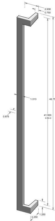
GH-996-42SL* – 41.500" center-to-center. – 1.313" handle width. – *AVAILABLE BACK-TO-BACK. – *AVAILABLE GLASS BACK-TO-BACK. – *AVAILABLE BLIND MOUNT.
