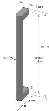
GH-165-12* – 12.000" Center-to-center. – 0.875" handle width. – *AVAILABLE BACK-TO-BACK. – *AVAILABLE GLASS BACK-TO-BACK. – *AVAILABLE BLIND MOUNT.
