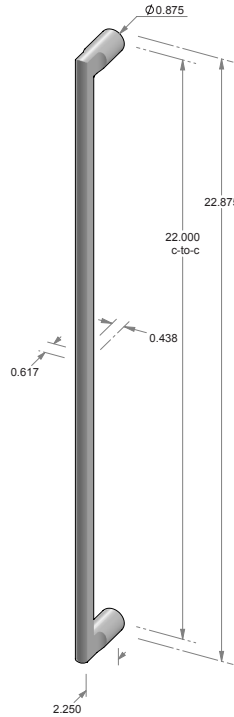
GH-1122* – 22.000" center-to-center. – 0.438" face width. – *AVAILABLE BACK-TO-BACK. – *AVAILABLE GLASS BACK-TO-BACK. – *AVAILABLE BLIND MOUNT.
