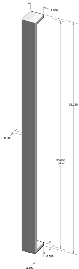
GH-974-36 – 35.688" center-to-center. – 2.000" handle width.
