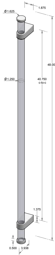
GH-ACR-DWL-CAP-48 - Acrylic grip handle w/caps. - 40.750" center-to-center. - Dowel available in acrylic, white oak or white oak w/black stain. - *AVAILABLE BLIND MOUNT.
