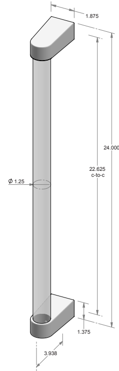
GH-ACR-DWL-24 – Acrylic grip handle. – 22.625" center-to-center. – Dowel available in acrylic, white oak or white oak w/black stain. – *AVAILABLE BLIND MOUNT.
