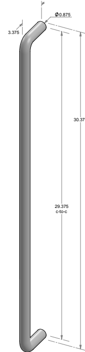
DH-30* – 29.375" center-to-center. – 0.875" handle width. – *AVAILABLE BACK-TO-BACK. – *AVAILABLE GLASS BACK-TO-BACK. – *AVAILABLE BLIND MOUNT.
