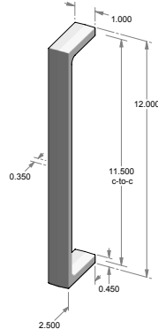
GH-983-12* – 11.500" center-to-center. – 1.000" handle width. – *AVAILABLE BACK-TO-BACK. – *AVAILABLE BLIND MOUNT.
