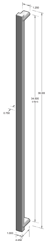
GH-9100-36* - 34.500" center-to-center. - 1.000" face width. - *AVAILABLE BACK-TO-BACK. - *AVAILABLE GLASS BACK-TO-BACK. - *AVAILABLE BLIND MOUNT.
