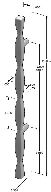
GH-CONVEX-24* - 12.600" center-to-center. - 0.9843 - 0.5118" handle face width. - *AVAILABLE BACK-TO-BACK. - *AVAILABLE GLASS BACK-TO-BACK. - *AVAILABLE BLIND MOUNT.
