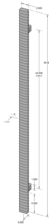
GH-630-55* – 43.500" center-to-center. – 2.000" handle width. – *AVAILABLE BACK-TO-BACK. – *AVAILABLE GLASS BACK-TO-BACK. – *AVAILABLE BLIND MOUNT.
