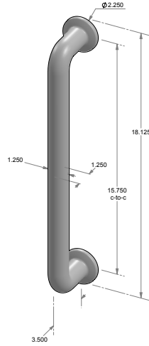
GH-553* – 15.750" center-to-center. – 1.250" handle width. – *AVAILABLE BACK-TO-BACK. – *AVAILABLE GLASS BACK-TO-BACK. – *AVAILABLE BLIND MOUNT.
