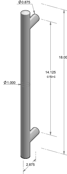
GH-150-18* – 14.125" Center-to-center. – 1.000" handle width. – *AVAILABLE BACK-TO-BACK. – *AVAILABLE GLASS BACK-TO-BACK. – *AVAILABLE BLIND MOUNT.
