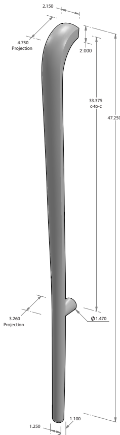
GH-747 - 33.375" center-to-center. - 2.150" handle width taper to 1.250".
