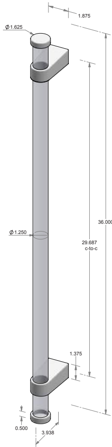
GH-ACR-DWL-CAP-36 - Acrylic grip handle w/caps. - 29.687" center-to-center. - Dowel available in acrylic, white oak or white oak w/black stain. - *AVAILABLE BLIND MOUNT.
