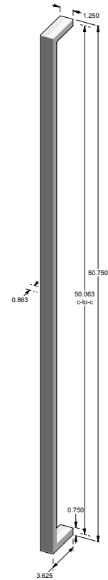
GH-998-50* – 50.063" center-to-center. – 1.250" handle width. – *AVAILABLE BACK-TO-BACK. – *AVAILABLE BLIND MOUNT.
