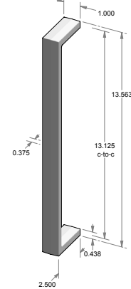
GH-985* – 13.125" center-to-center. – 1.000" handle width. – *AVAILABLE BACK-TO-BACK. – *AVAILABLE BLIND MOUNT.
