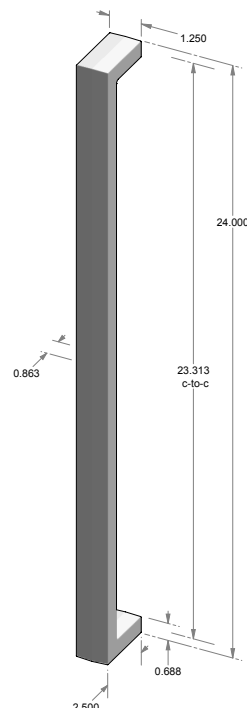
GH-999-24* – 23.313" center-to-center. – 1.250" handle width. – *AVAILABLE BACK-TO-BACK. – *AVAILABLE BLIND MOUNT.
