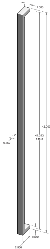
GH-999-1-42 – 41.312" Center-to-center. – 1.000" Handle width.
