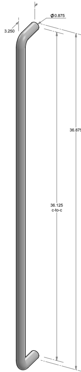
DH-36* – 36.125" center-to-center. – 0.875" handle width. – *AVAILABLE BACK-TO-BACK. – *AVAILABLE GLASS BACK-TO-BACK. – *AVAILABLE BLIND MOUNT.
