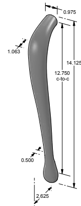
GH-714 – 12.750" center-to-center. – 0.975" handle width.
