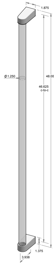
GH-ACR-DWL-48 – Acrylic grip handle. – 46.625" center-to-center. – Dowel available in acrylic, white oak or white oak w/black stain. – *AVAILABLE BLIND MOUNT.
