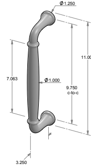
GH-142* – 9.750" center-to-center. – 1.250" handle width. – *AVAILABLE BACK-TO-BACK. – *AVAILABLE GLASS BACK-TO-BACK. – *AVAILABLE BLIND MOUNT.
