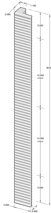
GH-6036* - 13.00" center-to-center (x2). - 3.000" handle width. - *AVAILABLE BACK-TO-BACK. - *AVAILABLE GLASS BACK-TO-BACK. - *AVAILABLE BLIND MOUNT.
