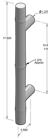
GH-1317* – 10.500" center-to-center. – 1.275" handle width. – *AVAILABLE BACK-TO-BACK. – *AVAILABLE GLASS BACK-TO-BACK. – *AVAILABLE BLIND MOUNT.
