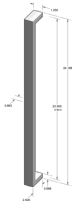
GH-998* – 23.625" center-to-center. – 1.250" handle width. – *AVAILABLE BACK-TO-BACK. – *AVAILABLE BLIND MOUNT.
