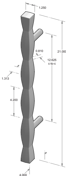
GH-CONVEX-21* - 12.625" center-to-center. - 1.250 - 0.810" handle face width. - *AVAILABLE BACK-TO-BACK. - *AVAILABLE GLASS BACK-TO-BACK. - *AVAILABLE BLIND MOUNT.
