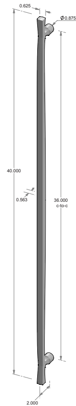
GH-228-40* – 36.000" center-to-center. – 0.625" handle width. – *AVAILABLE BACK-TO-BACK. – *AVAILABLE GLASS BACK-TO-BACK. – *AVAILABLE BLIND MOUNT.
