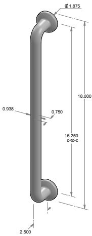
GH-550* – 16.250" center-to-center. – 0.938" handle width. – *AVAILABLE BACK-TO-BACK. – *AVAILABLE GLASS BACK-TO-BACK. – *AVAILABLE BLIND MOUNT.
