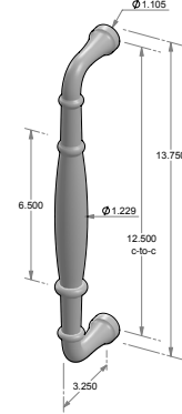
GH-143* – 12.500" center-to-center. – 1.105" handle width. – *AVAILABLE BACK-TO-BACK. – *AVAILABLE GLASS BACK-TO-BACK. – *AVAILABLE BLIND MOUNT.
