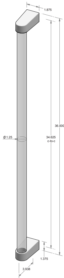
GH-ACR-DWL-36 – Acrylic grip handle. – 34.625" center-to-center. – Dowel available in acrylic, white oak or white oak w/black stain. – *AVAILABLE BLIND MOUNT.
