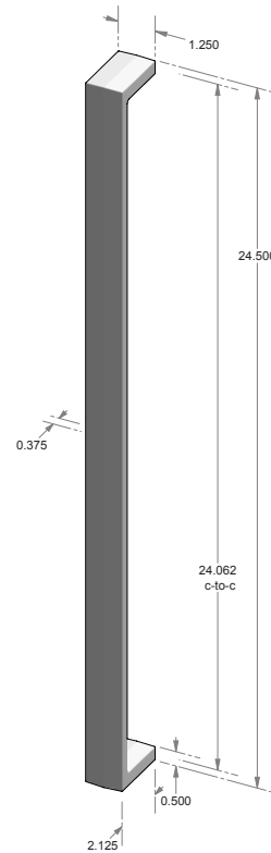
GH-924 – 24.062" center-to-center. – 1.250" handle width.
