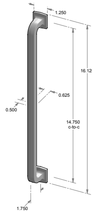
GH-559* – 14.750" center-to-center. – 0.625" square handle width. – *AVAILABLE BACK-TO-BACK. – *AVAILABLE GLASS BACK-TO-BACK. – *AVAILABLE BLIND MOUNT.
