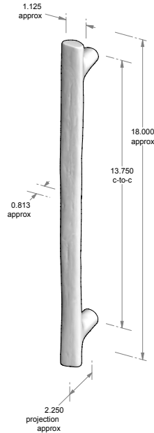
GH-728 – 13.750" center-to-center. – 1.125" approximate face width.
