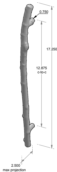
GH-TWG18 – 12.875" center-to-center. – 0.750" handle width.
