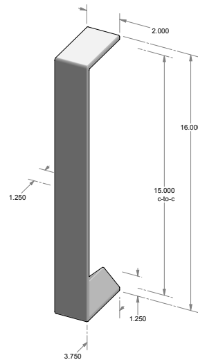
GH-9516* - 15.000" center-to-center. - 2.000" Handle width. - Underside of grip handle is v-shaped. - *AVAILABLE BACK-TO-BACK. - *AVAILABLE BLIND MOUNT.
