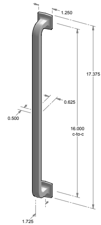
GH-560* – 16.000" center-to-center. – 0.625" square handle width. – *AVAILABLE BACK-TO-BACK. – *AVAILABLE GLASS BACK-TO-BACK. – *AVAILABLE BLIND MOUNT.
