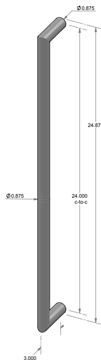
GH-169-24* – 24.000" Center-to-center. – 0.875" handle width. – *AVAILABLE BACK-TO-BACK. – *AVAILABLE GLASS BACK-TO-BACK. – *AVAILABLE BLIND MOUNT.
