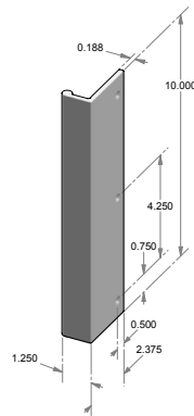
GH-B501-10R – Rolled edge mount grip handle.
