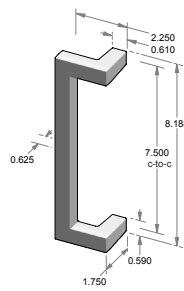
GH-131SL* – 7.500" center-to-center. – 0.625" handle width. – *AVAILABLE BACK-TO-BACK. – *AVAILABLE BLIND MOUNT.
