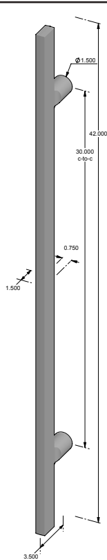
GH-9142* – 30.000" center-to-center. – 0.750" face width. – *AVAILABLE BACK-TO-BACK. – *AVAILABLE GLASS BACK-TO-BACK. – *AVAILABLE BLIND MOUNT.
