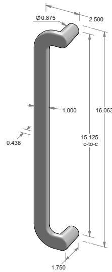
GH-116SL* – 15.125" center-to-center. – 1.000" handle width. – *AVAILABLE BACK-TO-BACK. – *AVAILABLE GLASS BACK-TO-BACK. – *AVAILABLE BLIND MOUNT.
