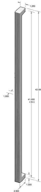
GH-1983-42* – 41.000" center-to-center. – 1.250" handle width. – *AVAILABLE BACK-TO-BACK. – *AVAILABLE GLASS BACK-TO-BACK. – *AVAILABLE BLIND MOUNT.
