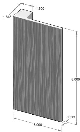
GH-1966-8-C* – 6.000" handle width. – 6.000" center-to-center. – *AVAILABLE BACK-TO-BACK. – *AVAILABLE GLASS BACK-TO-BACK. – *AVAILABLE BLIND MOUNT.
