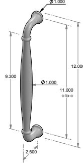
GH-141-12* – 11.000" center-to-center. – 1.000" handle width. – *AVAILABLE BACK-TO-BACK. – *AVAILABLE GLASS BACK-TO-BACK. – *AVAILABLE BLIND MOUNT.
