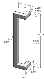
GH-132SL* – 9.625" center-to-center. – 0.625" handle width. – *AVAILABLE BACK-TO-BACK. – *AVAILABLE BLIND MOUNT.
