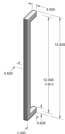
GH-1012* – Square grip handle. – 12.000" center-to-center. – 0.500" face width. – *AVAILABLE BACK-TO-BACK. – *AVAILABLE BLIND MOUNT.
