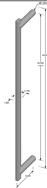
GH-9148* – 44.000" center-to-center. – 0.750" face width. – *AVAILABLE BACK-TO-BACK. – *AVAILABLE GLASS BACK-TO-BACK. – *AVAILABLE BLIND MOUNT.
