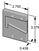
GL-RB-STRIKE – Left hand reverse shown.
