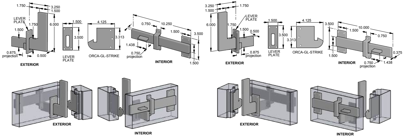
ORCA-CS-GL-LH – Complete passage set. – Left hand.
