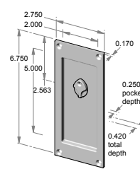
FP-404ERC – 2.750" x 6.750" x 0.420" thick. – 0.250" interior depth.
