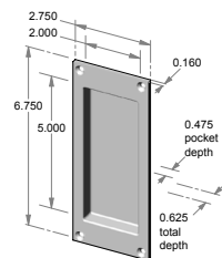
FP-405 – 2.750" x 6.750" x 0.625" thick. – 0.475" interior depth.
