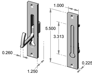
EDG-155 – 5.500" edge pull w/hook.
