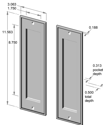
CS-FP1516IML – Complete passage set. OR TS-FP1516IML – Trim set only.
