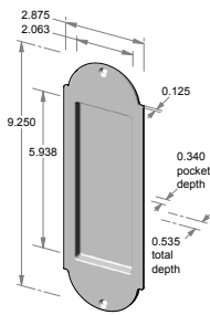
FP-A402 – 2.875" x 9.250" x 0.535" thick. – 0.340" interior depth.
