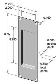
FP-451 – 2.750" x 8.750" x 0.650" thick. – 0.500" interior depth.
