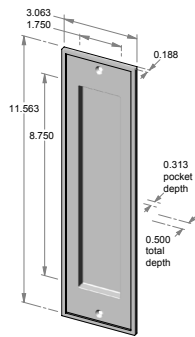
FP-1516 – 3.063" x 11.563" x 0.500" thick. – 0.313" interior depth.
