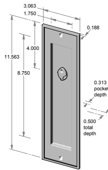
FP-1516ERC – 3.063" x 11.563" x 0.500" thick. – 0.313" interior depth.
