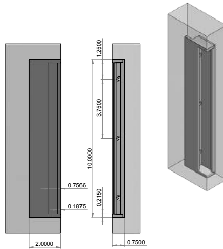
FEP-210BM – Blind mount flush edge pull.
