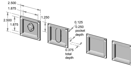
CS-FP2525IML-DBL-PR – Complete double privacy set. OR TS-FP2525IML-DBL-PR – Trim set only.
