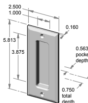
FP-504 – 2.500" x 5.813" x 0.750" thick. – 0.563" interior depth.
