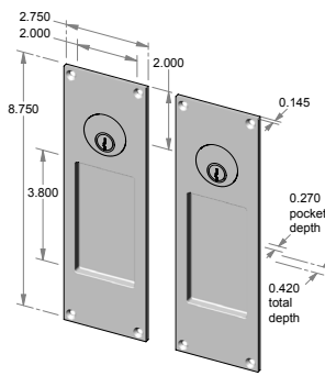
CS-FP450ML-DC – Complete double cylinder set. OR TS-FP450ML-DC – Trim set only.
