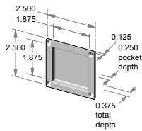
FP-2525 – 2.500" x 2.500" x 0.375" thick. – 0.250" interior depth.
