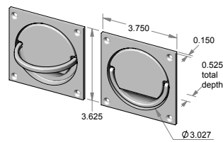
SQFP-358 – Squash court flush pull. – Eased edge. – Surface mount.
