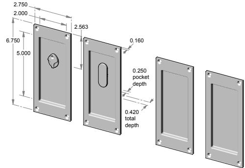
CS-FP404IML-DBL-PR – Complete double privacy set. OR TS-FP404IML-DBL-PR – Trim set only.
