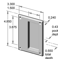
FP-505 (rolled edge) – 3.300" x 4.850" x 0.550" thick. – 0.430" interior depth.
