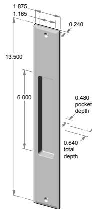
FP-308 – 1.875" x 13.500" x 0.640" thick. – 0.480" interior depth.
