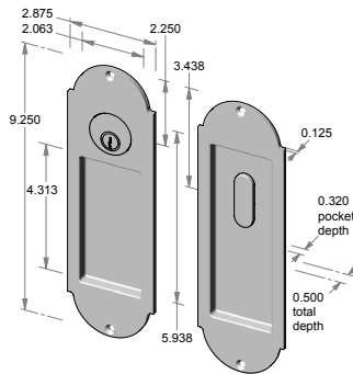
CS-FP-A402ML – Complete single cylinder set. OR TS-FP-A402ML – Trim set only.
