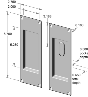
CS-FP451ML-PF – Complete patio function set. OR TS-FP451ML-PF – Trim set only.
