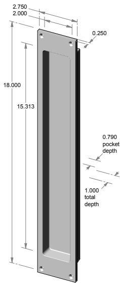
FP-454-18-1 – 2.750" x 18.000" x 1.000" thick. – 0.790" interior depth.
