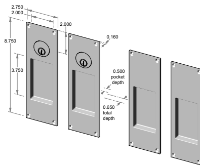
CS-FP451ML-DBL-DC – Complete double cylinder set. OR TS-FP451ML-DBL-DC – Trim set only.
