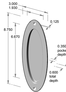
FP-OP700 – 3" x 8 3/4" x 1/2" thick. – 3/8" interior depth.
