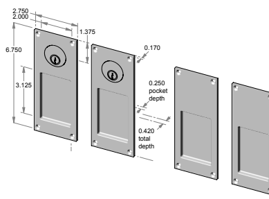
CS-FP404ML-DBL-DC – Complete double cylinder set. OR TS-FP404ML-DBL-DC – Trim set only.
