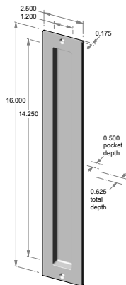
FP-316 – 2.500" x 16.000" x 0.625" thick. – 0.500" interior depth.
