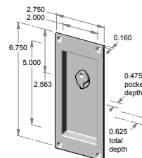
FP-405ERC – 2.750" x 6.750" x 0.625" thick. – 0.475" interior depth.
