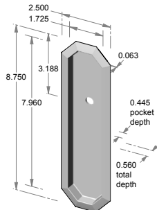
FP-2351ER – 2.500" x 8.750" x 0.560" thick. – 0.455" interior depth.
