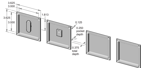
CS-FP358-3/8-IML-DBL-PR – Complete double privacy set. OR TS-FP358-3/8-IML-DBL-PR – Trim set only.
