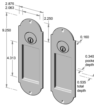
CS-FP-A402ML-DC – Complete double cylinder set. OR TS-FP-A402ML-DC – Trim set only.
