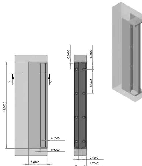
FEP-212DBL-T-1 3/4 – Edge flush pull w/T-tab back-to-back. – Requires a door thickness of 1.750".
