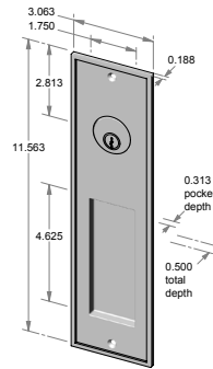
FP-1516K – 3.063" x 11.563" x 0.500" thick. – 0.313" interior depth.
