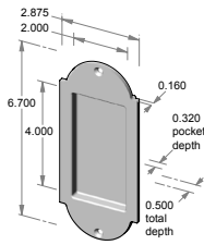
FP-A400 – 2.875" x 6.700" x 0.500" thick. – 0.320" interior depth.
