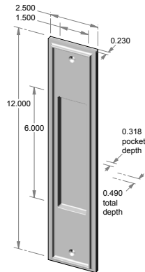
FP-423 – 2.500" x 12.000" x 0.490" thick. – 0.318" interior depth. – Ridge 0.63" high.
