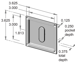
FP-358-3/8-TPC – 3.625" x 3.625" x 0.375" thick. – 0.250" interior depth.
