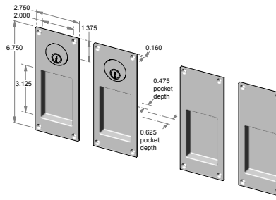
CS-FP405ML-DBL-DC – Complete double cylinder set. OR TS-FP405ML-DBL-DC – Trim set only.
