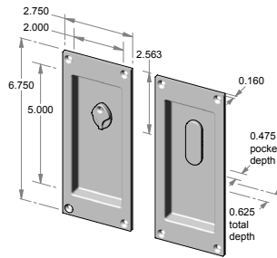
CS-FP405IML-PR – Complete privacy set. OR TS-FP405IML-PR – Trim set only.
