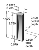
FP-206 – 0.9375" x 4.000" x 0.500" thick. – 0.400" interior depth. – Machine screws into back of flush pull.
