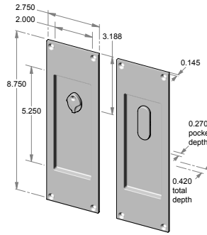
CS-FP450IML-PR – Complete privacy set. OR TS-FP450IML-PR – Trim set only.
