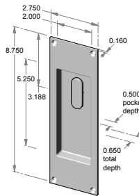
FP-451TPC – 2.750" x 8.750" x 0.650" thick. – 0.500" interior depth.
