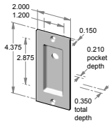
FP-203ER – 2.000" x 4.375" x 0.350" thick. – 0.210" interior depth.
