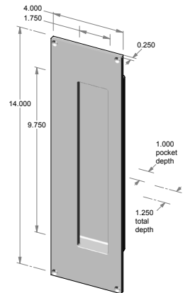
FP-514 – 4.000" x 14.000" x 1.250" thick. – 1.000" interior depth.
