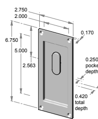
FP-404TPC – 2.750" x 6.750" x 0.420" thick. – 0.250" interior depth.
