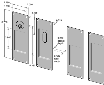
CS-FP450ML-DBL – Complete single cylinder set. OR TS-FP450ML-DBL – Trim set only.
