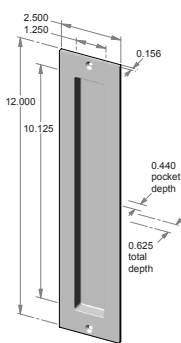
FP-312 – 2.500" x 11.938" x 0.625" thick. – 0.440" interior depth.
