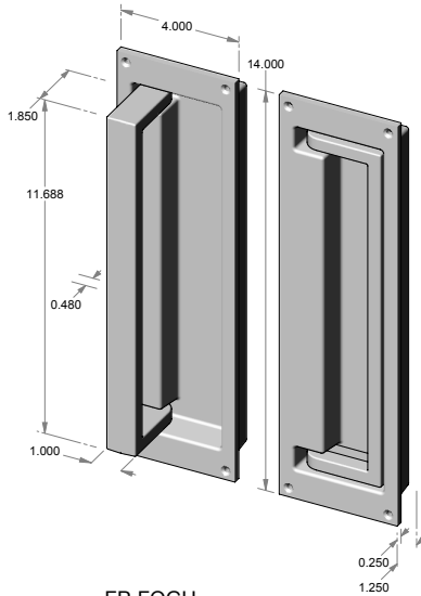
FP-FOGH – Fold out grip handle. – 4.000" x 14.000" x 1.250" thick. – 1.000" interior depth.
