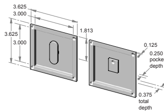
CS-FP358-3/8-IML-PR – Complete privacy set. OR TS-FP358-3/8-IML-PR – Trim set only.
