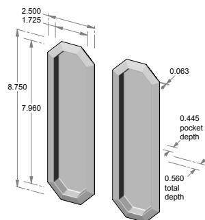
CS-FP2351IML – Complete passage set. OR TS-FP2351IML – Trim set only.
