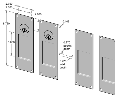
CS-FP450ML-DBL-DC – Complete double cylinder set. OR TS-FP450ML-DBL-DC – Trim set only.
