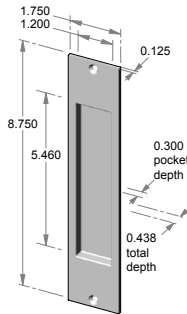
FP-475 – 1.750" x 8.750" x 0.438" thick. – 0.300" interior depth.
