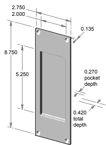
FP-450 – 2.750" x 8.750" x 0.420" thick. – 0.270" interior depth.
