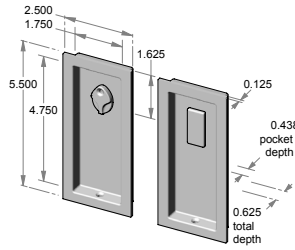
CS-FP303IML-PR – Complete privacy set. OR TS-FP303IML-PR – Trim set only.
