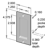
FP-202 – 2.000" x 4.375" x 0.360" thick. – 0.230" interior depth.
