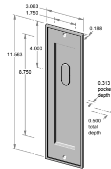
FP-1516TPC – 3.063" x 11.563" x 0.500" thick. – 0.313" interior depth.
