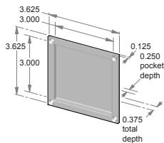
FP-358-3/8 – 3.625" x 3.625" x 0.375" thick. – 0.250" interior depth.
