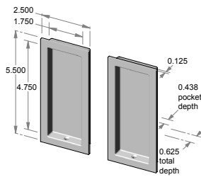
CS-FP303IML – Complete passage set. OR TS-FP303IML – Trim set only.
