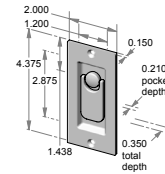
FP-203FK – 2.000" x 4.375" x 0.350" thick. – 0.210" interior depth.
