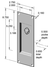
FP-451ERC – 2.750" x 8.750" x 0.650" thick. – 0.500" interior depth.
