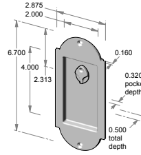
FP-A401ERC – 2.875" x 6.700" x 0.500" thick. – 0.320" interior depth.
