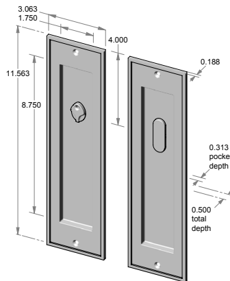
CS-FP1516IML-PR – Complete privacy set. OR TS-FP1516IML-PR – Trim set only.
