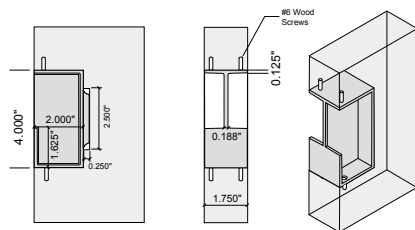
FEP-T4-175 – Edge flush pull w/tab. – Requires a door thickness of 1.750”.
