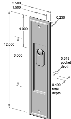
FP-423TPC – 2.500" x 12.000" x 0.490" thick. – 0.318" interior depth. – Ridge 0.63" high.
