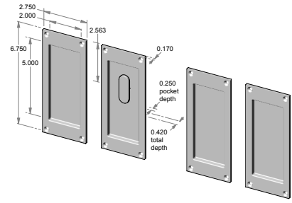
CS-FP404ML-DBL-PF – Complete patio function set. OR TS-FP404ML-DBL-PF – Trim set only.
