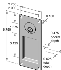
FP-405K – 2.750" x 6.750" x 0.625" thick. – 0.475" interior depth.
