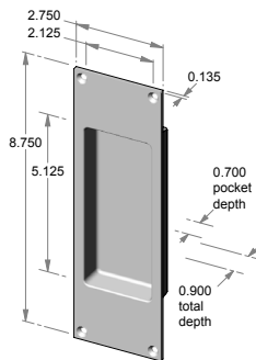
FP-452 – 2.750" x 8.750" x 0.900" thick. – 0.700" interior depth.
