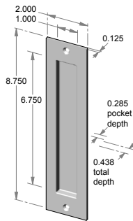
FP-309-7/16 – 2.000" x 8.750" x 0.438" thick. – 0.285" interior depth.
