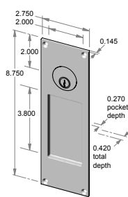
FP-450K – 2.750" x 8.750" x 0.420" thick. – 0.270" interior depth.
