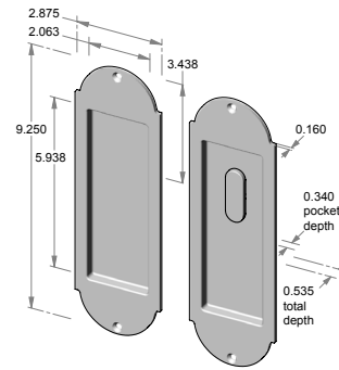
CS-FP-A402ML-PF – Complete patio function set. OR TS-FP-A402ML-PF – Trim set only.
