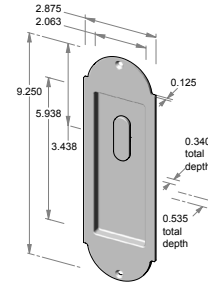
FP-A402TPC – 2.875" x 9.250" x 0.535" thick. – 0.340" interior depth.
