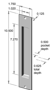
FP-307 – 1.750" x 10.500" x 0.625" thick. – 0.500" interior depth.
