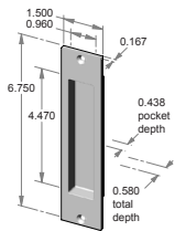
FP-205 – 1.500" x 6.750" x 0.580" thick. – 0.438" interior depth.
