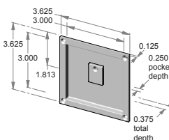
FP-358-3/8-RC-7 – 3.625" x 3.625" x 0.375" thick. – 0.250" interior depth.
