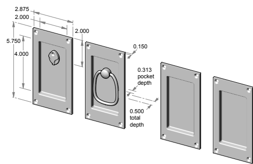
CS-FP401IML-DBL-PR – Complete double privacy set. OR TS-FP401IML-DBL-PR – Trim set only.
