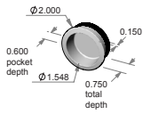
FP-RP150 – 2.000" round x 0.750" thick. – 0.600" interior depth.
