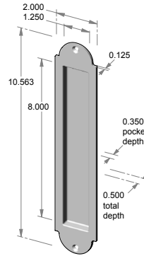
FP-A309 – 2.000" x 10.563" x 0.500" thick. – 0.350" interior depth.
