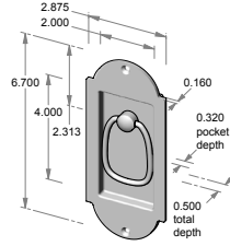
FP-A401FR – 2.875" x 6.700" x 0.500" thick. – 0.320" interior depth.
