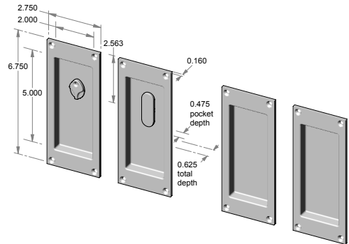
CS-FP405IML-DBL-PR – Complete double privacy set. OR TS-FP405IML-DBL-PR – Trim set only.
