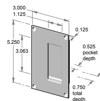
FP-500 – 3.000" x 5.250" x 0.750" thick. – 0.525" interior depth.
