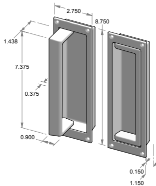
FP-409FOGH – Fold out grip handle. – 2.750" x 8.750" x 1.150" thick. – 1.000" interior depth.
