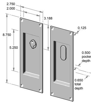
CS-FP451IML-PR – Complete privacy set. OR TS-FP451IML-PR – Trim set only.
