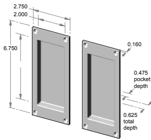
CS-FP405IML – Complete passage set. OR TS-FP405IML – Trim set only.
