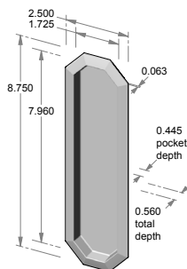
FP-2351 – 2.500" x 8.750" x 0.560" thick. – 0.455" interior depth.
