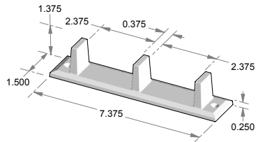
BPG-214 – 2.250" thick doors.
