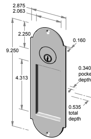
FP-A402K – 2.875" x 9.250" x 0.535" thick. – 0.340" interior depth.
