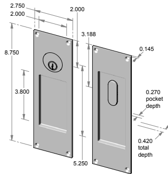
CS-FP450ML – Complete single cylinder set. OR TS-FP450ML – Trim set only.
