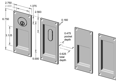
CS-FP405ML-DBL – Complete single cylinder set. OR TS-FP405ML-DBL – Trim set only.
