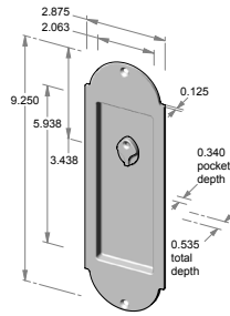
FP-A402ERC – 2.875" x 9.250" x 0.535" thick. – 0.340" interior depth.
