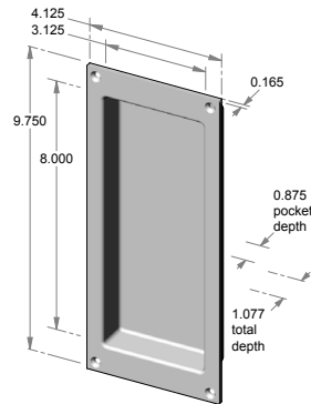
FP-509 – 4.125" x 9.750" x 1.077" thick. – 0.875" interior depth.
