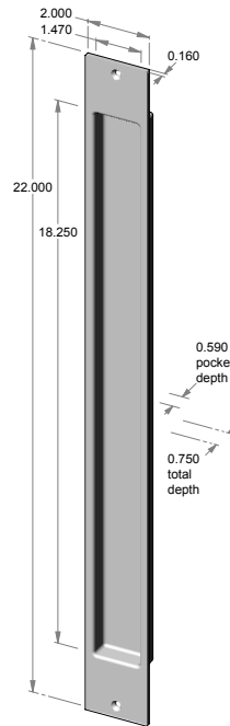
FP-2500 – 2.000" x 22.000" x 0.750" thick. – 0.590" interior depth.
