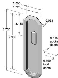
FP-2351TPC – 2.500" x 8.750" x 0.560" thick. – 0.455" interior depth.
