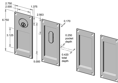
CS-FP404ML-DBL – Complete single cylinder set. OR TS-FP404ML-DBL – Trim set only.
