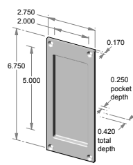
FP-404 – 2.750" x 6.750" x 0.420" thick. – 0.250" interior depth.
