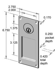
FP-404K – 2.750" x 6.750" x 0.420" thick. – 0.250" interior depth.
