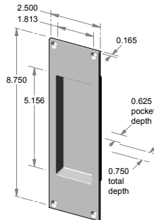
FP-445 – 2.500" x 8.750" x 0.750" thick. – 0.625" interior depth.
