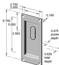
FP-405TPC – 2.750" x 6.750" x 0.625" thick. – 0.475" interior depth.
