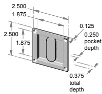
FP-2525WTPC – 2.500" x 2.500" x 0.375" thick. – 0.250" interior depth.
