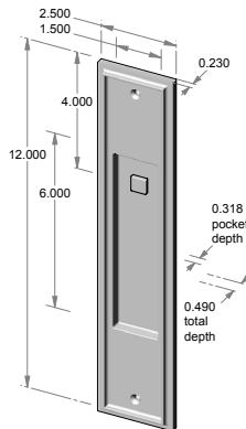
FP-423ER-13PLUG – 2.500" x 12.000" x 0.490" thick. – 0.318" interior depth. – Ridge 0.63" high.
