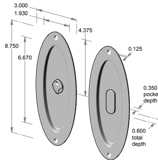
CS-FP-OP700IML-PR – Complete privacy set. OR TS-FP-OP700IML-PR – Trim set only.
