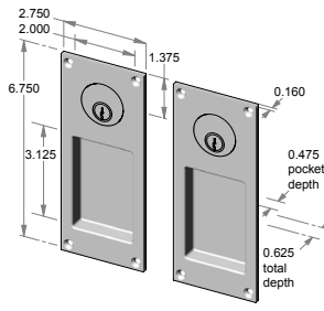
CS-FP405ML-DC – Complete double cylinder set. OR TS-FP405ML-DC – Trim set only.
