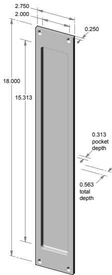
FP-454-18 – 2.750" x 18.000" x 0.563" thick. – 0.313" interior depth.
