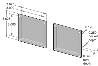
CS-FP358-3/8-IML – Complete passage set. OR TS-FP358-3/8-IML – Trim set only.
