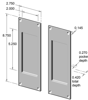
CS-FP450IML – Complete passage set. OR TS-FP450IML – Trim set only.
