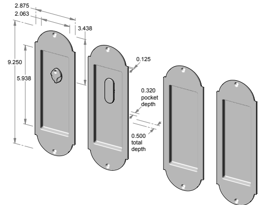
CS-FP-A402IML-DBL-PR – Complete double privacy set. OR TS-FP-A402IML-DBL-PR – Trim set only.
