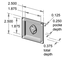
FP-2525RC – 2.500" x 2.500" x 0.375" thick. – 0.250" interior depth.
