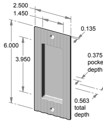
FP-1406 – 2.500" x 6.000" x 0.563" thick. – 0.375" interior depth.
