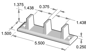
BPG-138 – 1.376" thick doors.
