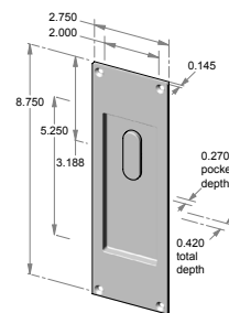
FP-450TPC – 2.750" x 8.750" x 0.420" thick. – 0.270" interior depth.
