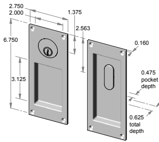
CS-FP405ML – Complete single cylinder set. OR TS-FP405ML – Trim set only.
