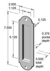
FP-A407 – 2.000" x 7.500" x 0.500" thick. – 0.320" interior depth.
