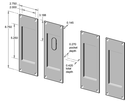
CS-FP450ML-DBL-PF – Complete patio function set. OR TS-FP450ML-DBL-PF – Trim set only.
