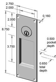
FP-451K – 2.750" x 8.750" x 0.650" thick. – 0.500" interior depth.
