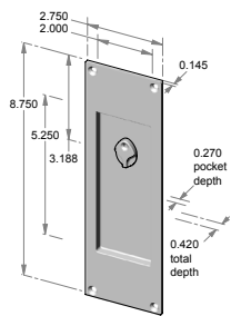
FP-450ERC – 2.750" x 8.750" x 0.420" thick. – 0.270" interior depth.
