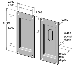
CS-FP405ML-PF – Complete patio function set. OR TS-FP405ML-PF – Trim set only.
