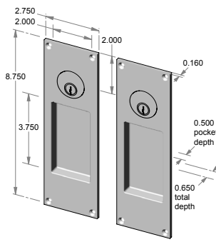
CS-FP451ML-DC – Complete double cylinder set. OR TS-FP451ML-DC – Trim set only.
