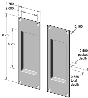
CS-FP451IML – Complete passage set. OR TS-FP451IML – Trim set only.
