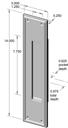
FP-425 – 3.000" x 14.000" x 0.975" thick. – 0.625" interior depth. – Ridge 0.63" high.
