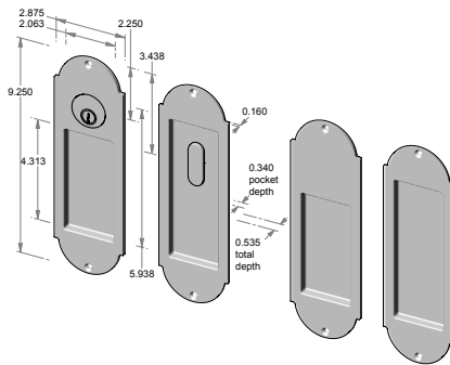
CS-FP-A402ML-DBL – Complete single cylinder set. OR TS-FP-A402ML-DBL – Trim set only.
