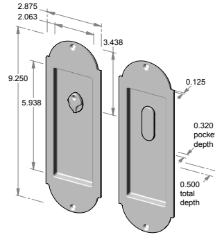
CS-FP-A402IML-PR – Complete privacy set. OR TS-FP-A402IML-PR – Trim set only.
