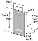
FP-200 – 2.000" x 4.375" x 0.360" thick. – 0.210" interior depth.
