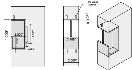
FEP-T4-2 – Edge flush pull w/tab. – Requires a door thickness of 2.000”.
