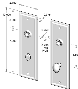
CS-F426PLMB – Complete set w/passage latch, mortise bolt & spindle. OR – TS-F426PLMB – Trim set only. No latch or mortise bolt. – Shown w/RC-4.
