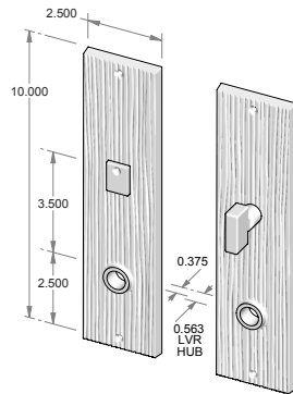
CS-1910PLMB – Complete set with passage latch, mortise bolt and spindle. OR TS-1910PLMB – Trim set only. No latch or mortise bolt. – Shown w/RC-7.
