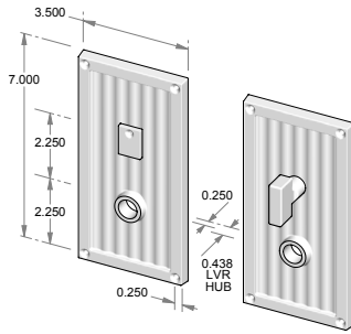
CS-336PLMB – Complete set w/passage latch, mortise bolt & spindle. OR – TS-336PLMB – Trim set only. No latch or mortise bolt. – Shown w/ RC-7.
