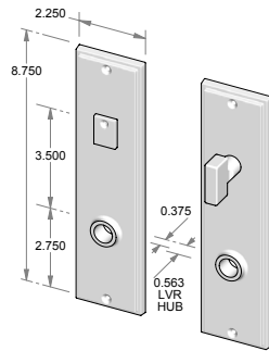
CS-2108PLMB – Complete set with passage latch, mortise bolt and spindle. OR TS-2108PLMB – Trim set only. No latch or mortise bolt. – Shown w/RC-7.
