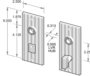
CS-F1406PLMB – Complete set with passage latch, mortise bolt and spindle. OR TS-F1406PLMB – Trim set only. No latch or mortise bolt. – Shown w/RC-7.
