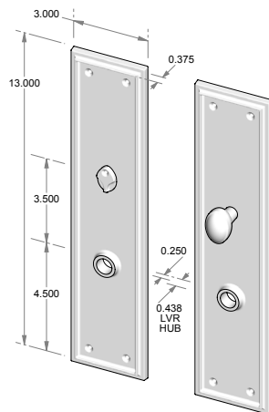
CS-425PLMB – Complete set w/passage latch, mortise bolt & spindle. OR – TS-425PLMB – Trim set only. No latch or mortise bolt. – Shown w/RC-4.
