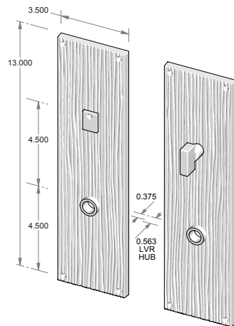
CS-1913PLMB – Complete set with passage latch, mortise bolt and spindle. OR TS-1913PLMB – Trim set only. No latch or mortise bolt. – Shown w/RC-7.
