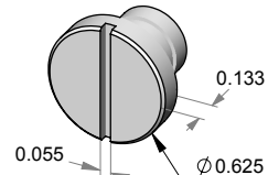
CR-9-2 Contemporary coin release. NOT available w/indicator.
