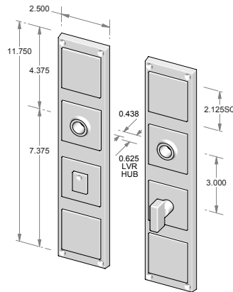
CS-F1811PLMB – Complete set with passage latch, mortise bolt and spindle. OR TS-F1811PLMB – Trim set only. No latch or mortise bolt.
