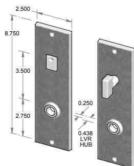
CS-2208PLMB – Complete set with passage latch, mortise bolt and spindle. OR TS-2208PLMB – Trim set only. No latch or mortise bolt. – Shown w/RC-7.
