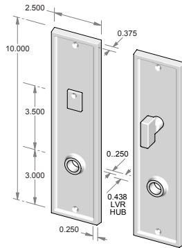
CS-1510PLMB – Complete set with passage latch, mortise bolt and spindle. OR TS-1510PLMB – Trim set only. No latch or mortise bolt. – Shown w/RC-7.
