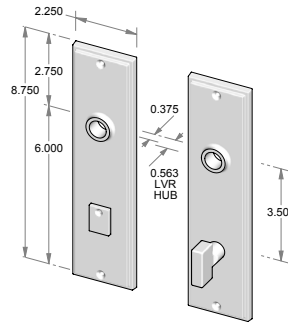
CS-F2108PLMB – Complete set with passage latch, mortise bolt and spindle. OR TS-F2108PLMB – Trim set only. No latch or mortise bolt. – Shown w/RC-7.
