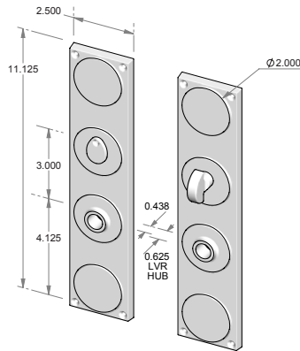
CS-1711PLMB – Complete set with passage latch, mortise bolt and spindle. OR TS-1711PLMB – Trim set only. No latch or mortise bolt. – Shown w/RC-9.
