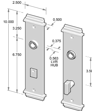
CS-F440PLMB – Complete set w/passage latch, mortise bolt & spindle. OR – TS-F440PLMB – Trim set only. No latch or mortise bolt. – Shown w/RC-7.
