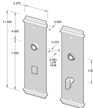
CS-F441PLMB – Complete set w/passage latch, mortise bolt & spindle. OR – TS-F441PLMB – Trim set only. No latch or mortise bolt. – Shown w/ RC-7.
