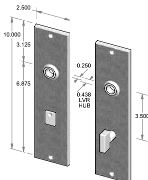
CS-F2210PLMB – Complete set with passage latch, mortise bolt and spindle. OR TS-F2210PLMB – Trim set only. No latch or mortise bolt. – Shown w/RC-7.
