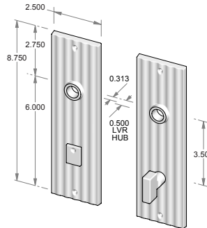
CS-F1408PLMB – Complete set with passage latch, mortise bolt and spindle. OR TS-F1408PLMB – Trim set only. No latch or mortise bolt. – Shown w/RC-7.
