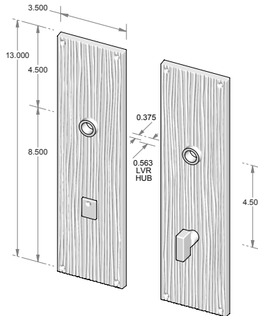
CS-F1913PLMB – Complete set with passage latch, mortise bolt and spindle. OR TS-F1913PLMB – Trim set only. No latch or mortise bolt. – Shown w/RC-7.
