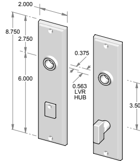
CS-F2107PLMB – Complete set with passage latch, mortise bolt and spindle. OR TS-F2107PLMB – Trim set only. No latch or mortise bolt. – Shown w/RC-7.
