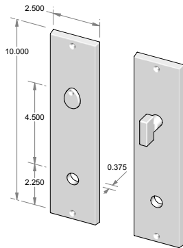
CS-N952PLMB – Complete set w/passage latch, mortise bolt & spindle. OR – TS-N952PLMB – Trim set only. No latch or mortise bolt. – Shown w/RC-9.
