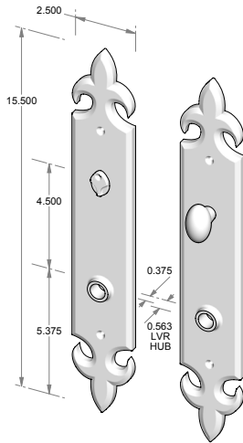
CS-1245PLMB – Complete set with passage latch, mortise bolt and spindle. OR TS-1245PLMB – Trim set only. No latch or mortise bolt. – Shown w/RC-4.
