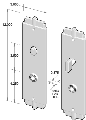
CS-461PLMB – Complete set w/passage latch, mortise bolt & spindle. OR – TS-461PLMB – Trim set only. No latch or mortise bolt. – Shown w/RC-9.
