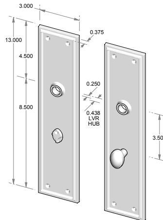
CS-F425PLMB – Complete set w/passage latch, mortise bolt & spindle. OR – TS-F425PLMB – Trim set only. No latch or mortise bolt. – Shown w/RC-4.
