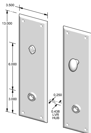
CS-602PLMB – Complete set w/passage latch, mortise bolt & spindle. OR – TS-602PLMB – Trim set only. No latch or mortise bolt. – Shown w/RC-4.
