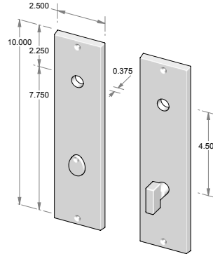
CS-F-N952PLMB – Complete set w/passage latch, mortise bolt & spindle. OR – TS-F-N952PLMB – Trim set only. No latch or mortise bolt. – Shown w/RC-9.
