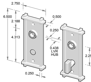
CS-F355PLMB – Complete set w/passage latch, mortise bolt & spindle. OR – TS-F355PLMB – Trim set only. No latch or mortise bolt.
