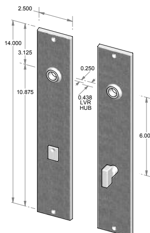
CS-F2214PLMB – Complete set with passage latch, mortise bolt and spindle. OR TS-F2214PLMB – Trim set only. No latch or mortise bolt. – Shown w/RC-7.
