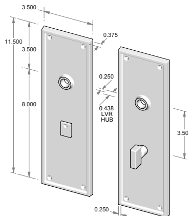
CS-F1512PLMB – Complete set with passage latch, mortise bolt and spindle. OR TS-F1512PLMB – Trim set only. No latch or mortise bolt. – Shown w/RC-7.
