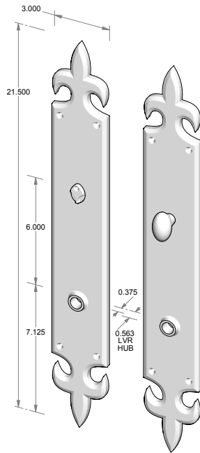
CS-1250PLMB – Complete set with passage latch, mortise bolt and spindle. OR TS-1250PLMB – Trim set only. No latch or mortise bolt. – Shown w/RC-4.
