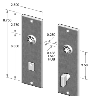
CS-F2208PLMB – Complete set with passage latch, mortise bolt and spindle. OR TS-F2208PLMB – Trim set only. No latch or mortise bolt. – Shown w/RC-7.
