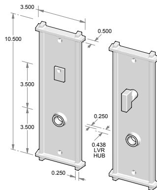
CS-451PLMB – Complete set w/passage latch, mortise bolt & spindle. OR – TS-451PLMB – Trim set only. No latch or mortise bolt. – Shown w/RC-7.
