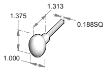
ERK-306 – Emergency release key.
