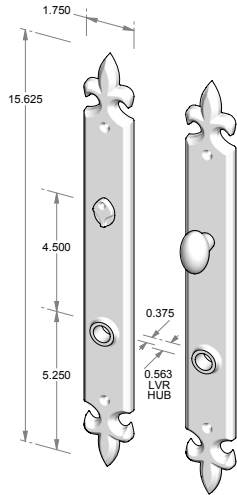
CS-1240PLMB – Complete set with passage latch, mortise bolt and spindle. OR TS-1240PLMB – Trim set only. No latch or mortise bolt. – Shown w/RC-4.
