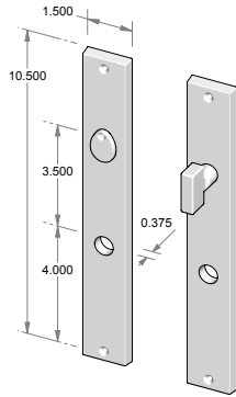
CS-N980PLMB – Complete set w/passage latch, mortise bolt & spindle. OR – TS-N980PLMB – Trim set only. No latch or mortise bolt. – Shown w/RC-9.
