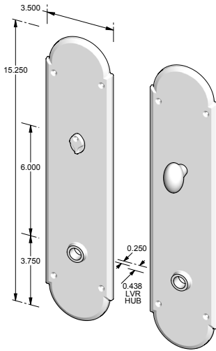
CS-A602PLMB – Complete set w/passage latch, mortise bolt & spindle. OR – TS-A602PLMB – Trim set only. No latch or mortise bolt. – Shown w/RC-4.
