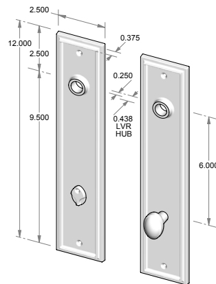
CS-F423PLMB – Complete set w/passage latch, mortise bolt & spindle. OR – TS-F423PLMB – Trim set only. No latch or mortise bolt. – Shown w/RC-4.
