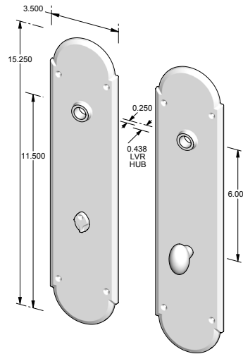
CS-F-A602PLMB – Complete set w/passage latch, mortise bolt & spindle. OR – TS-F-A602PLMB – Trim set only. No latch or mortise bolt. – Shown w/RC-4.
