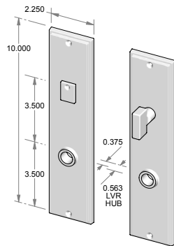
CS-2110PLMB – Complete set with passage latch, mortise bolt and spindle. OR TS-2110PLMB – Trim set only. No latch or mortise bolt. – Shown w/RC-7.
