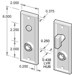
CS-1505PLMB – Complete set with passage latch, mortise bolt and spindle. OR TS-1505PLMB – Trim set only. No latch or mortise bolt.
