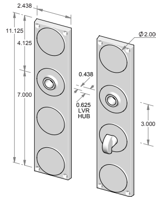
CS-F1711PLMB – Complete set with passage latch, mortise bolt and spindle. OR TS-F1711PLMB – Trim set only. No latch or mortise bolt.
