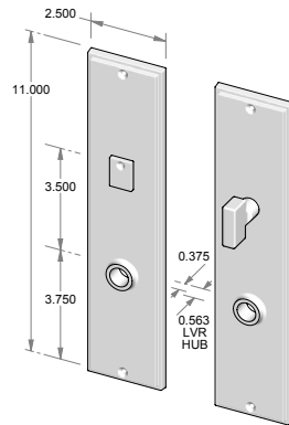
CS-2111PLMB – Complete set with passage latch, mortise bolt and spindle. OR TS-2111PLMB – Trim set only. No latch or mortise bolt. – Shown w/RC-7.
