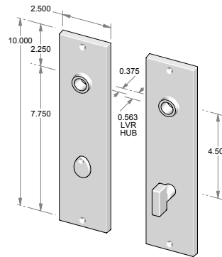
CS-F952PLMB – Complete set w/passage latch, mortise bolt & spindle. OR – TS-F952PLMB – Trim set only. No latch or mortise bolt. – Shown w/RC-9.
