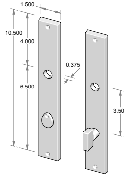
CS-F-N980PLMB – Complete set w/passage latch, mortise bolt & spindle. OR – TS-F-N980PLMB – Trim set only. No latch or mortise bolt. – Shown w/RC-9.
