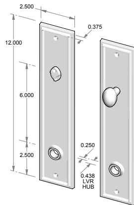
CS-423PLMB – Complete set w/passage latch, mortise bolt & spindle. OR – TS-423PLMB – Trim set only. No latch or mortise bolt. – Shown w/RC-4.
