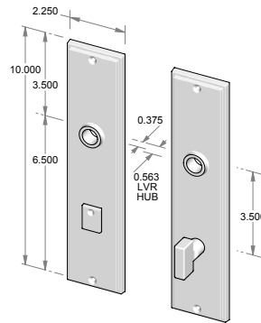
CS-F2110PLMB – Complete set with passage latch, mortise bolt and spindle. OR TS-F2110PLMB – Trim set only. No latch or mortise bolt. – Shown w/RC-7.
