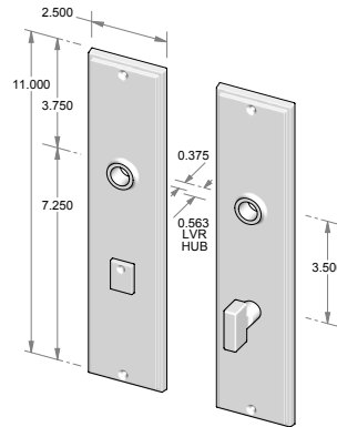
CS-F2111PLMB – Complete set with passage latch, mortise bolt and spindle. OR TS-F2111PLMB – Trim set only. No latch or mortise bolt. – Shown w/RC-7.
