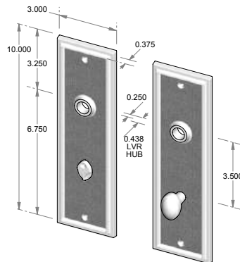
CS-F-2410PLMB – Complete set w/passage latch, mortise bolt & spindle. OR – TS-F-2410PLMB – Trim set only. No latch or mortise bolt. – Shown w/RC-4.
