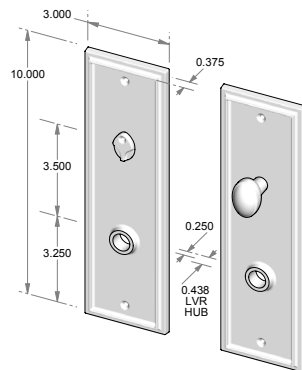
CS-422PLMB – Complete set w/passage latch, mortise bolt & spindle. OR – TS-422PLMB – Trim set only. No latch or mortise bolt. – Shown w/RC-4.
