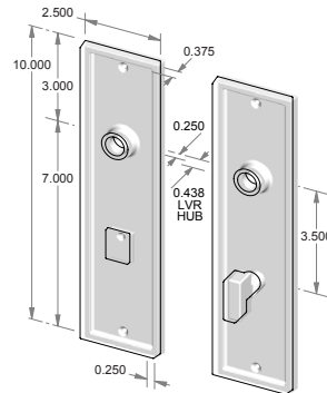
CS-F1510PLMB – Complete set with passage latch, mortise bolt and spindle. OR TS-F1510PLMB – Trim set only. No latch or mortise bolt. – Shown w/RC-7.
