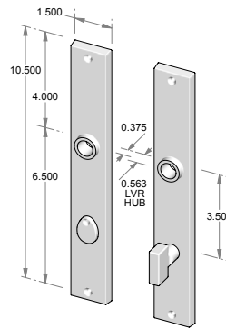
CS-F980PLMB – Complete set w/passage latch, mortise bolt & spindle. OR – TS-F980PLMB – Trim set only. No latch or mortise bolt. – Shown w/RC-9.
