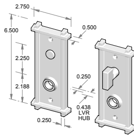
CS-355PLMB – Complete set w/passage latch, mortise bolt & spindle. OR – TS-355PLMB – Trim set only. No latch or mortise bolt.
