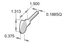
ERK-326 – Emergency release key.
