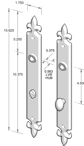
CS-F1240PLMB – Complete set with passage latch, mortise bolt and spindle. OR TS-F1240PLMB – Trim set only. No latch or mortise bolt. – Shown w/RC-4.
