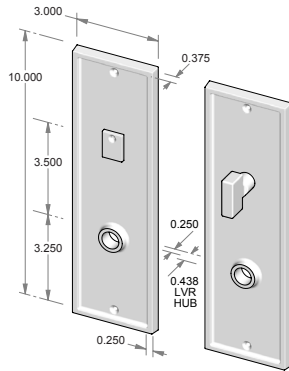
CS-1511PLMB – Complete set with passage latch, mortise bolt and spindle. OR TS-1511PLMB – Trim set only. No latch or mortise bolt. – Shown w/RC-7.
