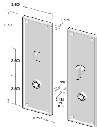
CS-1512PLMB – Complete set with passage latch, mortise bolt and spindle. OR TS-1512PLMB – Trim set only. No latch or mortise bolt. – Shown w/RC-7.
