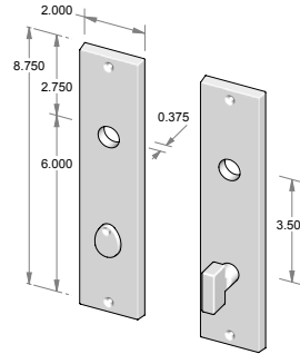
CS-F-N950PLMB – Complete set w/passage latch, mortise bolt & spindle. OR – TS-F-N950PLMB – Trim set only. No latch or mortise bolt. – Shown w/RC-9.
