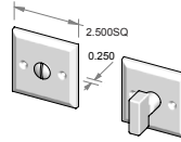
CS-CR-402MB – Complete privacy coin release set with mortise bolt. OR TS-CR-402MB – Trim set only. No latch.
