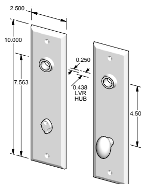
CS-F409PLMB – Complete set w/passage latch, mortise bolt & spindle. OR – TS-F409PLMB – Trim set only. No latch or mortise bolt. – Shown w/RC-4.
