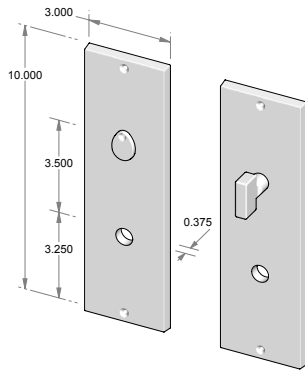
CS-N955PLMB – Complete set w/passage latch, mortise bolt & spindle. OR – TS-N955PLMB – Trim set only. No latch or mortise bolt. – Shown w/RC-9.
