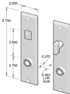
CS-2107PLMB – Complete set with passage latch, mortise bolt and spindle. OR TS-2107PLMB – Trim set only. No latch or mortise bolt. – Shown w/RC-7.
