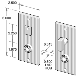
CS-1406PLMB – Complete set with passage latch, mortise bolt and spindle. OR TS-1406PLMB – Trim set only. No latch or mortise bolt. – Shown w/RC-7.
