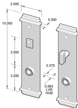
CS-440PLMB – Complete set w/passage latch, mortise bolt & spindle. OR – TS-440PLMB – Trim set only. No latch or mortise bolt. – Shown w/RC-7.
