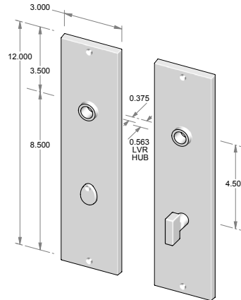
CS-F957PLMB – Complete set w/passage latch, mortise bolt & spindle. OR – TS-F957PLMB – Trim set only. No latch or mortise bolt. – Shown w/RC-9.
