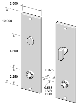
CS-952PLMB – Complete set w/passage latch, mortise bolt & spindle. OR – TS-952PLMB – Trim set only. No latch or mortise bolt. – Shown w/RC-9.
