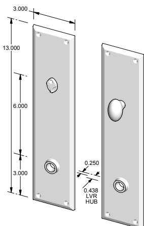
CS-601PLMB – Complete set w/passage latch, mortise bolt & spindle. OR – TS-601PLMB – Trim set only. No latch or mortise bolt. – Shown w/RC-4.
