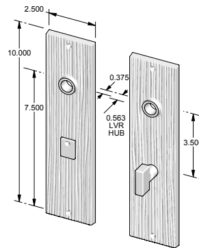
CS-F1910PLMB – Complete set with passage latch, mortise bolt and spindle. OR TS-F1910PLMB – Trim set only. No latch or mortise bolt. – Shown w/RC-7.
