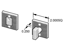
CS-22199/22200MB – Complete set with mortise bolt. OR TS-22199/22200MB – Trim set only. No latch.
