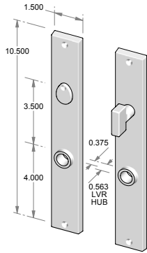
CS-980PLMB – Complete set w/passage latch, mortise bolt & spindle. OR – TS-980PLMB – Trim set only. No latch or mortise bolt. – Shown w/RC-9.
