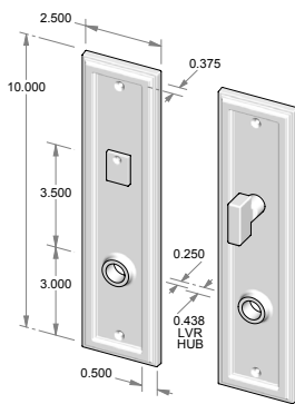
CS-2510PLMB – Complete set w/passage latch, mortise bolt & spindle. OR – TS-2510PLMB – Trim set only. No latch or mortise bolt – Shown w/RC-7.
