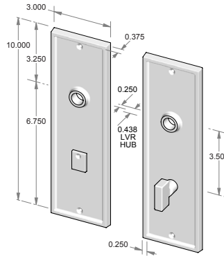
CS-F1511PLMB – Complete set with passage latch, mortise bolt and spindle. OR TS-F1511PLMB – Trim set only. No latch or mortise bolt. – Shown w/RC-7.
