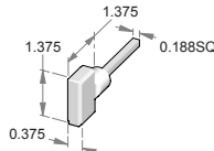
ERK-761 – Emergency release key.
