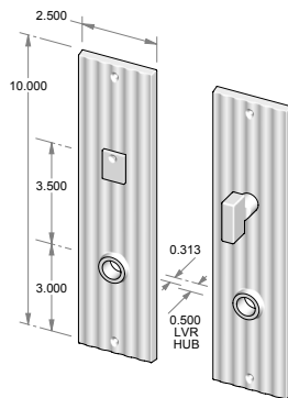
CS-1410PLMB – Complete set with passage latch, mortise bolt and spindle. OR TS-1410PLMB – Trim set only. No latch or mortise bolt. – Shown w/RC-7.
