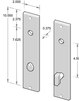
CS-F-N951PLMB – Complete set w/passage latch, mortise bolt & spindle. OR – TS-F-N951PLMB – Trim set only. No latch or mortise bolt. – Shown w/RC-9.
