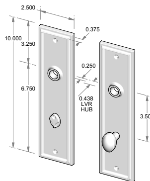
CS-F424PLMB – Complete set w/passage latch, mortise bolt & spindle. OR – TS-F424PLMB – Trim set only. No latch or mortise bolt. – Shown w/RC-4.
