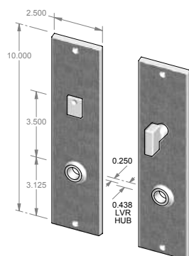
CS-2210PLMB – Complete set with passage latch, mortise bolt and spindle. OR TS-2210PLMB – Trim set only. No latch or mortise bolt. – Shown w/RC-7.
