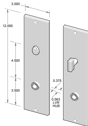
CS-957PLMB – Complete set w/passage latch, mortise bolt & spindle. OR – TS-957PLMB – Trim set only. No latch or mortise bolt. – Shown w/RC-9.
