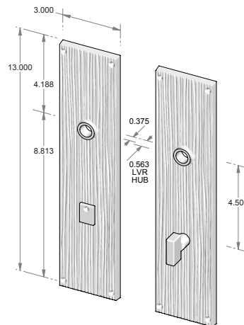
CS-F1912PLMB – Complete set with passage latch, mortise bolt and spindle. OR TS-F1912PLMB – Trim set only. No latch or mortise bolt. – Shown w/RC-7.
