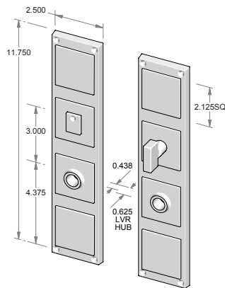
CS-1811PLMB – Complete set with passage latch, mortise bolt and spindle. OR TS-1811PLMB – Trim set only. No latch or mortise bolt. – Shown w/RC-7.
