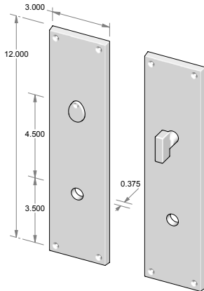
CS-N957PLMB – Complete set w/passage latch, mortise bolt & spindle. OR – TS-N957PLMB – Trim set only. No latch or mortise bolt. – Shown w/RC-9.
