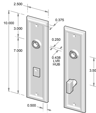
CS-F-2510PLMB – Complete set w/passage latch, mortise bolt & spindle. OR – TS-F-2510PLMB – Trim set only. No latch or mortise bolt. – Shown w/RC-7.
