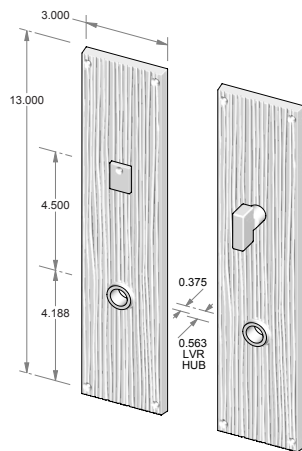
CS-1912PLMB – Complete set with passage latch, mortise bolt and spindle. OR TS-1912PLMB – Trim set only. No latch or mortise bolt. – Shown w/RC-7.
