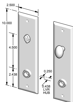
CS-409PLMB – Complete set w/passage latch, mortise bolt & spindle. OR – TS-409PLMB – Trim set only. No latch or mortise bolt. – Shown w/RC-4.
