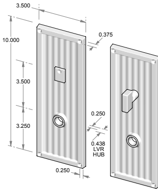
CS-431PLMB – Complete set w/passage latch, mortise bolt & spindle. OR – TS-431PLMB – Trim set only. No latch or mortise bolt. – Shown w/RC-7.
