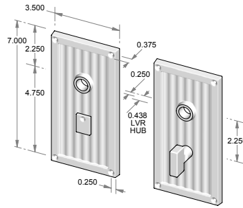
CS-F336PLMB – Complete set w/passage latch, mortise bolt & spindle. OR – TS-F336PLMB – Trim set only. No latch or mortise bolt. – Shown w/ RC-7.
