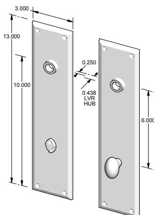
CS-F601PLMB – Complete set w/passage latch, mortise bolt & spindle. OR – TS-F601PLMB – Trim set only. No latch or mortise bolt. – Shown w/RC-4.
