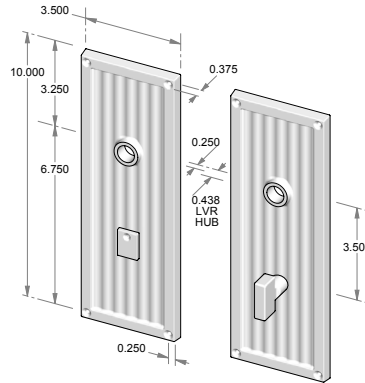
CS-F431PLMB – Complete set w/passage latch, mortise bolt & spindle. OR – TS-F431PLMB – Trim set only. No latch or mortise bolt. – Shown w/RC-7.
