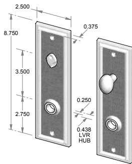
CS-2408PLMB – Complete set w/passage latch, mortise bolt & spindle. OR – TS-2408PLMB – Trim set only. No latch or mortise bolt. – Shown w/RC-4.
