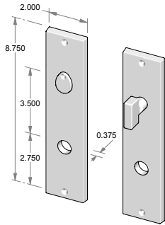
CS-N950PLMB – Complete set w/passage latch, mortise bolt & spindle. OR – TS-N950PLMB – Trim set only. No latch or mortise bolt. – Shown w/RC-9.
