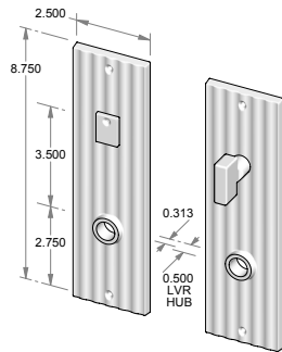
CS-1408PLMB – Complete set with passage latch, mortise bolt and spindle. OR TS-1408PLMB – Trim set only. No latch or mortise bolt. – Shown w/RC-7.
