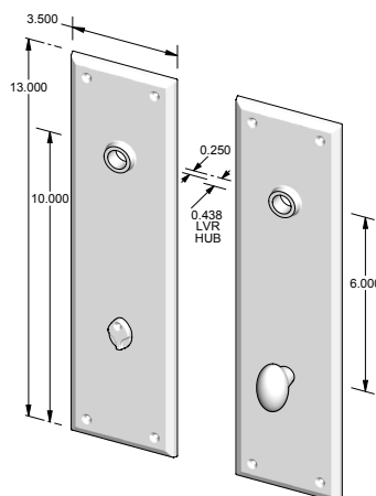
CS-F602PLMB – Complete set w/passage latch, mortise bolt & spindle. OR – TS-F602PLMB – Trim set only. No latch or mortise bolt. – Shown w/RC-4.
