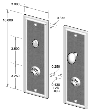
CS-2410PLMB – Complete set w/passage latch, mortise bolt & spindle. OR – TS-2410PLMB – Trim set only. No latch or mortise bolt. – Shown w/RC-4.
