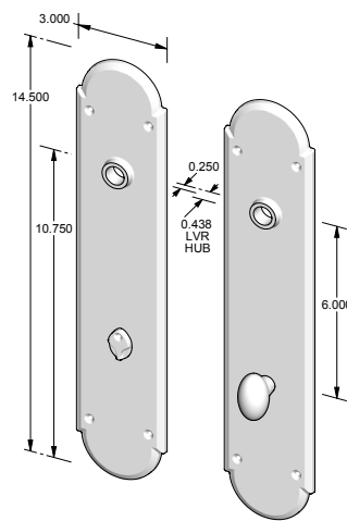
CS-F-A601PLMB – Complete set w/passage latch, mortise bolt & spindle. OR – TS-F-A601PLMB – Trim set only. No latch or mortise bolt. – Shown w/RC-4.
