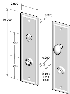
CS-424PLMB – Complete set w/passage latch, mortise bolt & spindle. OR – TS-424PLMB – Trim set only. No latch or mortise bolt. – Shown w/RC-4.
