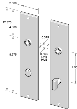
CS-F958PLMB – Complete set w/passage latch, mortise bolt & spindle. OR – TS-F958PLMB – Trim set only. No latch or mortise bolt. – Shown w/RC-9.
