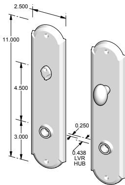
CS-A409PLMB - Complete set w/passage latch, mortise bolt & spindle. OR - TS-A409PLMB - Trim set only. No latch or mortise bolt. - Shown w/RC-4.
