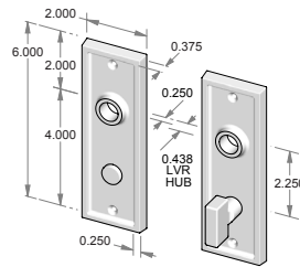
CS-F1505PLMB – Complete set with passage latch, mortise bolt and spindle. OR TS-F1505PLMB – Trim set only. No latch or mortise bolt.
