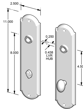
CS-F-A409PLMB - Complete set w/passage latch, mortise bolt & spindle. OR - TS-F-A409PLMB - Trim set only. No latch or mortise bolt. - Shown w/RC-4.
