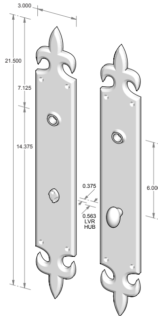
CS-F1250PLMB – Complete set with passage latch, mortise bolt and spindle. OR TS-F1250PLMB – Trim set only. No latch or mortise bolt. – Shown w/RC-4.
