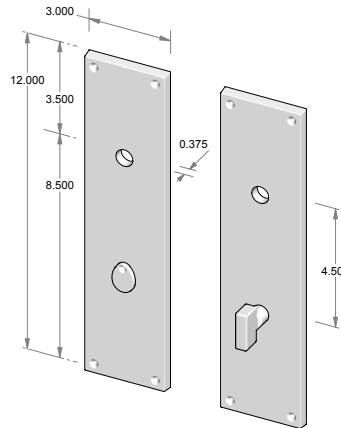
CS-F-N957PLMB – Complete set w/passage latch, mortise bolt & spindle. OR – TS-F-N957PLMB – Trim set only. No latch or mortise bolt. – Shown w/RC-9.
