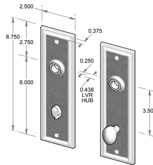
CS-F-2408PLMB – Complete set w/passage latch, mortise bolt & spindle. OR – TS-F-2408PLMB – Trim set only. No latch or mortise bolt. – Shown w/RC-4.
