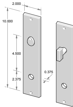
CS-N951PLMB – Complete set w/passage latch, mortise bolt & spindle. OR – TS-N951PLMB – Trim set only. No latch or mortise bolt. – Shown w/RC-9.
