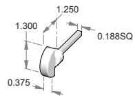
ERK-900 – Emergency release key.
