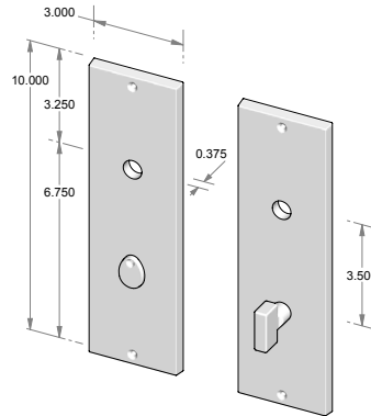
CS-F-N955PLMB – Complete set w/passage latch, mortise bolt & spindle. OR – TS-F-N955PLMB – Trim set only. No latch or mortise bolt. – Shown w/RC-9.
