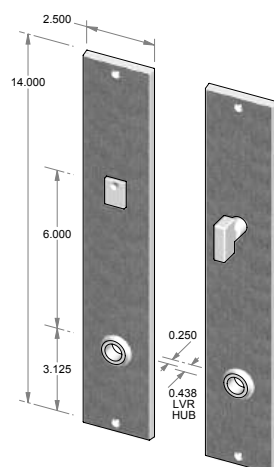
CS-2214PLMB – Complete set with passage latch, mortise bolt and spindle. OR TS-2214PLMB – Trim set only. No latch or mortise bolt. – Shown w/RC-7.
