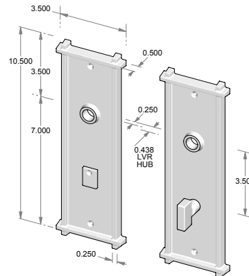
CS-F451PLMB – Complete set w/passage latch, mortise bolt & spindle. OR – TS-F451PLMB – Trim set only. No latch or mortise bolt. – Shown w/RC-7.
