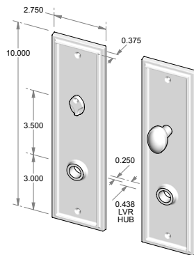
CS-426PLMB – Complete set w/passage latch, mortise bolt & spindle. OR – TS-426PLMB – Trim set only. No latch or mortise bolt. – Shown w/RC-4.
