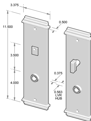
CS-441PLMB – Complete set w/passage latch, mortise bolt & spindle. OR – TS-441PLMB – Trim set only. No latch or mortise bolt. – Shown w/RC-7.
