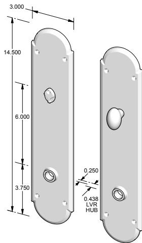
CS-A601PLMB – Complete set w/passage latch, mortise bolt & spindle. OR – TS-A601PLMB – Trim set only. No latch or mortise bolt. – Shown w/RC-4.
