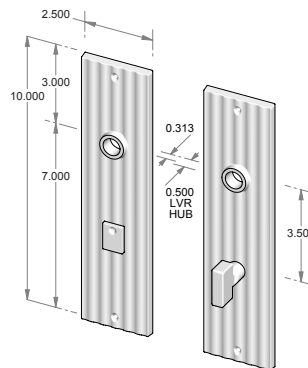
CS-F1410PLMB – Complete set with passage latch, mortise bolt and spindle. OR TS-F1410PLMB – Trim set only. No latch or mortise bolt. – Shown w/RC-7.
