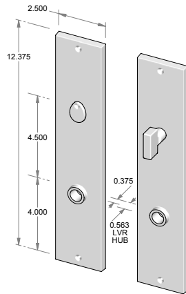
CS-958PLMB – Complete set w/passage latch, mortise bolt & spindle. OR – TS-958PLMB – Trim set only. No latch or mortise bolt. – Shown w/RC-9.
