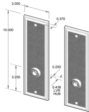
CS-2410 – Complete set with latch and spindle. OR TS-2410 – Trim set only. No latch.
