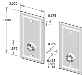
CS-326OH – Complete set with latch and spindle. OR TS-326OH – Trim set only. No latch.
