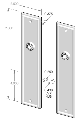
CS-F423 – Complete set with latch and spindle. OR TS-F423 – Trim set only. No latch.
