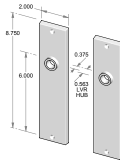
CS-F950 – Complete set with latch and spindle. OR TS-F950 – Trim set only. No latch.
