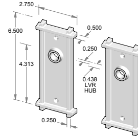
CS-F355OH – Complete set with latch and spindle. OR TS-F355OH – Trim set only. No latch.
