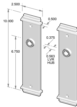
CS-F440 – Complete set with latch and spindle. OR TS-F440 – Trim set only. No latch.
