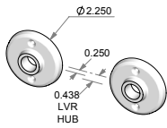
CS-RP225 – Complete set with latch and spindle. OR TS-RP225 – Trim set only. No latch.
