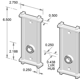
CS-355OH – Complete set with latch and spindle. OR TS-355OH – Trim set only. No latch.
