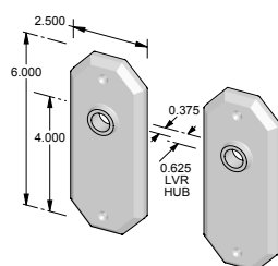
CS-F2306OH – Complete set with latch and spindle. OR TS-F2306OH – Trim set only. No latch.
