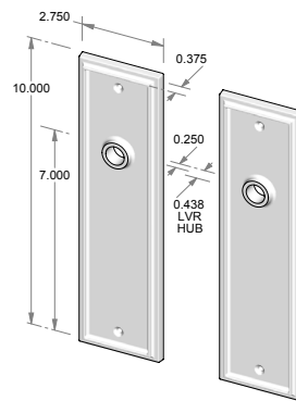
CS-F426 – Complete set with latch and spindle. OR TS-F426 – Trim set only. No latch.
