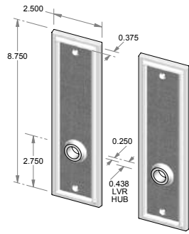
CS-2408 – Complete set with latch and spindle. OR TS-2408 – Trim set only. No latch.
