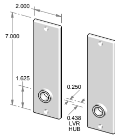
CS-E206OH – Complete set with latch and spindle. OR TS-E206OH – Trim set only. No latch.
