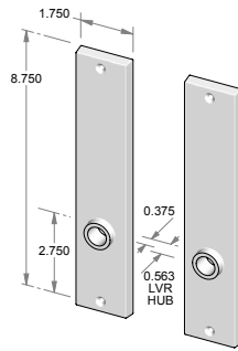
CS-959 – Complete set with latch and spindle. OR TS-959 – Trim set only. No latch.
