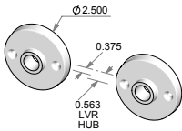
CS-RP926 – Complete set with latch and spindle. OR TS-RP926 – Trim set only. No latch.
