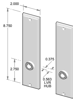
CS-2107 – Complete set with latch and spindle. OR TS-2107 – Trim set only. No latch.
