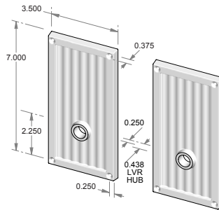
CS-336OH – Complete set with latch and spindle. OR TS-336OH – Trim set only. No latch.
