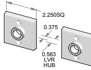
CS-925 – Complete set with latch and spindle. OR TS-925 – Trim set only. No latch.
