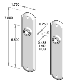
CS-F-A405OH – Complete set with latch and spindle. OR TS-F-A405OH – Trim set only. No latch.
