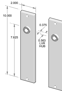
CS-F951 – Complete set with latch and spindle. OR TS-F951 – Trim set only. No latch.
