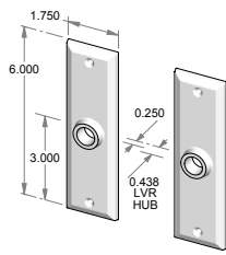
CS-405 – Complete set with latch and spindle. OR TS-405 – Trim set only. No latch.
