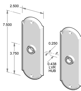
CS-A406 – Complete set with latch and spindle. OR TS-A406 – Trim set only. No latch.
