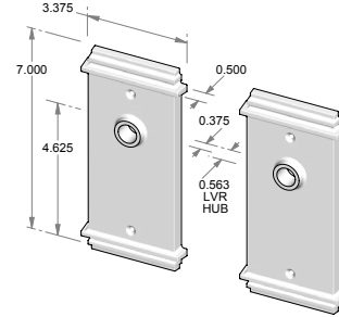
CS-F346OH – Complete set with latch and spindle. OR TS-F346OH – Trim set only. No latch.
