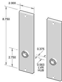
CS-950 – Complete set with latch and spindle. OR TS-950 – Trim set only. No latch.
