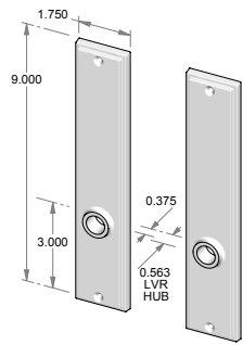
CS-2109 – Complete set with latch and spindle. OR TS-2109 – Trim set only. No latch.
