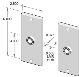
CS-954 – Complete set with latch and spindle. OR TS-954 – Trim set only. No latch.
