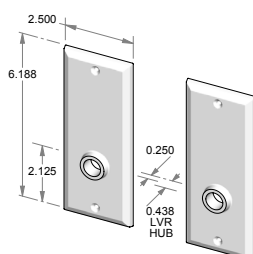
CS-406OH – Complete set with latch and spindle. OR TS-406OH – Trim set only. No latch.
