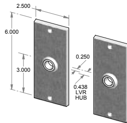
CS-2206 – Complete set with latch and spindle. OR TS-2206 – Trim set only. No latch.
