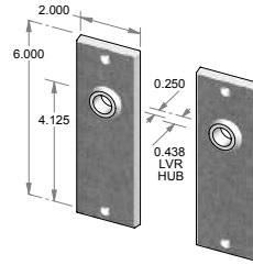
CS-F2205OH – Complete set with latch and spindle. OR TS-F2205OH – Trim set only. No latch.
