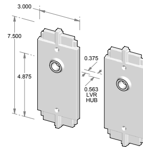
CS-F366OH – Complete set with latch and spindle. OR TS-F366OH – Trim set only. No latch.
