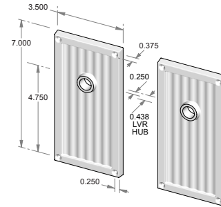
CS-F336OH – Complete set with latch and spindle. OR TS-F336OH – Trim set only. No latch.
