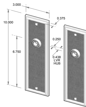
CS-F2410 – Complete set with latch and spindle. OR TS-F2410 – Trim set only. No latch.
