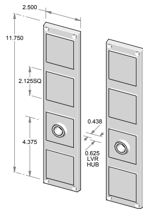
CS-1811 – Complete set with latch and spindle. OR TS-1811 – Trim set only. No latch.
