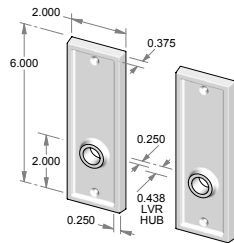
CS-1505OH – Complete set with latch and spindle. OR TS-1505OH – Trim set only. No latch.
