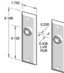
CS-F405OH – Complete set with latch and spindle. OR TS-F405OH – Trim set only. No latch.
