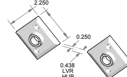
CS-225DI – Complete set with latch and spindle. OR TS-225DI – Trim set only. No latch.
