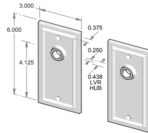
CS-F326OH – Complete set with latch and spindle. OR TS-F326OH – Trim set only. No latch.
