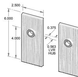
CS-F1906OH – Complete set with latch and spindle. OR TS-F1906OH – Trim set only. No latch.
