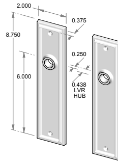
CS-F420 – Complete set with latch and spindle. OR TS-F420 – Trim set only. No latch.
