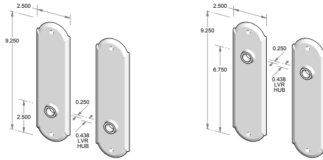
CS-A408 – Complete set with latch and spindle. OR TS-A408 – Trim set only. No latch.
