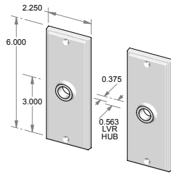
CS-2106 – Complete set with latch and spindle. OR TS-2106 – Trim set only. No latch.
