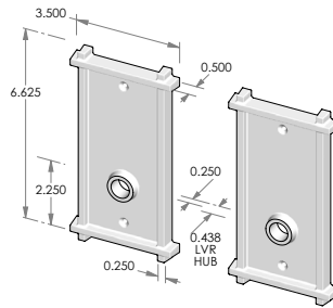
CS-356OH – Complete set with latch and spindle. OR TS-356OH – Trim set only. No latch.
