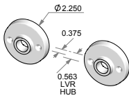
CS-RP925 – Complete set with latch and spindle. OR TS-RP925 – Trim set only. No latch.
