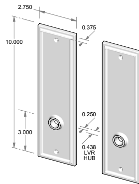
CS-426 – Complete set with latch and spindle. OR TS-426 – Trim set only. No latch.
