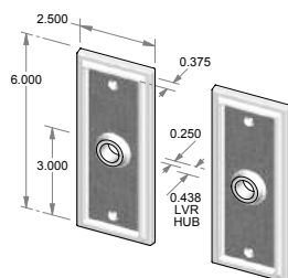
CS-2406 – Complete set with latch and spindle. OR TS-2406 – Trim set only. No latch.
