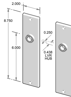
CS-F-E407 – Complete set with latch and spindle. OR TS-F-E407 – Trim set only. No latch.
