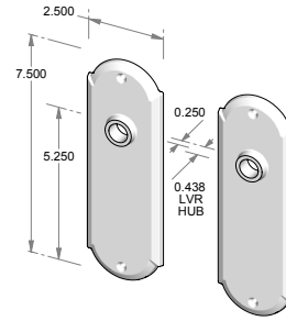
CS-F-A406OH – Complete set with latch and spindle. OR TS-F-A406OH – Trim set only. No latch.
