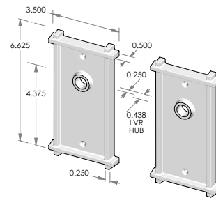
CS-F356OH – Complete set with latch and spindle. OR TS-F356OH – Trim set only. No latch.
