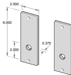
CS-N949OH – Complete set with latch and spindle. OR TS-N949OH – Trim set only. No latch.
