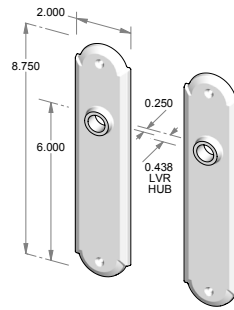
CS-F-A407 – Complete set with latch and spindle. OR TS-F-A407 – Trim set only. No latch.
