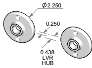
CS-RP-E225 – Complete set with latch and spindle. OR TS-RP-E225 – Trim set only. No latch.
