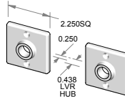
CS-E225 – Complete set with latch and spindle. OR TS-E225 – Trim set only. No latch.
