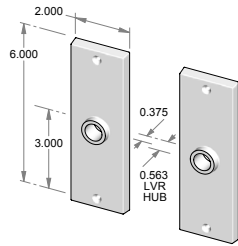
CS-949 – Complete set with latch and spindle. OR TS-949 – Trim set only. No latch.
