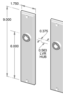
CS-F2109 – Complete set with latch and spindle. OR TS-F2109 – Trim set only. No latch.
