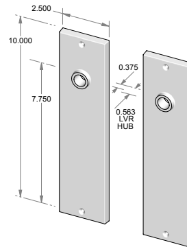
CS-F952 – Complete set with latch and spindle. OR TS-F952 – Trim set only. No latch.
