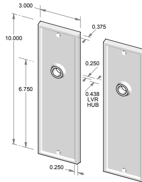
CS-F1511 – Complete set with latch and spindle. OR TS-F1511 – Trim set only. No latch.
