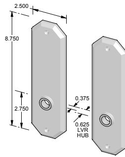
CS-2308 – Complete set with latch and spindle. OR TS-2308 – Trim set only. No latch.
