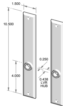
CS-811 – Complete set with latch and spindle. OR TS-811 – Trim set only. No latch.
