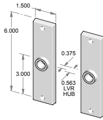
CS-979 – Complete set with latch and spindle. OR TS-979 – Trim set only. No latch.
