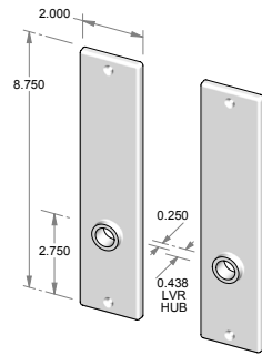
CS-E407 – Complete set with latch and spindle. OR TS-E407 – Trim set only. No latch.
