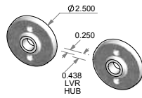
CS-RP2200 – Complete set with latch and spindle. OR TS-RP2200 – Trim set only. No latch.
