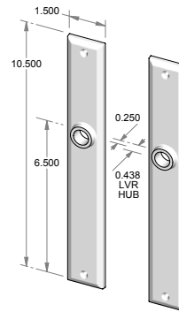
CS-F811 – Complete set with latch and spindle. OR TS-F811 – Trim set only. No latch.
