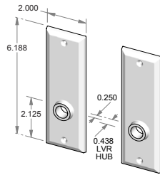
CS-206OH – Complete set with latch and spindle. OR TS-206OH – Trim set only. No latch.
