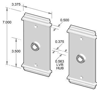
CS-346 – Complete set with latch and spindle. OR TS-346 – Trim set only. No latch.
