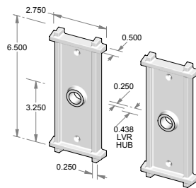
CS-355 – Complete set with latch and spindle. OR TS-355 – Trim set only. No latch.
