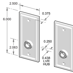
CS-325OH – Complete set with latch and spindle. OR TS-325OH – Trim set only. No latch.
