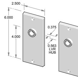
CS-F954OH – Complete set with latch and spindle. OR TS-F954OH – Trim set only. No latch.
