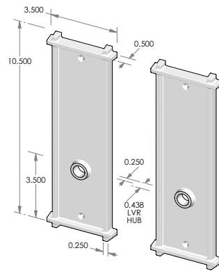
CS-451 – Complete set with latch and spindle. OR TS-451 – Trim set only. No latch.
