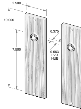
CS-F1910 – Complete set with latch and spindle. OR TS-F1910 – Trim set only. No latch.
