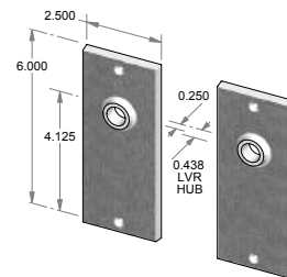
CS-F2206OH – Complete set with latch and spindle. OR TS-F2206OH – Trim set only. No latch.
