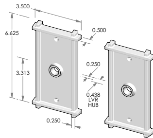
CS-356 – Complete set with latch and spindle. OR TS-356 – Trim set only. No latch.
