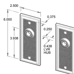
CS-F2406OH – Complete set with latch and spindle. OR TS-F2406OH – Trim set only. No latch.
