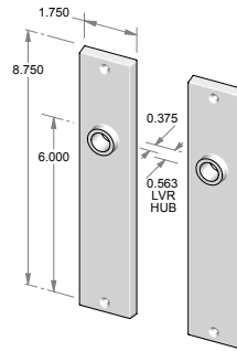
CS-F959 – Complete set with latch and spindle. OR TS-F959 – Trim set only. No latch.
