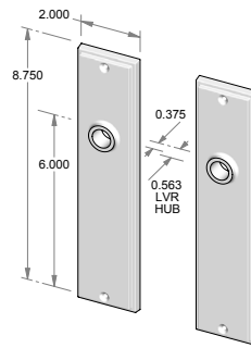
CS-F2107 – Complete set with latch and spindle. OR TS-F2107 – Trim set only. No latch.
