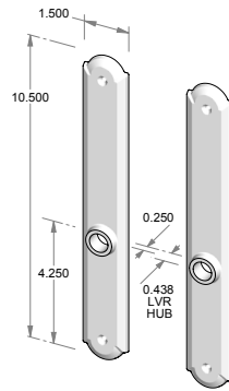
CS-A811 – Complete set with latch and spindle. OR TS-A811 – Trim set only. No latch.
