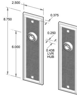
CS-F2408 – Complete set with latch and spindle. OR TS-F2408 – Trim set only. No latch.
