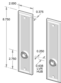
CS-420 – Complete set with latch and spindle. OR TS-420 – Trim set only. No latch.
