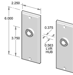
CS-F2106OH – Complete set with latch and spindle. OR TS-F2106OH – Trim set only. No latch.
