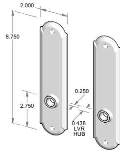
CS-A407 – Complete set with latch and spindle. OR TS-A407 – Trim set only. No latch.
