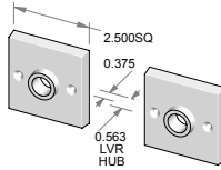
CS-926 – Complete set with latch and spindle. OR TS-926 – Trim set only. No latch.
