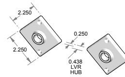
CS-E225DI – Complete set with latch and spindle. OR TS-E225DI – Trim set only. No latch.
