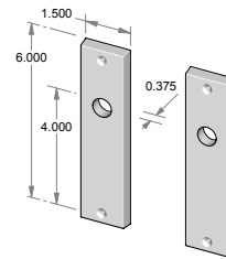
CS-F-N979OH – Complete set with latch and spindle. OR TS-F-N979OH – Trim set only. No latch.
