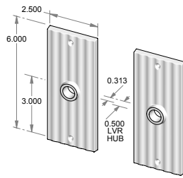
CS-1406 – Complete set with latch and spindle. OR TS-1406 – Trim set only. No latch.
