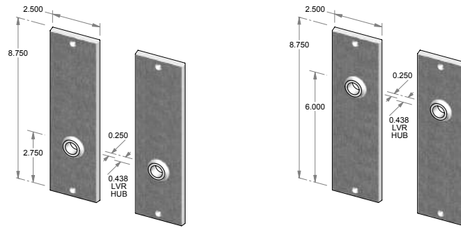
CS-2208 – Complete set with latch and spindle. OR TS-2208 – Trim set only. No latch.
