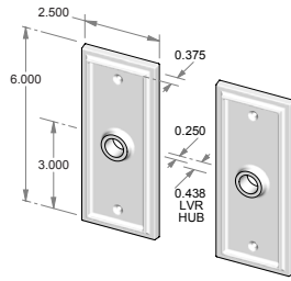
CS-325 – Complete set with latch and spindle. OR TS-325 – Trim set only. No latch.
