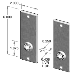
CS-2205OH – Complete set with latch and spindle. OR TS-2205OH – Trim set only. No latch.
