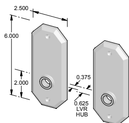
CS-2306OH – Complete set with latch and spindle. OR TS-2306OH – Trim set only. No latch.
