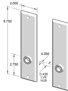
CS-407 – Complete set with latch and spindle. OR TS-407 – Trim set only. No latch.
