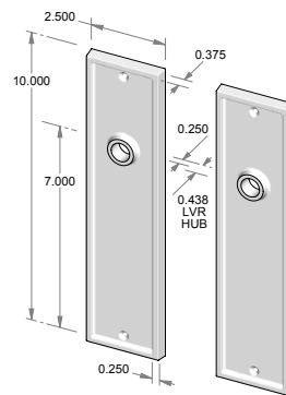
CS-F1510 – Complete set with latch and spindle. OR TS-F1510 – Trim set only. No latch.
