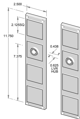
CS-F1811 – Complete set with latch and spindle. OR TS-F1811 – Trim set only. No latch.
