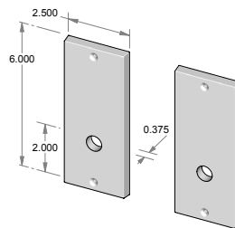
CS-N954OH – Complete set with latch and spindle. OR TS-N954OH – Trim set only. No latch.
