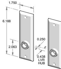
CS-405OH – Complete set with latch and spindle. OR TS-405OH – Trim set only. No latch.
