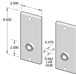
CS-954OH – Complete set with latch and spindle. OR TS-954OH – Trim set only. No latch.
