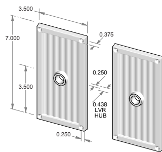
CS-336 – Complete set with latch and spindle. OR TS-336 – Trim set only. No latch.
