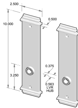
CS-440 – Complete set with latch and spindle. OR TS-440 – Trim set only. No latch.
