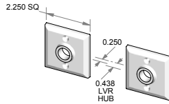
CS-225 – Complete set with latch and spindle. OR TS-225 – Trim set only. No latch.
