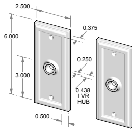
CS-2506 – Complete set with latch and spindle. OR TS-2506 – Trim set only. No latch.
