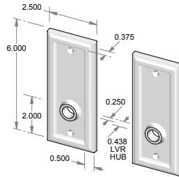
CS-2506OH – Complete set with latch and spindle. OR TS-2506OH – Trim set only. No latch.
