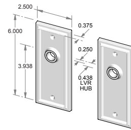
CS-F325OH – Complete set with latch and spindle. OR TS-F325OH – Trim set only. No latch.
