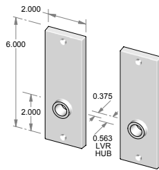
CS-949OH – Complete set with latch and spindle. OR TS-949OH – Trim set only. No latch.
