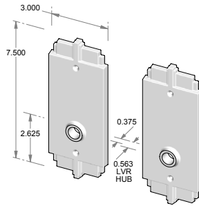
CS-366OH – Complete set with latch and spindle. OR TS-366OH – Trim set only. No latch.
