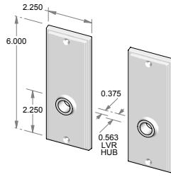
CS-2106OH – Complete set with latch and spindle. OR TS-2106OH – Trim set only. No latch.
