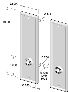
CS-1510 – Complete set with latch and spindle. OR TS-1510 – Trim set only. No latch.
