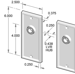
CS-F1506OH – Complete set with latch and spindle. OR TS-F1506OH – Trim set only. No latch.
