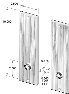
CS-1910 – Complete set with latch and spindle. OR TS-1910 – Trim set only. No latch.
