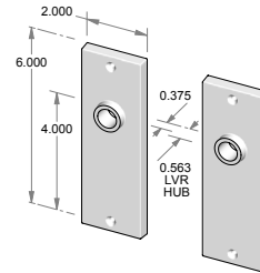
CS-F949OH – Complete set with latch and spindle. OR TS-F949OH – Trim set only. No latch.
