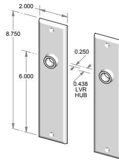
CS-F407 – Complete set with latch and spindle. OR TS-F407 – Trim set only. No latch.
