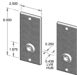
CS-2206OH – Complete set with latch and spindle. OR TS-2206OH – Trim set only. No latch.
