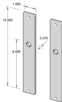
CS-N980 – Complete set with latch and spindle. OR TS-N980 – Trim set only. No latch.
