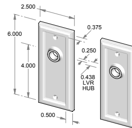
CS-F2506OH – Complete set with latch and spindle. OR TS-F2506OH – Trim set only. No latch.
