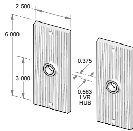
CS-1906 – Complete set with latch and spindle. OR TS-1906 – Trim set only. No latch.
