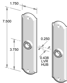
CS-A405 – Complete set with latch and spindle. OR TS-A405 – Trim set only. No latch.
