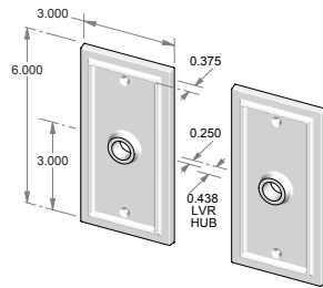
CS-326 – Complete set with latch and spindle. OR TS-326 – Trim set only. No latch.
