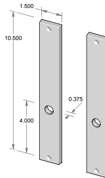
CS-F-N980 – Complete set with latch and spindle. OR TS-F-N980 – Trim set only. No latch.
