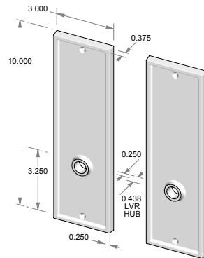
CS-1511 – Complete set with latch and spindle. OR TS-1511 – Trim set only. No latch.
