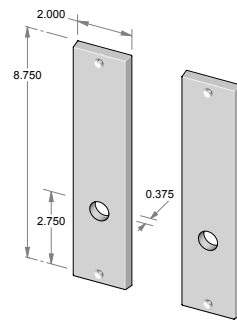
CS-N950 – Complete set with latch and spindle. OR TS-N950 – Trim set only. No latch.
