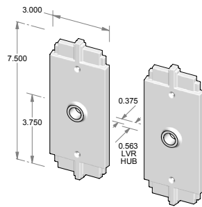
CS-366 – Complete set with latch and spindle. OR TS-366 – Trim set only. No latch.
