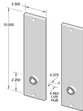
CS-952 – Complete set with latch and spindle. OR TS-952 – Trim set only. No latch.
