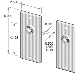
CS-F1406OH – Complete set with latch and spindle. OR TS-F1406OH – Trim set only. No latch.
