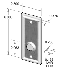
TS-2406IML-HD – Trim set only. – Full dummy.
