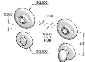
CS-F-RP402-8xRP200IML-PR – Complete privacy set with interior mortise lock and spindle. OR TS-F-RP402-8xRP200IML-PR – Trim set only. No lock.
