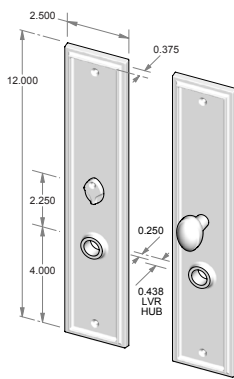
CS-423IML-PR – Complete privacy set with interior mortise lock and spindle. OR TS-423IML-PR – Trim set only. No lock.
