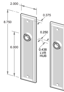
TS-F420IML-FD – Trim set only. – Full dummy.
