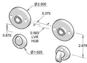
CS-F-RP926-8xRP9158IML-PR – Complete privacy set with interior mortise lock and spindle. OR TS-F-RP926-8xRP9158IML-PR – Trim set only. No lock.
