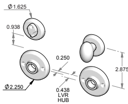
CS-RP225-8xRP158IML-PR – Complete privacy set with interior mortise lock and spindle. OR TS-RP225-8xRP158IML-PR – Trim set only. No lock.
