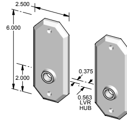
TS-2306IML-FD – Trim set only. – Full dummy.
