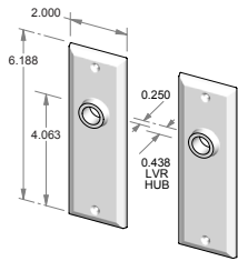
CS-F206IML – Complete passage set with interior mortise lock and spindle. OR TS-F206IML – Trim set only. No lock.
