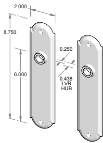
CS-F-A407IML – Complete passage set with interior mortise lock and spindle. OR TS-F-A407IML – Trim set only. No lock.
