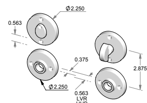
CS-RP925-8xRP9225IML-PR – Complete privacy set with interior mortise lock and spindle. OR TS-RP925-8xRP9225IML-PR – Trim set only. No lock.
