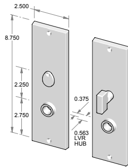
CS-953IML-PR – Complete privacy set with interior mortise lock and spindle. OR TS-953IML-PR – Trim set only. No lock.
