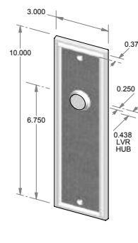
TS-F2410IML-HD – Trim set only. – Full dummy.
