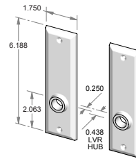
TS-405IML-FD – Trim set only. – Full dummy.
