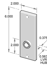
TS-926IML-HD – Trim set only. – Half dummy.
