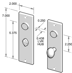
CS-F-E206IML-PR – Complete privacy set with interior mortise lock and spindle. OR TS-F-E206IML-PR – Trim set only. No lock.
