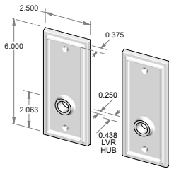
CS-325IML – Complete passage set with interior mortise lock and spindle. OR TS-325IML – Trim set only. No lock.
