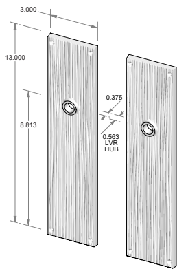
CS-F1912IML – Complete passage set with interior mortise lock and spindle. OR TS-F1912IML – Trim set only. No lock.
