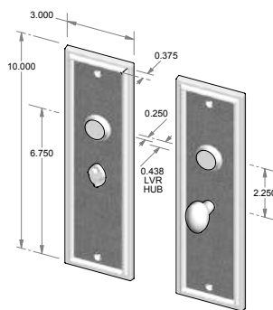
CS-F2410IML-PR – Complete privacy set with interior mortise lock and spindle. OR TS-F2410IML-PR – Trim set only. No lock.
