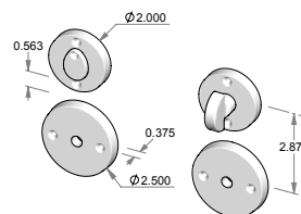
CS-RP-N926-8xRP9200IML-PR – Complete privacy set with interior mortise lock and spindle. OR TS-RP-N926-8xRP9200IML-PR – Trim set only. No lock.
