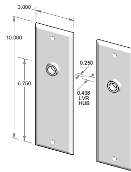
TS-F410IML-FD – Trim set only. – Full dummy.
