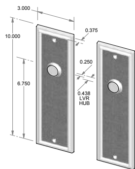
CS-F2410IML – Complete passage set with interior mortise lock and spindle. OR TS-F2410IML – Trim set only. No lock.
