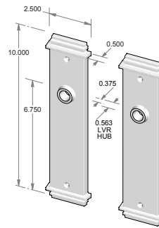
TS-F440IML-FD – Trim set only. – Full dummy.
