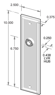
TS-F424IML-HD – Trim set only. – Full dummy.
