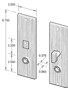
CS-1908IML-PR – Complete privacy set with interior mortise lock and spindle. OR TS-1908IML-PR – Trim set only. No lock.
