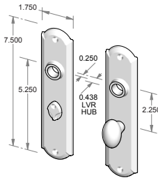
CS-F-A405IML-PR – Complete privacy set with interior mortise lock and spindle. OR TS-F-A405IML-PR – Trim set only. No lock.
