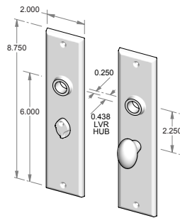
CS-F407IML-PR – Complete privacy set with interior mortise lock and spindle. OR TS-F407IML-PR – Trim set only. No lock.
