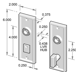
CS-F1505IML-PR – Complete privacy set with interior mortise lock and spindle. OR TS-F1505IML-PR – Trim set only. No lock.
