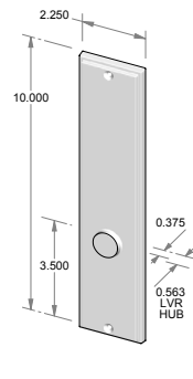
TS-2110IML-HD – Trim set only. – Full dummy.
