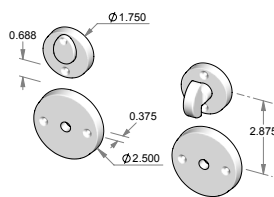
CS-RP-N926-8xRP9175IML-PR – Complete privacy set with interior mortise lock and spindle. OR TS-RP-N926-8xRP9175IML-PR – Trim set only. No lock.
