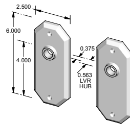
TS-F2306IML-FD – Trim set only. – Full dummy.
