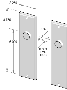
TS-F2108IML-FD – Trim set only. – Full dummy.
