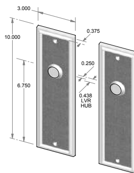
TS-F2410IML-FD – Trim set only. – Full dummy.
