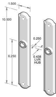
CS-F-A811IML – Complete passage set with interior mortise lock and spindle. OR TS-F-A811IML – Trim set only. No lock.
