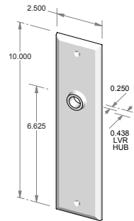
TS-F409IML-HD – Trim set only. – Full dummy.
