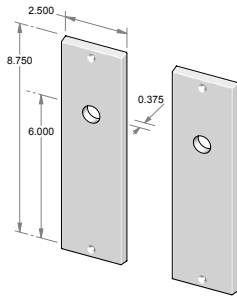
CS-F-N953IML – Complete passage set with interior mortise lock and spindle. OR TS-F-N953IML – Trim set only. No lock.
