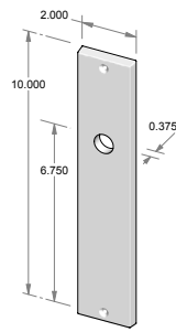
TS-F-N951IML-HD – Trim set only. – Full dummy.
