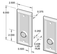
TS-2506IML-FD – Trim set only. – Full dummy.
