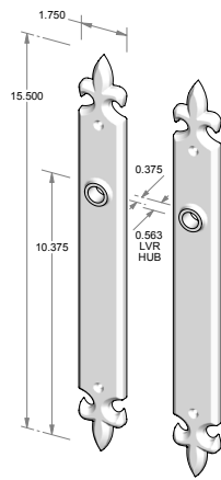
CS-F1240IML – Complete passage set with interior mortise lock and spindle. OR TS-F1240IML – Trim set only. No lock.
