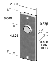
TS-F2205IML-HD – Trim set only. – Full dummy.
