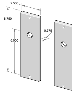
TS-F-N953IML-FD – Trim set only. – Full dummy.
