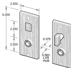
CS-1906IML-PR – Complete privacy set with interior mortise lock and spindle. OR TS-1906IML-PR – Trim set only. No lock.
