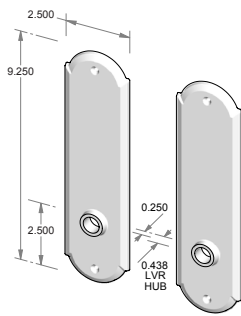
CS-A408IML – Complete passage set with interior mortise lock and spindle. OR TS-A408IML – Trim set only. No lock.
