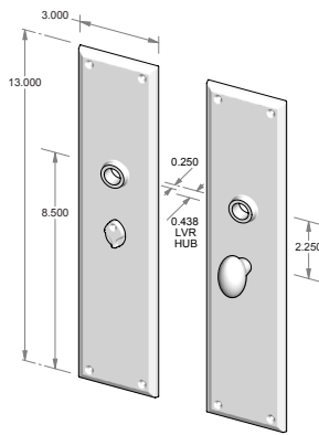
CS-F601IML-PR – Complete privacy set with interior mortise lock and spindle. OR TS-F601IML-PR – Trim set only. No lock.
