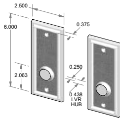
CS-2406IML – Complete passage set with interior mortise lock and spindle. OR TS-2406IML – Trim set only. No lock.
