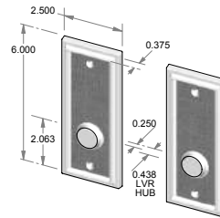
TS-2406IML-FD – Trim set only. – Full dummy.
