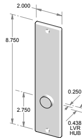
TS-E407IML-HD – Trim set only. – Full dummy.
