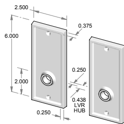
CS-1506IML – Complete passage set with interior mortise lock and spindle. OR TS-1506IML – Trim set only. No lock.
