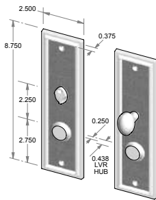
CS-2408IML-PR – Complete privacy set with interior mortise lock and spindle. OR TS-2408IML-PR – Trim set only. No lock.
