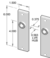
TS-F979IML-FD – Trim set only. – Full dummy.
