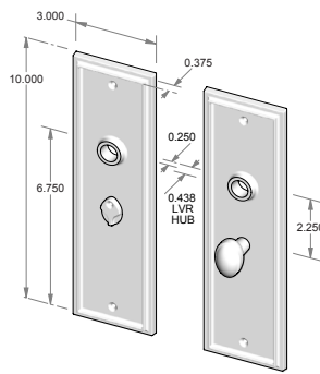
CS-F422IML-PR – Complete privacy set with interior mortise lock and spindle. OR TS-F422IML-PR – Trim set only. No lock.
