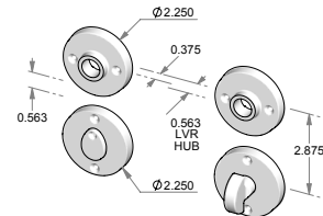
CS-F-RP925-8xRP9225IML-PR – Complete privacy set with interior mortise lock and spindle. OR TS-F-RP925-8xRP9225IML-PR – Trim set only. No lock.
