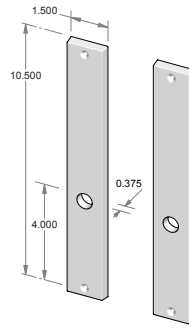
TS-N980IML-FD – Trim set only. – Full dummy.
