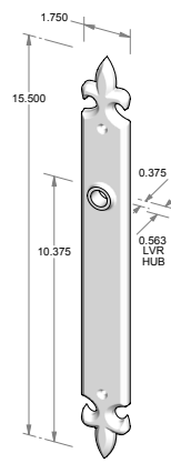
TS-F1240IML-HD – Trim set only. – Full dummy.
