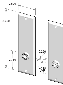
TS-408IML-FD – Trim set only. – Full dummy.
