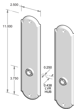
CS-A409IML – Complete passage set with interior mortise lock and spindle. OR TS-A409IML – Trim set only. No lock.
