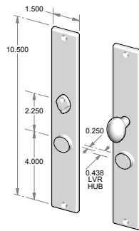
CS-E811IML-PR – Complete privacy set with interior mortise lock and spindle. OR TS-E811IML-PR – Trim set only. No lock.
