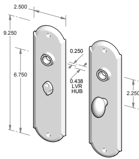
CS-F-A408IML-PR – Complete privacy set with interior mortise lock and spindle. OR TS-F-A408IML-PR – Trim set only. No lock.
