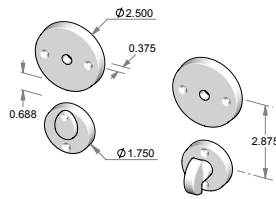
CS-F-RP-N926-8xRP9175IML-PR – Complete privacy set with interior mortise lock and spindle. OR TS-F-RP-N926-8xRP9175IML-PR – Trim set only. No lock.
