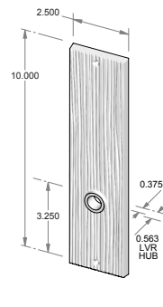
TS-1910IML-HD – Trim set only. – Full dummy.
