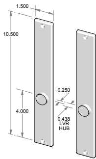
CS-E811IML – Complete passage set with interior mortise lock and spindle. OR TS-E811IML – Trim set only. No lock.
