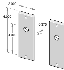
TS-F-N949IML-FD – Trim set only. – Full dummy.
