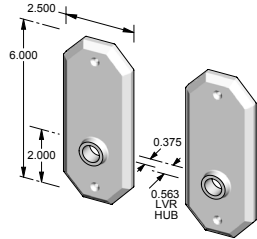
CS-2306IML – Complete passage set with interior mortise lock and spindle. OR TS-2306IML – Trim set only. No lock.
