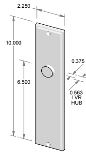
TS-F2110IML-HD – Trim set only. – Full dummy.
