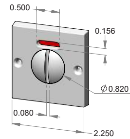
CR-1-INDICATOR Coin release w/ indicator.
