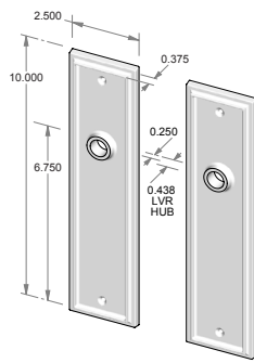
CS-F424IML – Complete passage set with interior mortise lock and spindle. OR TS-F424IML – Trim set only. No lock.
