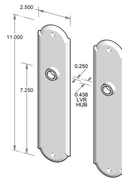
TS-F-A409IML-FD – Trim set only. – Full dummy.
