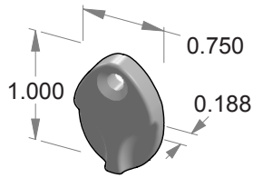
RC-4 Original teardrop release cover.
