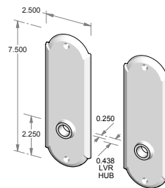
TS-A406IML-FD – Trim set only. – Full dummy.
