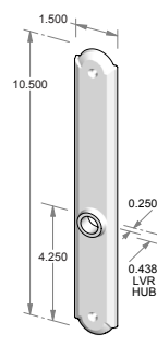
TS-A811IML-HD – Trim set only. – Full dummy.
