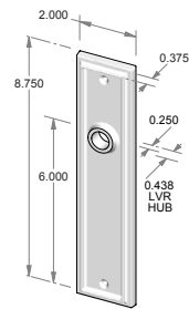
TS-F420IML-HD – Trim set only. – Full dummy.
