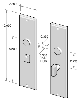
CS-F2110IML-PR – Complete privacy set with interior mortise lock and spindle. OR TS-F2110IML-PR – Trim set only. No lock.
