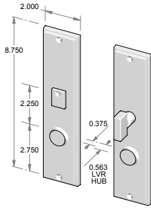
CS-2107IML-PR – Complete privacy set with interior mortise lock and spindle. OR TS-2107IML-PR – Trim set only. No lock.
