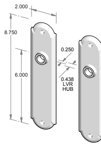
TS-F-A407IML-FD – Trim set only. – Full dummy.
