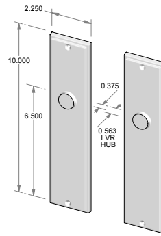
TS-F2110IML-FD – Trim set only. – Full dummy.
