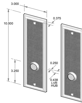
TS-2410IML-FD – Trim set only. – Full dummy.
