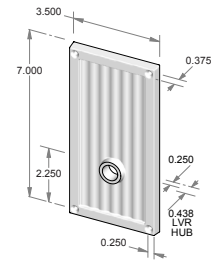
TS-336IML-HD – Trim set only. – Full dummy.
