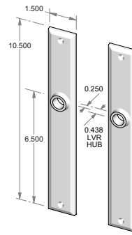
TS-F811IML-FD – Trim set only. – Full dummy.
