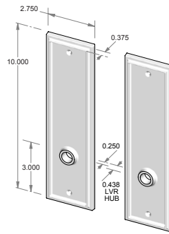
TS-426IML-FD – Trim set only. – Full dummy.
