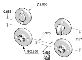
CS-RP925-8xRP9200IML-PR – Complete privacy set with interior mortise lock and spindle. OR TS-RP925-8xRP9200IML-PR – Trim set only. No lock.
