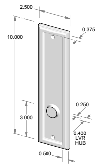
TS-2510IML-HD – Trim set only. – Full dummy.
