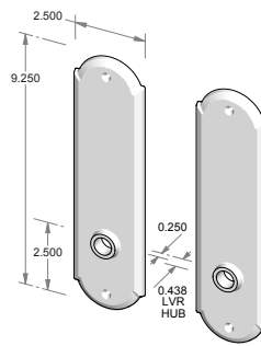
TS-A408IML-FD – Trim set only. – Full dummy.
