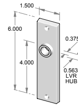
TS-F979IML-HD – Trim set only. – Half dummy.
