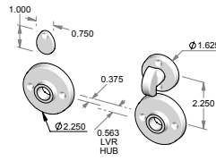
CS-RP925IML-PR-RC – Complete privacy set with interior mortise lock and spindle. OR TS-RP925IML-PR-RC – Trim set only. No lock.
