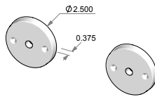
CS-RP-N926-8IML – Complete passage set with interior mortise lock and spindle. OR TS-RP-N926-8IML – Trim set only. No lock.
