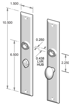
CS-F811IML-PR – Complete privacy set with interior mortise lock and spindle. OR TS-F811IML-PR – Trim set only. No lock.
