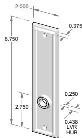
TS-420IML-HD – Trim set only. – Full dummy.
