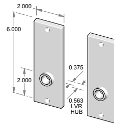
TS-949IML-FD – Trim set only. – Full dummy.
