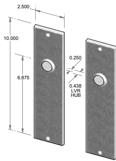
CS-F2210IML – Complete passage set with interior mortise lock and spindle. OR TS-F2210IML – Trim set only. No lock.
