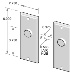
TS-F2106IML-FD – Trim set only. – Full dummy.
