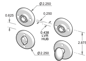
CS-F-RP225-8xRP225IML-PR – Complete privacy set with interior mortise lock and spindle. OR TS-F-RP225-8xRP225IML-PR – Trim set only. No lock.
