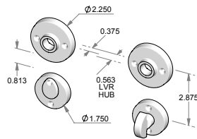
CS-F-RP925-8xRP9175IML-PR – Complete privacy set with interior mortise lock and spindle. OR TS-F-RP925-8xRP9175IML-PR – Trim set only. No lock.
