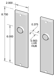
CS-F2107IML – Complete passage set with interior mortise lock and spindle. OR TS-F2107IML – Trim set only. No lock.
