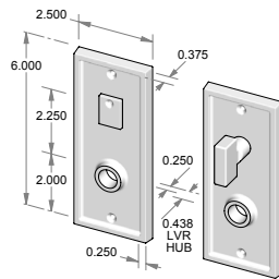
CS-1506IML-PR – Complete privacy set with interior mortise lock and spindle. OR TS-1506IML-PR – Trim set only. No lock.
