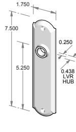
TS-F-A405IML-HD – Trim set only. – Full dummy.
