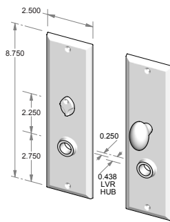
CS-408IML-PR – Complete privacy set with interior mortise lock and spindle. OR TS-408IML-PR – Trim set only. No lock.
