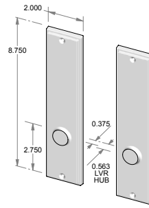
TS-2107IML-FD – Trim set only. – Full dummy.
