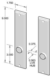
CS-2109IML – Complete passage set with interior mortise lock and spindle. OR TS-2109IML – Trim set only. No lock.
