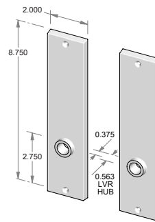
TS-950IML-FD – Trim set only. – Full dummy.
