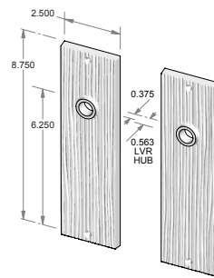
TS-F1908IML-FD – Trim set only. – Full dummy.
