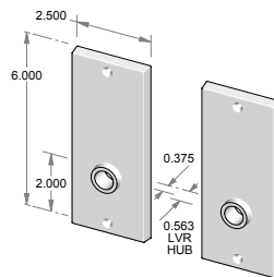
TS-954IML-FD – Trim set only. – Full dummy.
