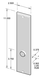
TS-2111IML-HD – Trim set only. – Full dummy.
