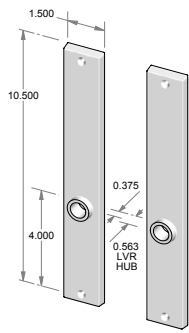
CS-980IML – Complete passage set with interior mortise lock and spindle. OR TS-980IML – Trim set only. No lock.
