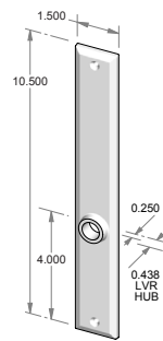
TS-811IML-HD – Trim set only. – Full dummy.
