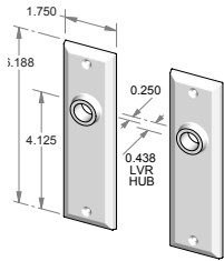
CS-F405IML – Complete passage set with interior mortise lock and spindle. OR TS-F405IML – Trim set only. No lock.
