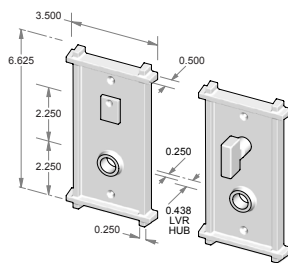
CS-356IML-PR – Complete privacy set with interior mortise lock and spindle. OR TS-356IML-PR – Trim set only. No lock.
