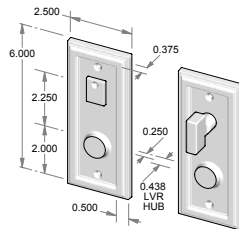
CS-2506IML-PR – Complete privacy set with interior mortise lock and spindle. OR TS-2506IML-PR – Trim set only. No lock.
