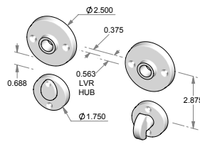
CS-F-RP926-8xRP9175IML-PR – Complete privacy set with interior mortise lock and spindle. OR TS-F-RP926-8xRP9175IML-PR – Trim set only. No lock.
