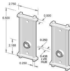
CS-355IML – Complete passage set with interior mortise lock and spindle. OR TS-355IML – Trim set only. No lock.
