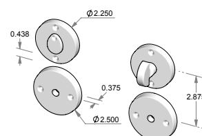
CS-RP-N926-8xRP9225IML-PR – Complete privacy set with interior mortise lock and spindle. OR TS-RP-N926-8xRP9225IML-PR – Trim set only. No lock.
