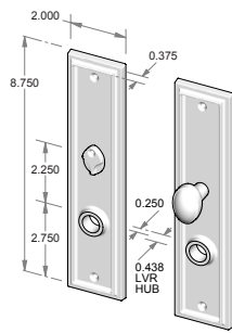
CS-420IML-PR – Complete privacy set with interior mortise lock and spindle. OR TS-420IML-PR – Trim set only. No lock.
