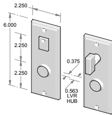
CS-2106IML-PR – Complete privacy set with interior mortise lock and spindle. OR TS-2106IML-PR – Trim set only. No lock.
