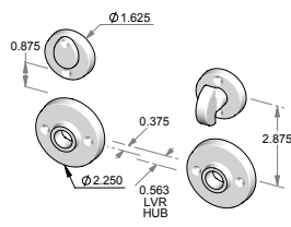
CS-RP925-8xRP9158IML-PR – Complete privacy set with interior mortise lock and spindle. OR TS-RP925-8xRP9158IML-PR – Trim set only. No lock.
