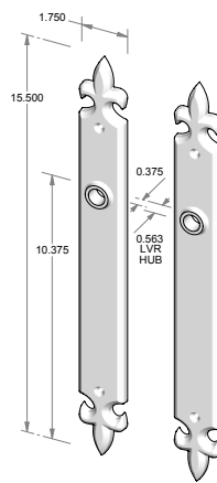
TS-F1240IML-FD – Trim set only. – Full dummy.
