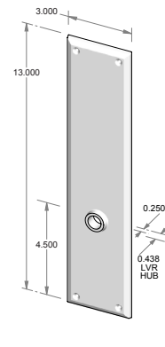
TS-601IML-HD – Trim set only. – Full dummy.
