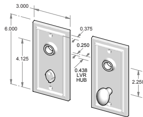
CS-F326IML-PR – Complete privacy set with interior mortise lock and spindle. OR TS-F326IML-PR – Trim set only. No lock.
