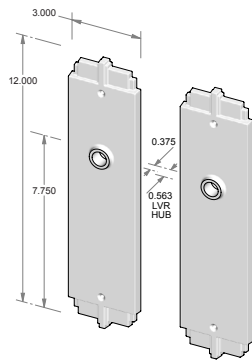
CS-F461IML – Complete passage set with interior mortise lock and spindle. OR TS-F461IML – Trim set only. No lock.
