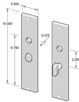
CS-F-N951IML-PR – Complete privacy set with interior mortise lock and spindle. OR TS-F-N951IML-PR – Trim set only. No lock.
