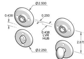
CS-F-RP402-8xRP225IML-PR – Complete privacy set with interior mortise lock and spindle. OR TS-F-RP402-8xRP225IML-PR – Trim set only. No lock.
