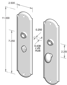
CS-F-A409IML-PR – Complete privacy set with interior mortise lock and spindle. OR TS-F-A409IML-PR – Trim set only. No lock.
