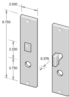
CS-N950IML-PR – Complete privacy set with interior mortise lock and spindle. OR TS-N950IML-PR – Trim set only. No lock.
