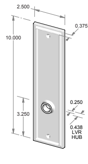
TS-424IML-HD – Trim set only. – Full dummy.
