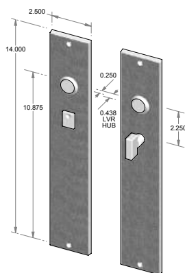
CS-F2214IML-PR – Complete privacy set with interior mortise lock and spindle. OR TS-F2214IML-PR – Trim set only. No lock.
