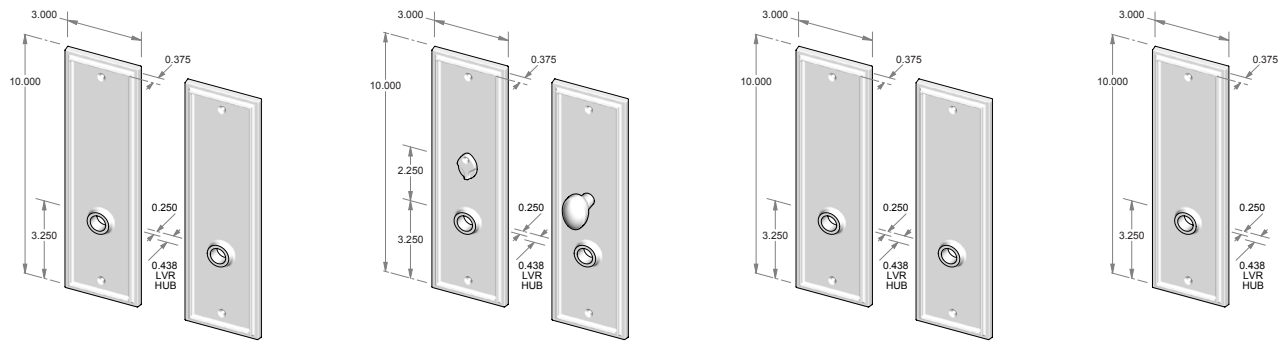
CS-422IML – Complete passage set with interior mortise lock and spindle. OR TS-422IML – Trim set only. No lock.
