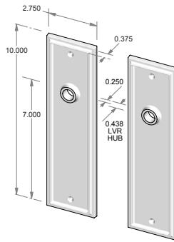
TS-F426IML-FD – Trim set only. – Full dummy.
