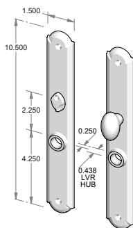
CS-A811IML-PR – Complete privacy set with interior mortise lock and spindle. OR TS-A811IML-PR – Trim set only. No lock.
