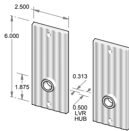
CS-1406IML – Complete passage set with interior mortise lock and spindle. OR TS-1406IML – Trim set only. No lock.
