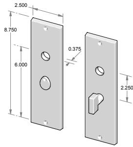
CS-F-N953IML-PR – Complete privacy set with interior mortise lock and spindle. OR TS-F-N953IML-PR – Trim set only. No lock.
