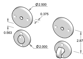
CS-F-RP-N926-8xRP9200IML-PR – Complete privacy set with interior mortise lock and spindle. OR TS-F-RP-N926-8xRP9200IML-PR – Trim set only. No lock.
