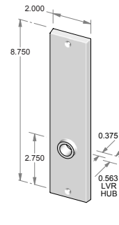
TS-950IML-HD – Trim set only. – Half dummy.
