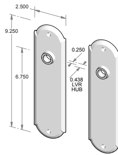
TS-F-A408IML-FD – Trim set only. – Full dummy.
