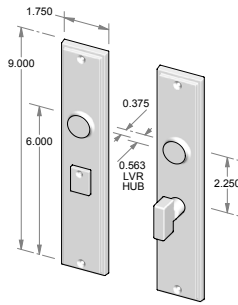
CS-F2109IML-PR – Complete privacy set with interior mortise lock and spindle. OR TS-F2109IML-PR – Trim set only. No lock.
