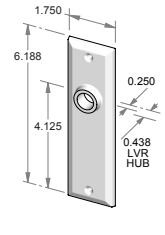
TS-F405IML-HD – Trim set only. – Full dummy.
