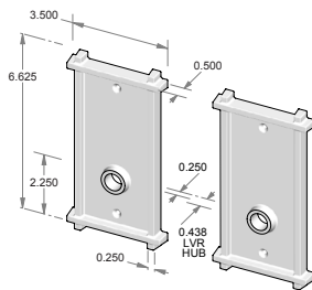
CS-356IML – Complete passage set with interior mortise lock and spindle. OR TS-356IML – Trim set only. No lock.
