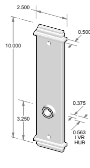
TS-440IML-HD – Trim set only. – Full dummy.
