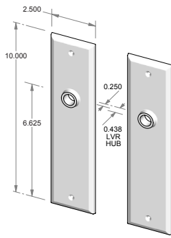
CS-F409IML – Complete passage set with interior mortise lock and spindle. OR TS-F409IML – Trim set only. No lock.
