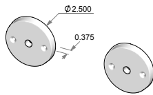
TS-RP-N926-8IML-FD – Trim set only. – Full dummy.
