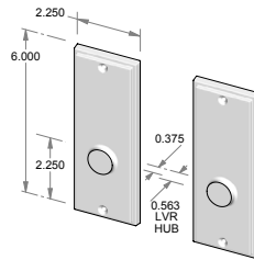
TS-2106IML-FD – Trim set only. – Full dummy.
