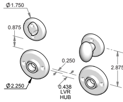
CS-RP225-8xRP175IML-PR – Complete privacy set with interior mortise lock and spindle. OR TS-RP225-8xRP175IML-PR – Trim set only. No lock.
