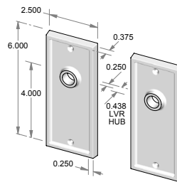
TS-F1506IML-FD – Trim set only. – Full dummy.
