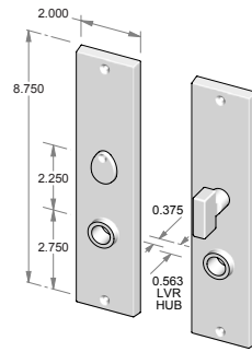
CS-950IML-PR – Complete privacy set with interior mortise lock and spindle. OR TS-950IML-PR – Trim set only. No lock.
