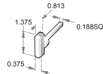
ERK-767 – Emergency release key.
