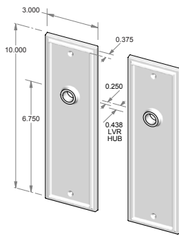
CS-F422IML – Complete passage set with interior mortise lock and spindle. OR TS-F422IML – Trim set only. No lock.
