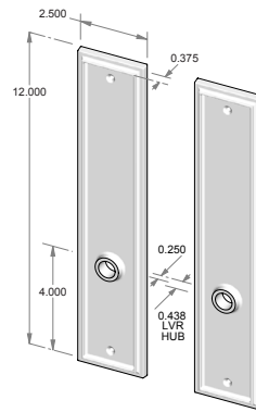
TS-423IML-FD – Trim set only. – Full dummy.
