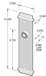
TS-F440IML-HD – Trim set only. – Full dummy.
