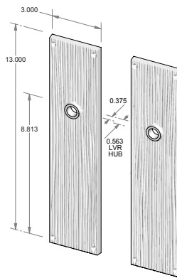
TS-F1912IML-FD – Trim set only. – Full dummy.
