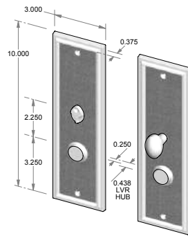
CS-2410IML-PR – Complete privacy set with interior mortise lock and spindle. OR TS-2410IML-PR – Trim set only. No lock.
