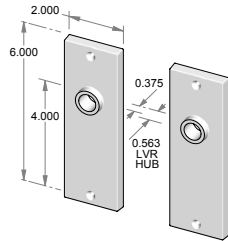
CS-F949IML – Complete passage set with interior mortise lock and spindle. OR TS-F949IML – Trim set only. No lock.
