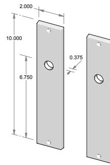
TS-F-N951IML-FD – Trim set only. – Full dummy.
