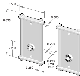
TS-356IML-FD – Trim set only. – Full dummy.
