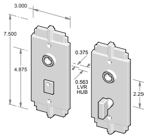
CS-F366IML-PR – Complete privacy set with interior mortise lock and spindle. OR TS-F366IML-PR – Trim set only. No lock.
