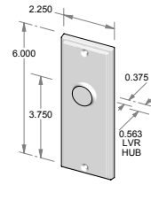
TS-F2106IML-HD – Trim set only. – Full dummy.
