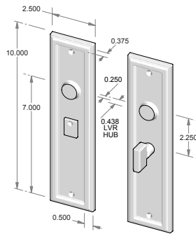
CS-F2510IML-PR – Complete privacy set with interior mortise lock and spindle. OR TS-F2510IML-PR – Trim set only. No lock.
