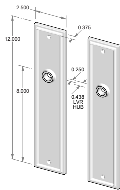
CS-F423IML – Complete passage set with interior mortise lock and spindle. OR TS-F423IML – Trim set only. No lock.
