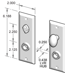
CS-206IML-PR – Complete privacy set with interior mortise lock and spindle. OR TS-206IML-PR – Trim set only. No lock.
