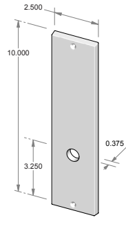
TS-N952IML-HD – Trim set only. – Full dummy.
