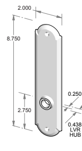
TS-A407IML-HD – Trim set only. – Full dummy.
