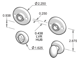
CS-F-RP225-8xRP158IML-PR – Complete privacy set with interior mortise lock and spindle. OR TS-F-RP225-8xRP158IML-PR – Trim set only. No lock.
