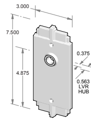
TS-F366IML-HD – Trim set only. – Full dummy.
