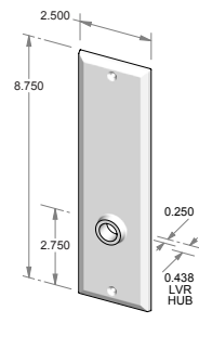
TS-408IML-HD – Trim set only. – Full dummy.
