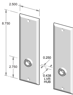
CS-408IML – Complete passage set with interior mortise lock and spindle. OR TS-408IML – Trim set only. No lock.
