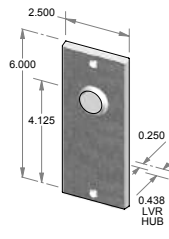
TS-F2206IML-HD – Trim set only. – Full dummy.
