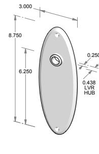
TS-F-OP700IML-HD – Trim set only. – Full dummy.
