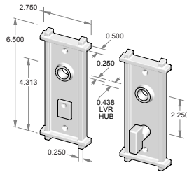
CS-F355IML-PR – Complete privacy set with interior mortise lock and spindle. OR TS-F355IML-PR – Trim set only. No lock.
