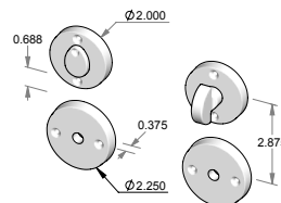
CS-RP-N925-8xRP9200IML-PR – Complete privacy set with interior mortise lock and spindle. OR TS-RP-N925-8xRP9200IML-PR – Trim set only. No lock.
