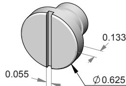
CR-9-2 Contemporary coin release. NOT available w/indicator.
