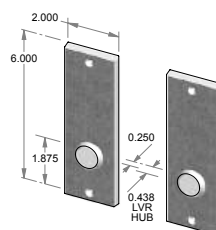
TS-2205IML-FD – Trim set only. – Full dummy.
