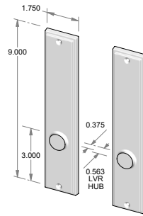
TS-2109IML-FD – Trim set only. – Full dummy.
