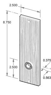
TS-1908IML-HD – Trim set only. – Full dummy.
