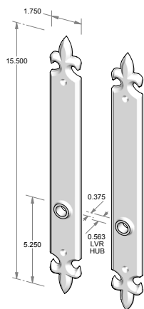
CS-1240IML – Complete passage set with interior mortise lock and spindle. OR TS-1240IML – Trim set only. No lock.
