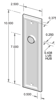
TS-F2510IML-HD – Trim set only. – Full dummy.
