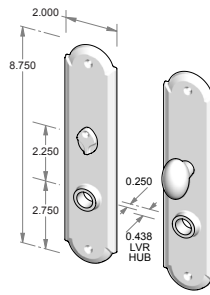
CS-A407IML-PR – Complete privacy set with interior mortise lock and spindle. OR TS-A407IML-PR – Trim set only. No lock.
