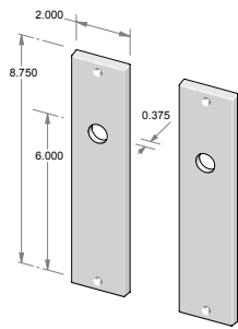
CS-F-N950IML – Complete passage set with interior mortise lock and spindle. OR TS-F-N950IML – Trim set only. No lock.
