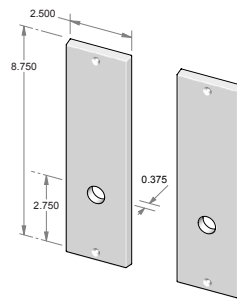
TS-N953IML-FD – Trim set only. – Full dummy.
