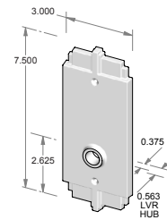
TS-366IML-HD – Trim set only. – Full dummy.
