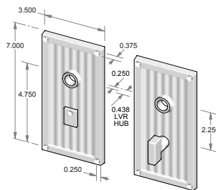
CS-F336IML-PR – Complete privacy set with interior mortise lock and spindle. OR TS-F336IML-PR – Trim set only. No lock.
