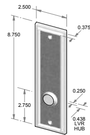
TS-2408IML-HD – Trim set only. – Full dummy.
