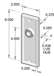
TS-F1505IML-HD – Trim set only. – Half dummy.
