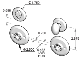
CS-RP402-8xRP175IML-PR – Complete privacy set with interior mortise lock and spindle. OR TS-RP402-8xRP175IML-PR – Trim set only. No lock.
