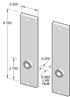
CS-950IML – Complete passage set with interior mortise lock and spindle. OR TS-950IML – Trim set only. No lock.
