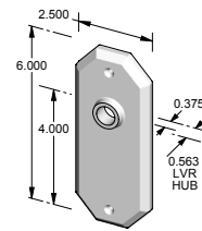
TS-F2306IML-HD – Trim set only. – Half dummy.
