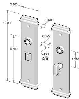
CS-F440IML-PR – Complete privacy set with interior mortise lock and spindle. OR TS-F440IML-PR – Trim set only. No lock.
