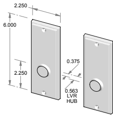
CS-2106IML – Complete passage set with interior mortise lock and spindle. OR TS-2106IML – Trim set only. No lock.
