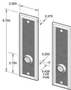
CS-2408IML – Complete passage set with interior mortise lock and spindle. OR TS-2408IML – Trim set only. No lock.
