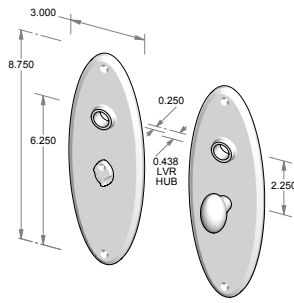
CS-F-OP700IML-PR – Complete privacy set with interior mortise lock and spindle. OR TS-F-OP700IML-PR – Trim set only. No lock.
