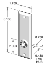
TS-405IML-HD – Trim set only. – Full dummy.
