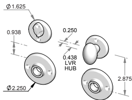
CS-RP-E225-8IML-PR – Complete privacy set with interior mortise lock and spindle. OR TS-RP-E225-8IML-PR – Trim set only. No lock.
