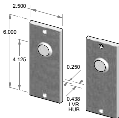
CS-F2206IML – Complete passage set with interior mortise lock and spindle. OR TS-F2206IML – Trim set only. No lock.
