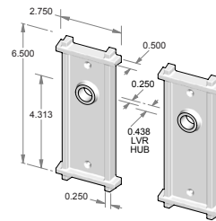
TS-F355IML-FD – Trim set only. – Full dummy.
