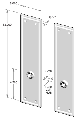
TS-425IML-FD – Trim set only. – Full dummy.
