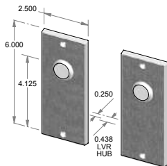
TS-F2206IML-FD – Trim set only. – Full dummy.
