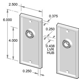
CS-F1506IML – Complete passage set with interior mortise lock and spindle. OR TS-F1506IML – Trim set only. No lock.
