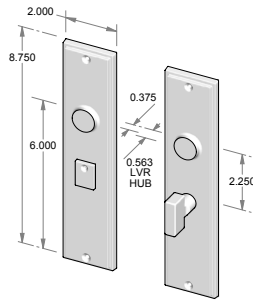
CS-F2107IML-PR – Complete privacy set with interior mortise lock and spindle. OR TS-F2107IML-PR – Trim set only. No lock.
