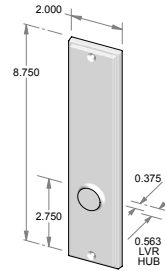
TS-2107IML-HD – Trim set only. – Full dummy.
