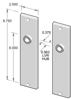
CS-F950IML – Complete passage set with interior mortise lock and spindle. OR TS-F950IML – Trim set only. No lock.
