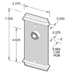
TS-F346IML-HD – Trim set only. – Full dummy.
