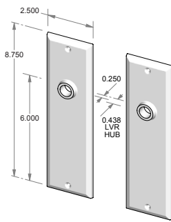
CS-F408IML – Complete passage set with interior mortise lock and spindle. OR TS-F408IML – Trim set only. No lock.
