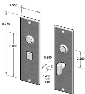
CS-F2208IML-PR – Complete privacy set with interior mortise lock and spindle. OR TS-F2208IML-PR – Trim set only. No lock.
