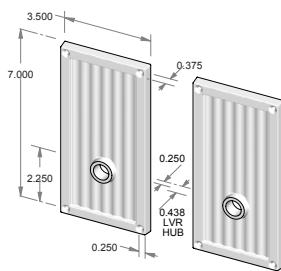
CS-336IML – Complete passage set with interior mortise lock and spindle. OR TS-336IML – Trim set only. No lock.
