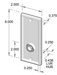
TS-1506IML-HD – Trim set only. – Half dummy.
