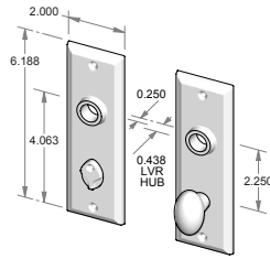
CS-F206IML-PR – Complete privacy set with interior mortise lock and spindle. OR TS-F206IML-PR – Trim set only. No lock.
