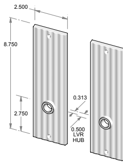
CS-1408IML – Complete passage set with interior mortise lock and spindle. OR TS-1408IML – Trim set only. No lock.
