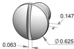
CR-2 Coin release. NOT available w/ indicator.
