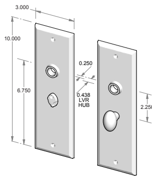
CS-F410IML-PR – Complete privacy set with interior mortise lock and spindle. OR TS-F410IML-PR – Trim set only. No lock.
