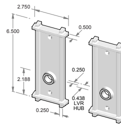
TS-355IML-FD – Trim set only. – Full dummy.
