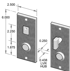
CS-2206IML-PR – Complete privacy set with interior mortise lock and spindle. OR TS-2206IML-PR – Trim set only. No lock.
