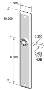
TS-F811IML-HD – Trim set only. – Full dummy.
