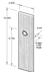
TS-F1910IML-HD – Trim set only. – Full dummy.
