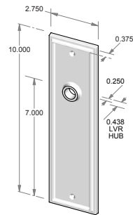
TS-F426IML-HD – Trim set only. – Full dummy.
