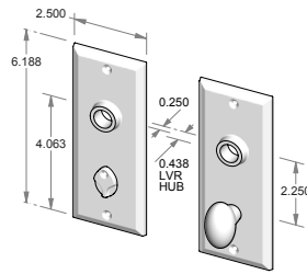
CS-F406IML-PR – Complete privacy set with interior mortise lock and spindle. OR TS-F406IML-PR – Trim set only. No lock.
