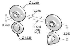
CS-F-RP925IML-PR – Complete privacy set with interior mortise lock and spindle. OR TS-F-RP925IML-PR – Trim set only. No lock.
