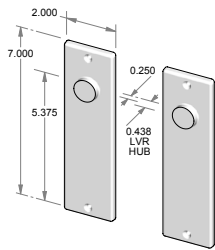
CS-F-E206IML – Complete passage set with interior mortise lock and spindle. OR TS-F-E206IML – Trim set only. No lock.
