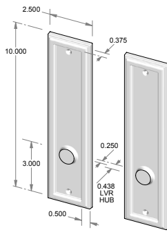
CS-2510IML – Complete passage set with interior mortise lock and spindle. OR TS-2510IML – Trim set only. No lock.
