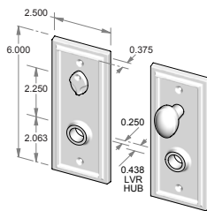
CS-325IML-PR – Complete privacy set with interior mortise lock and spindle. OR TS-325IML-PR – Trim set only. No lock.
