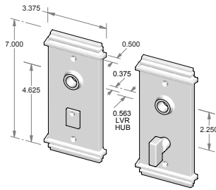
CS-F346IML-PR – Complete privacy set with interior mortise lock and spindle. OR TS-F346IML-PR – Trim set only. No lock.
