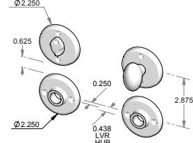
CS-RP225-8xRP225IML-PR – Complete privacy set with interior mortise lock and spindle. OR TS-RP225-8xRP225IML-PR – Trim set only. No lock.
