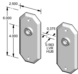
CS-F2306IML – Complete passage set with interior mortise lock and spindle. OR TS-F2306IML – Trim set only. No lock.
