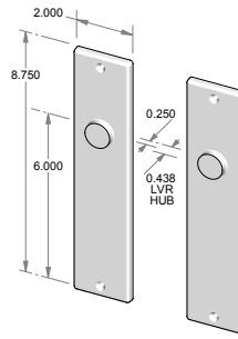
TS-F-E407IML-FD – Trim set only. – Full dummy.
