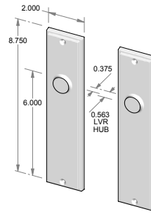
TS-F2107IML-FD – Trim set only. – Full dummy.
