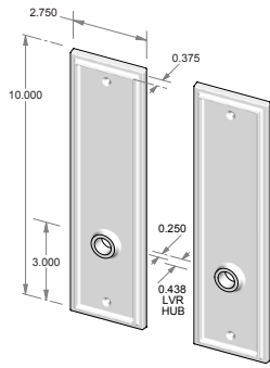
CS-426IML – Complete passage set with interior mortise lock and spindle. OR TS-426IML – Trim set only. No lock.
