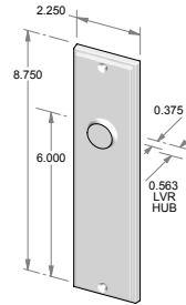
TS-F2108IML-HD – Trim set only. – Full dummy.
