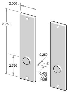
CS-E407IML – Complete passage set with interior mortise lock and spindle. OR TS-E407IML – Trim set only. No lock.
