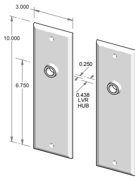
CS-F410IML – Complete passage set with interior mortise lock and spindle. OR TS-F410IML – Trim set only. No lock.
