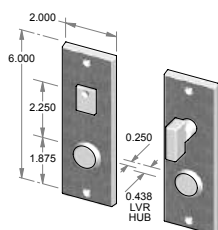
CS-2205IML-PR – Complete privacy set with interior mortise lock and spindle. OR TS-2205IML-PR – Trim set only. No lock.
