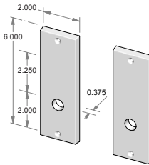
TS-N949IML-FD – Trim set only. – Full dummy.
