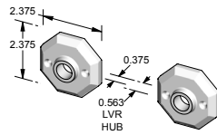
CS-F2301-8IML – Complete passage set with interior mortise lock and spindle. OR TS-F2301-8IML – Trim set only. No lock.
