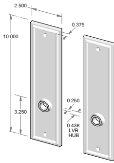
CS-424IML – Complete passage set with interior mortise lock and spindle. OR TS-424IML – Trim set only. No lock.
