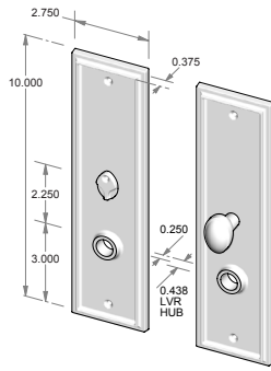
CS-426IML-PR – Complete privacy set with interior mortise lock and spindle. OR TS-426IML-PR – Trim set only. No lock.
