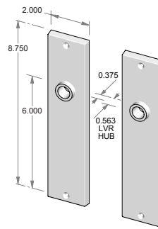
TS-F950IML-FD – Trim set only. – Full dummy.
