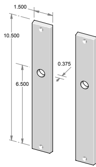
CS-F-N980IML – Complete passage set with interior mortise lock and spindle. OR TS-F-N980IML – Trim set only. No lock.
