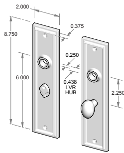
CS-F420IML-PR – Complete privacy set with interior mortise lock and spindle. OR TS-F420IML-PR – Trim set only. No lock.
