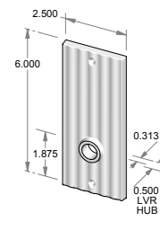
TS-1406IML-HD – Trim set only. – Half dummy.
