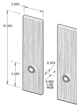
CS-1910IML – Complete passage set with interior mortise lock and spindle. OR TS-1910IML – Trim set only. No lock.
