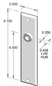
TS-F407IML-HD – Trim set only. – Full dummy.
