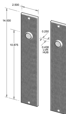
TS-F2214IML-FD – Trim set only. – Full dummy.
