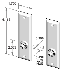
CS-405IML – Complete passage set with interior mortise lock and spindle. OR TS-405IML – Trim set only. No lock.
