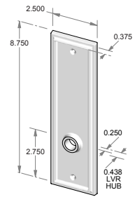
TS-421IML-HD – Trim set only. – Full dummy.
