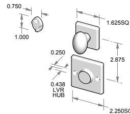
CS-E225-8IML-PR-RC – Complete privacy set with interior mortise lock and spindle. OR TS-E225-8IML-PR-RC – Trim set only. No lock.
