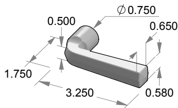
L-96 Squarelet Lever
