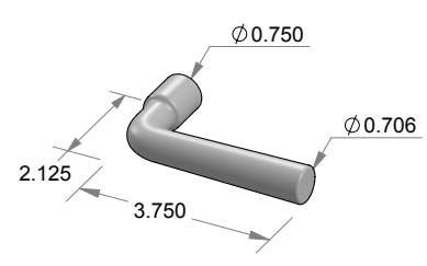
L-12.75 Extended Tiny Tube Lever
