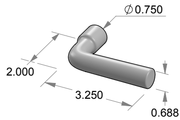
L-12 Tiny Tube Lever
