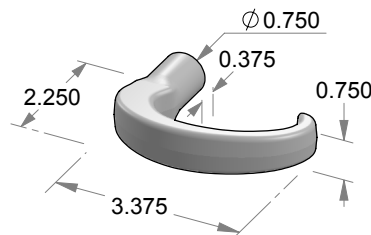
L-94 Little Hook Lever
