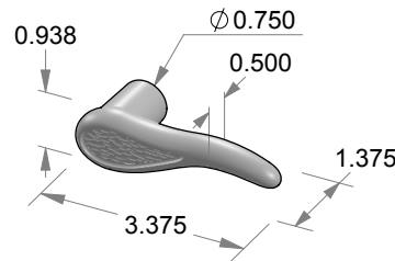
L-91 Little Horn Lever
