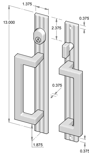
CMP-US-1430SL – Complete set with keyed US cylinder and SVB turn piece. – Single cylinder. – Shown with GH-130SL.
