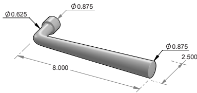
LS-130 Ruby lift & slide lever.
