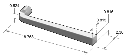
LS-115 Square lift & slide lever.
