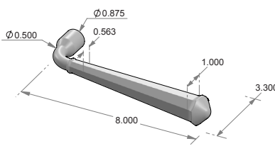
LS-128 Stanley lift & slide lever.
