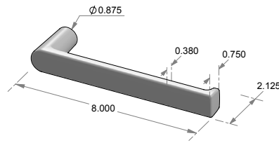
LS-125 Flat lift & slide lever.
