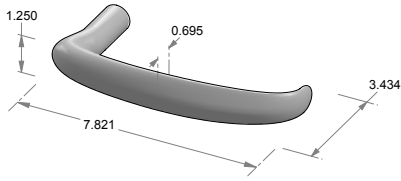
LS-107 Large Hook lift & slide lever.
