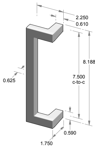
GH-131SL 8.188" Contemporary grip handle.
