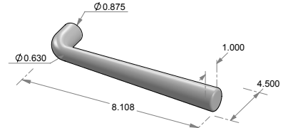
LS-119 Muldoon lift & slide lever.
