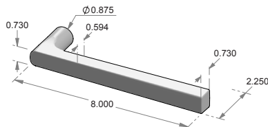
LS-122 Metro lift & slide lever.
