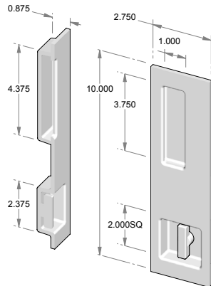
BFP-1000RH – Bi-fold flush cup pull set. – 0.687" Interior depth. – Right hand.
