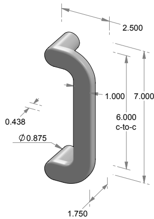
GH-112SL 7.000" Grip handle.
