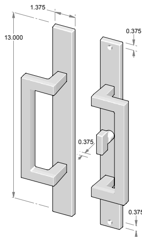
CMP-US-918SL-PF – Complete set with SVB turn piece. – Patio function. – Shown with GH-130SL.
