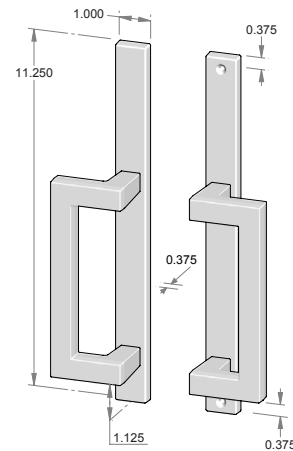
CMP-US-820SL-FD - Trim set only. - Full dummy. - Shown with GH-129SL.
