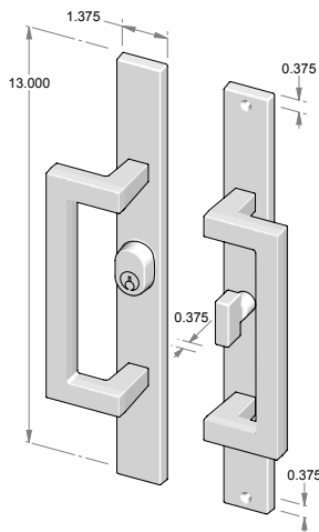
CMP-US-918SL – Complete set with keyed US cylinder and SVB turn piece. – Single cylinder. – Shown with GH-130SL.
