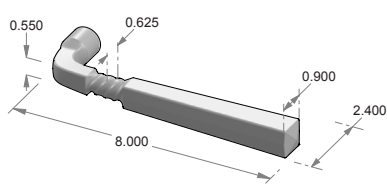
LS-123 Twist lift & slide lever.
