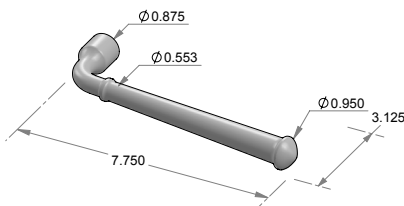
LS-127 Hailey lift & slide lever.
