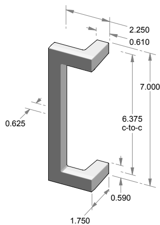
GH-130SL 7.000" Contemporary grip handle.
