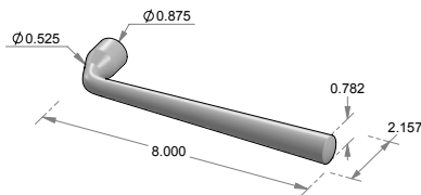
LS-113 Alturas lift & slide lever.
