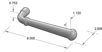
LS-143 Harriman lift & slide lever.
