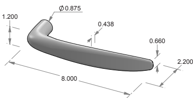
LS-155 White Cloud lift & slide lever.
