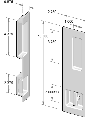
BFP-1000LH – Bi-fold flush cup pull set. – 0.687" Interior depth. – Left hand.
