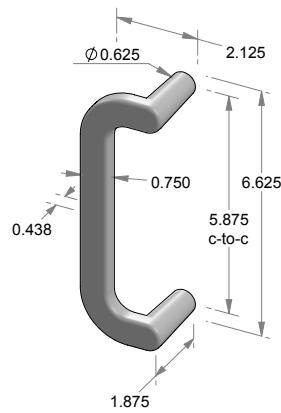
GH-110SL 6.625" Grip handle.
