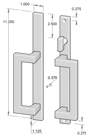
CMP-US-820SL-PF - Complete set with SVB turn piece. - Patio function. - Shown with GH-129SL.
