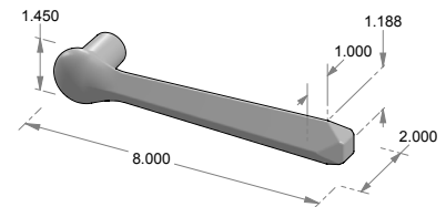
LS-170 Preston lift & slide lever.
