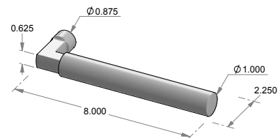
LS-160 Pioneer lift & slide lever.
