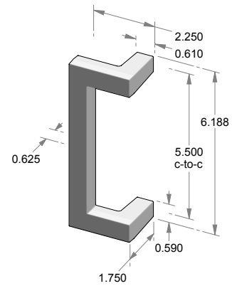
GH-129SL 6.188" Contemporary grip handle.
