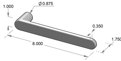
LS-111 Flat lift & slide lever.
