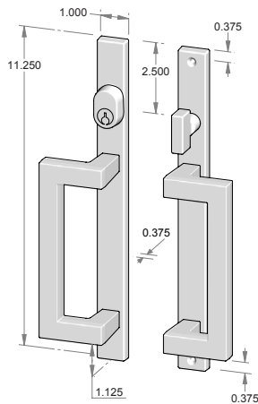
CMP-US-820SL - Complete set with keyed US cylinder and SVB turn piece. - Single cylinder. - Shown with GH-129SL.
