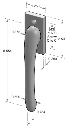
BFS-900 – Retrofit bi-fold door latch. – Shown with L-90 lever.
