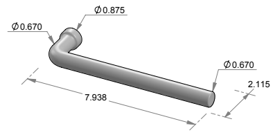
LS-112 Tube lift & slide lever.
