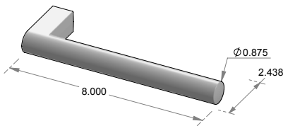
LS-165SQ Pettit lift & slide lever. * Square hub for use with Novus.
