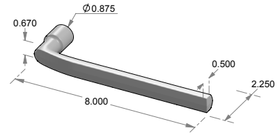
LS-151 Alpen lift & slide lever.
