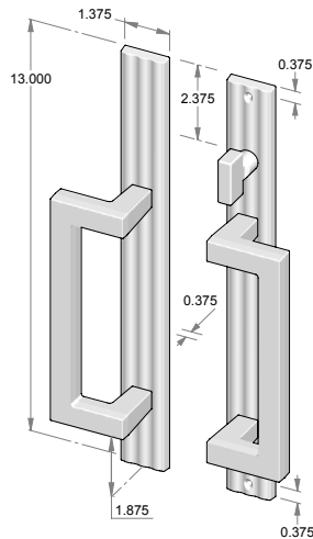
CMP-US-1430SL-PF – Complete set with SVB turn piece. – Patio function. – Shown with GH-130SL.
