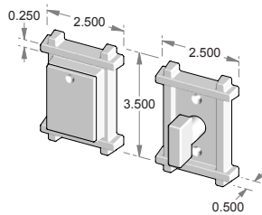
CS-521/522DL – Complete set with deadlock and cylinder. – Single cylinder. OR TS-521/522DL – Trim set only. No lock.
