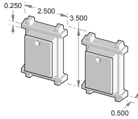
CS-521DL-DC – Complete set with deadlock and cylinders. – Double cylinder. OR TS-521DL-DC – Trim set only. No lock.
