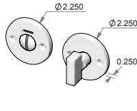
CS-I-RP925MB – Complete vacant-occupied indicator set w/mortise bolt. OR TS-I-RP926MB – Trim set only. No latch.
