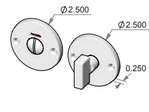
CS-I-RP926MB – Complete vacant-occupied indicator set w/mortise bolt. OR TS-I-RP926MB – Trim set only. No latch.
