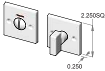
CS-I-925MB – Complete vacant-occupied indicator set w/mortise bolt. OR TS-I-925MB – Trim set only. No latch.
