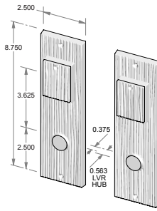
CS-1908PLD-DC – Complete set with passage latch, deadbolt, cylinders and spindle. – Double cylinder. – Shown with KC-1900. OR TS-1908PLD-DC – Trim set only. No latch or deadbolt.
