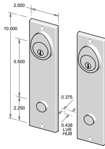
CS-952-5.5PLD-DC-NKC* – Complete set with passage latch, deadbolt, cylinders and spindle. – Double cylinder. – *Shown without key cover. Must be specified NKC. OR TS-952-5.5PLD-DC-NKC – Trim set only. No latch or deadbolt.
