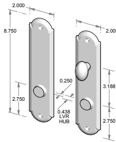
CS-A407PLD-PF – Complete set with passage latch, deadbolt and spindle. – Patio function. OR TS-A407PLD-PF – Trim set only. No latch or deadbolt.
