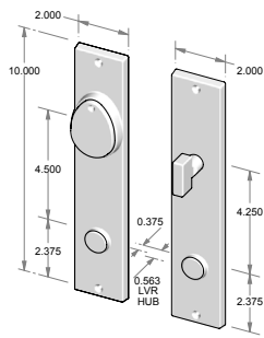
CS-951PLD – Complete set with passage latch, deadbolt, cylinder and spindle. – Single cylinder. OR TS-951PLD – Trim set only. No latch or deadbolt.
