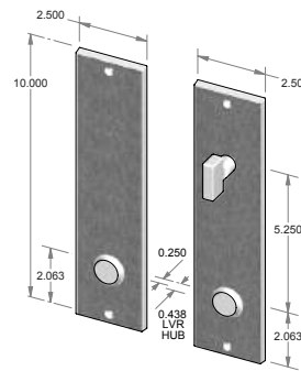
CS-2210-5.5PLD-PF – Complete set with passage latch, deadbolt and spindle. – Patio function. OR TS-2210-5.5PLD-PF – Trim set only. No latch or deadbolt.
