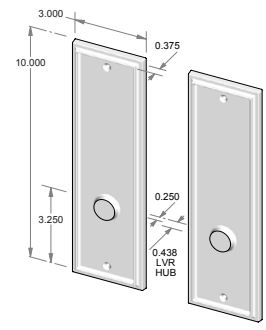
TS-422PLD-FD – Trim set only. – Full dummy.
