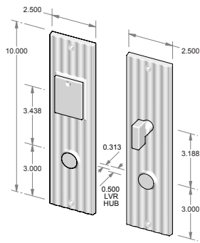
CS-1410PLD – Complete set with passage latch, deadbolt, cylinder and spindle. – Single cylinder. OR TS-1410PLD – Trim set only. No latch or deadbolt.
