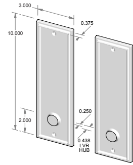
TS-422-5.5PLD-FD – Trim set only. – Full dummy.
