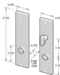
CS-950PLD-P* – Complete set with passage latch, deadbolt and spindle. – Patio function. OR TS-950PLD-PF – Trim set only. No latch or deadbolt.
