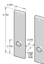
TS-950PLD-FD – Trim set only. – Full dummy.
