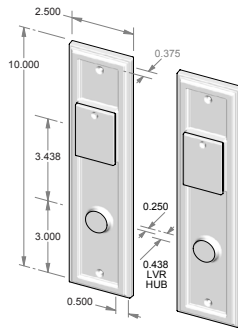
CS-2510PLD-DC – Complete set with passage latch, deadbolt, cylinders and spindle. – Double cylinder. OR TS-2510PLD-DC – Trim set only. No latch or deadbolt.
