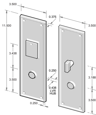
CS-1512PLD – Complete set with passage latch, deadbolt, cylinder and spindle. – Single cylinder. OR TS-1512PLD – Trim set only. No latch or deadbolt.
