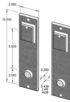
CS-2210-5.5PLD-DC – Complete set with passage latch, deadbolt, cylinders and spindle. – Double cylinder. – Shown with KC-2200. OR TS-2210-5.5PLD-DC – Trim set only. No latch or deadbolt.
