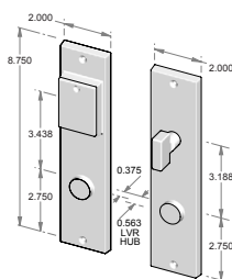
CS-950R-PLD – Complete set with passage latch, deadbolt, cylinder and spindle. – Single cylinder. OR TS-950R-PLD – Trim set only. No latch or deadbolt.
