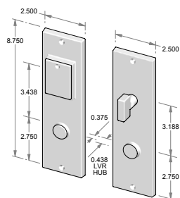
CS-953R-PLD – Complete set with passage latch, deadbolt, cylinder and spindle. – Single cylinder. OR TS-953R-PLD – Trim set only. No latch or deadbolt.
