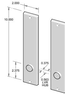
TS-951PLD-FD – Trim set only. – Full dummy.
