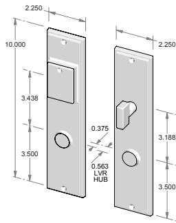
CS-2110PLD – Complete set with passage latch, deadbolt, cylinder and spindle. – Single cylinder. OR TS-2110PLD – Trim set only. No latch or deadbolt.
