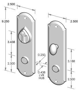
CS-A408PLD – Complete set with passage latch, deadbolt, cylinder and spindle. – Single cylinder. OR TS-A408PLD – Trim set only. No latch or deadbolt.
