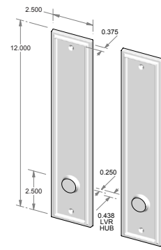
TS-423PLD-FD - Trim set only. - Full dummy.
