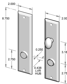
CS-407PLD-PF – Complete set with passage latch, deadbolt and spindle. – Patio function. OR TS-407PLD-PF – Trim set only. No latch or deadbolt.
