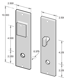
CS-N952R-PLD – Complete set with passage latch, deadbolt, cylinder and spindle. – Single cylinder. OR TS-N952R-PLD – Trim set only. No latch or deadbolt.
