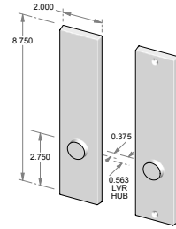
TS-950PLD-FD – Trim set only. – Full dummy.
