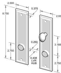
CS-420PLD-PF - Complete set with passage latch, deadbolt and spindle. - Patio function. - Shown with TPC-306. OR TS-420PLD-PF - Trim set only. No latch or deadbolt.
