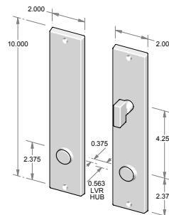
CS-951PLD-PF – Complete set with passage latch, deadbolt and spindle. – Patio function. OR TS-951PLD-PF – Trim set only. No latch or deadbolt.
