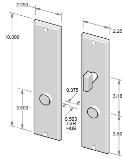
CS-2110PLD-PF – Complete set with passage latch, deadbolt and spindle. – Patio function. OR TS-2110PLD-PF – Trim set only. No latch or deadbolt.
