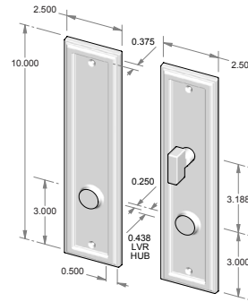
CS-2510PLD-PF – Complete set with passage latch, deadbolt and spindle. – Patio function. OR TS-2510PLD-PF – Trim set only. No latch or deadbolt.
