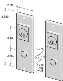
CS-953R-PLD-DC-NKC* – Complete set with passage latch, deadbolt, cylinders and spindle. – Double cylinder. – *Shown without key cover. Must be specified NKC. OR TS-953R-PLD-DC-NKC – Trim set only. No latch or deadbolt.
