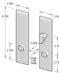
CS-2107PLD-PF – Complete set with passage latch, deadbolt and spindle. – Patio function. OR TS-2107PLD-PF – Trim set only. No latch or deadbolt.
