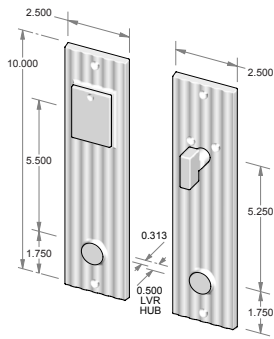
CS-1410-5.5PLD – Complete set with passage latch, deadbolt, cylinder and spindle. – Single cylinder. OR TS-1410-5.5PLD – Trim set only. No latch or deadbolt.
