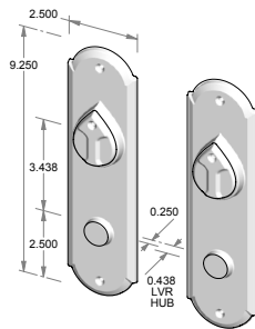
CS-A408PLD-DC – Complete set with passage latch, deadbolt, cylinders and spindle. – Double cylinder. OR TS-A408PLD-DC – Trim set only. No latch or deadbolt.
