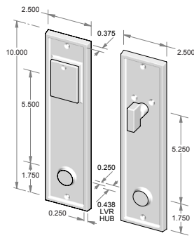
CS-1510-5.5PLD – Complete set with passage latch, deadbolt, cylinder and spindle. – Single cylinder. OR TS-1510-5.5PLD – Trim set only. No latch or deadbolt.
