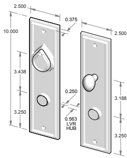
CS-424PLD – Complete set with passage latch, deadbolt, cylinder and spindle. – Single cylinder. – Shown with KC-300 and TPC-306. OR TS-424PLD – Trim set only. No latch or deadbolt.
