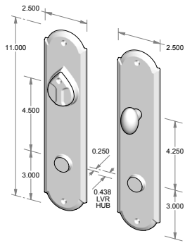
CS-A409PLD – Complete set with passage latch, deadbolt, cylinder and spindle. – Single cylinder. OR TS-A409PLD – Trim set only. No latch or deadbolt.
