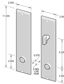
CS-2111-5.5PLD-PF – Complete set with passage latch, deadbolt and spindle. – Patio function. OR TS-2111-5.5PLD-PF – Trim set only. No latch or deadbolt.
