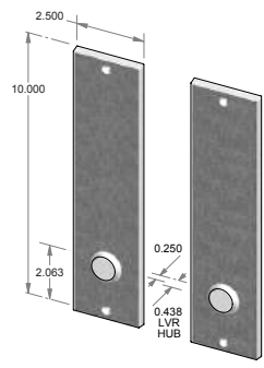
TS-2210-5.5PLD-FD – Trim set only. – Full dummy.
