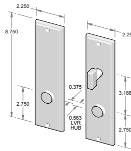
CS-2108PLD-PF – Complete set with passage latch, deadbolt and spindle. – Patio function. OR TS-2108PLD-PF – Trim set only. No latch or deadbolt.
