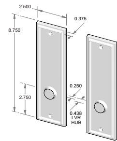
TS-421PLD-FD – Trim set only. – Full dummy.
