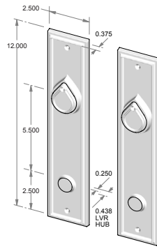
CS-423-5.5PLD-DC – Complete set with passage latch, deadbolt, cylinders and spindle. – Double cylinder. – Shown with KC-300. OR TS-423-5.5PLD-DC – Trim set only. No latch or deadbolt.
