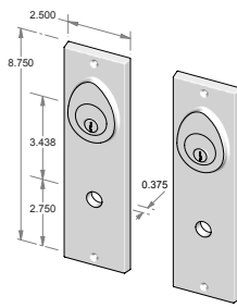
CS-N953PLD-DC-NKC* – Complete set with passage latch, deadbolt, cylinders and spindle. – Double cylinder. – *Shown without key cover. Must be specified NKC. OR TS-N953PLD-DC-NKC – Trim set only. No latch or deadbolt.
