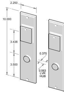
CS-2110PLD-DC – Complete set with passage latch, deadbolt, cylinders and spindle. – Double cylinder. OR TS-2110PLD-DC – Trim set only. No latch or deadbolt.
