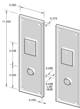
CS-1512PLD-DC – Complete set with passage latch, deadbolt, cylinders and spindle. – Double cylinder. OR TS-1512PLD-DC – Trim set only. No latch or deadbolt.
