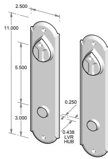
CS-A409-5.5PLD-DC – Complete set with passage latch, deadbolt, cylinders and spindle. – Double cylinder. OR TS-A409-5.5PLD-DC – Trim set only. No latch or deadbolt.
