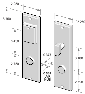
CS-2108PLD – Complete set with passage latch, deadbolt, cylinder and spindle. – Single cylinder. OR TS-2108PLD – Trim set only. No latch or deadbolt.
