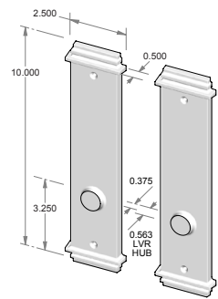
TS-440PLD-FD – Trim set only. – Full dummy.
