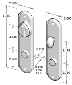
CS-A407PLD – Complete set with passage latch, deadbolt, cylinder and spindle. – Single cylinder. OR TS-A407PLD – Trim set only. No latch or deadbolt.
