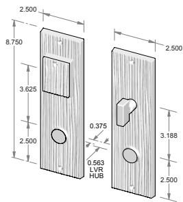
CS-1908PLD – Complete set with passage latch, deadbolt, cylinder and spindle. – Single cylinder. – Shown with KC-1900. OR TS-1908PLD – Trim set only. No latch or deadbolt.
