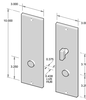
CS-955PLD-PF – Complete set with passage latch, deadbolt and spindle. – Patio function. OR TS-955PLD-PF – Trim set only. No latch or deadbolt.
