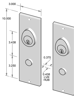
CS-955PLD-DC-NKC* – Complete set with passage latch, deadbolt, cylinders and spindle. – Double cylinder. – *Shown without key cover. Must be specified NKC. OR TS-955PLD-DC-NKC – Trim set only. No latch or deadbolt.
