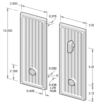
CS-431-5.5PLD-PF – Complete set with passage latch, deadbolt and spindle. – Patio function. OR TS-431-5.5PLD-PF – Trim set only. No latch or deadbolt.
