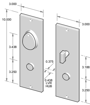
CS-955PLD – Complete set with passage latch, deadbolt, cylinder and spindle. – Single cylinder. OR TS-955PLD – Trim set only. No latch or deadbolt.
