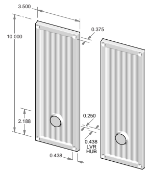
TS-431-5.5PLD-FD – Trim set only. – Full dummy.
