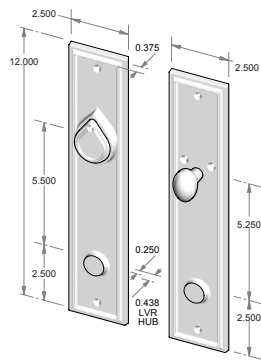
CS-423-5.5PLD – Complete set with passage latch, deadbolt, cylinder and spindle. – Single cylinder. – Shown with KC-300 and TPC-306. OR TS-423-5.5PLD – Trim set only. No latch or deadbolt.
