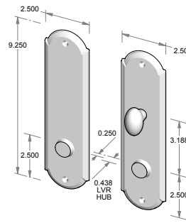
CS-A408PLD-PF – Complete set with passage latch, deadbolt and spindle. – Patio function. OR TS-A408PLD-PF – Trim set only. No latch or deadbolt.
