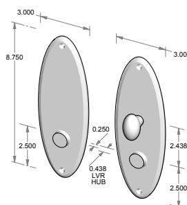
CS-OP700PLD-PF - Complete set with passage latch, deadbolt and spindle. - Patio function. OR TS-OP700PLD-PF - Trim set only. No latch or deadbolt.
