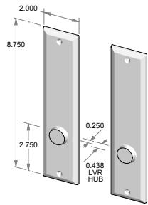
TS-407PLD-FD – Trim set only. – Full dummy.
