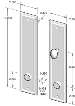
CS-423-5.5PLD-PF – Complete set with passage latch, deadbolt and spindle. – Patio function. – Shown with TPC-306. OR TS-423-5.5PLD-PF – Trim set only. No latch or deadbolt.
