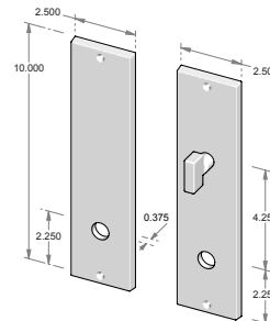
CS-N952PLD-PF – Complete set with passage latch, deadbolt and spindle. – Patio function. OR TS-N952PLD-PF – Trim set only. No latch or deadbolt.
