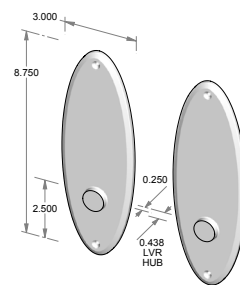
TS-OP700PLD-FD - Trim set only. - Full dummy.
