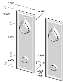
CS-422-5.5PLD-DC – Complete set with passage latch, deadbolt, cylinders and spindle. – Double cylinder. – Shown with KC-300. OR TS-422-5.5PLD-DC – Trim set only. No latch or deadbolt.
