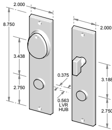
CS-950PLD – Complete set with passage latch, deadbolt, cylinder and spindle. – Single cylinder. OR TS-950PLD – Trim set only. No no latch or deadbolt.
