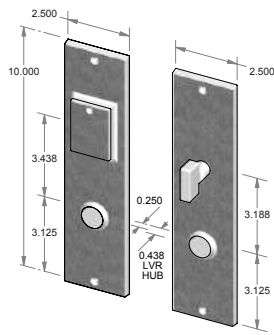
CS-2210PLD – Complete set with passage latch, deadbolt, cylinder and spindle. – Single cylinder. – Shown with KC-2200. OR TS-2210PLD – Trim set only. No latch or deadbolt.
