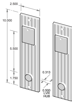
CS-1410-5.5PLD-DC – Complete set with passage latch, deadbolt, cylinders and spindle. – Double cylinder. OR TS-1410-5.5PLD-DC – Trim set only. No latch or deadbolt.
