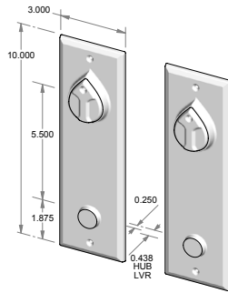
CS-410-5.5PLD-DC – Complete set with passage latch, deadbolt, cylinders and spindle. – Double cylinder. OR TS-410-5.5PLD-DC – Trim set only. No latch or deadbolt.
