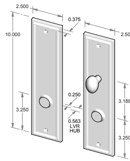
CS-424PLD-PF – Complete set with passage latch, deadbolt and spindle. – Patio function. – Shown with TPC-306. OR TS-424PLD-PF – Trim set only. No latch or deadbolt.
