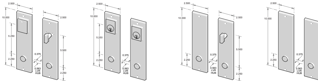
CS-952R5.5PLD – Complete set with passage latch, deadbolt, cylinder and spindle. – Single cylinder. OR TS-952R5.5PLD – Trim set only. No latch or deadbolt.
