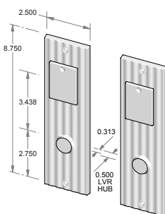
CS-1408PLD-DC – Complete set with passage latch, deadbolt, cylinders and spindle. – Double cylinder. OR TS-1408PLD-DC – Trim set only. No latch or deadbolt.
