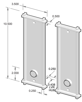
TS-451-5.5PLD-FD – Trim set only. – Full dummy.
