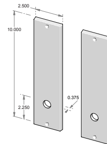
TS-N952PLD-FD – Trim set only. – Full dummy.
