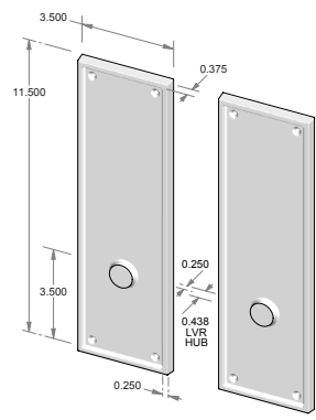
TS-1512PLD-FD – Trim set only. – Full dummy.
