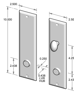
CS-409PLD-PF - Complete set with passage latch, deadbolt and spindle. - Patio function. OR TS-409PLD-PF - Trim set only. No latch or deadbolt.
