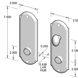
CS-A406PLD-PF – Complete set with passage latch, deadbolt and spindle. – Patio function. OR TS-A406PLD-PF – Trim set only. No latch or deadbolt.
