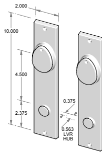
CS-951PLD-DC-NKC* – Complete set with passage latch, deadbolt, cylinders and spindle. – Double cylinder. – *Shown without key cover. Must be specified NKC. OR TS-951PLD-DC-NKC – Trim set only. No latch or deadbolt.
