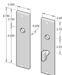
CS-F-N950ML-PF – Complete set with mortise lock and spindle. – Patio function. OR TS-F-N950ML-PF – Trim set only. No lock.
