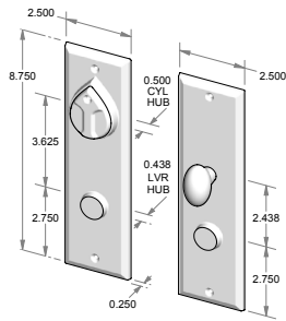
CS-408ML – Complete set with mortise lock, cylinder and spindle. – Single cylinder. OR TS-408ML – Trim set only. No lock.
