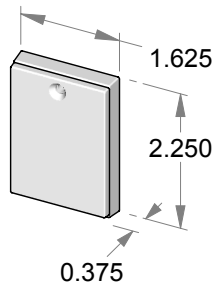
CC-407ML-C Rectangular mortise cylinder collar w/key cover.
