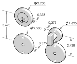
CS-RP-N926ML – Complete set with mortise lock, cylinder and spindle. – Single cylinder. – Shown with 9507ML-C. OR TS-RP-N926ML – Trim set only. No lock.
