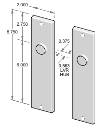
TS-F950ML-FD – Trim set only. – Full dummy.
