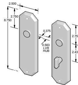
CS-F2308ML-PF – Complete set with mortise lock and spindle. – Patio function. OR TS-F2308ML-PF – Trim set only. No lock.
