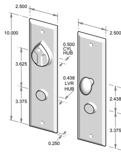
CS-409ML – Complete set with mortise lock, cylinder and spindle. – Single cylinder. OR TS-409ML – Trim set only. No lock.
