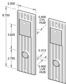
CS-1408ML-DC – Complete set with mortise lock, cylinders and spindle. – Double cylinder. – Non-egress. OR TS-1408ML-DC – Trim set only. No lock.
