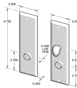
CS-408ML-PF – Complete set with mortise lock and spindle. – Patio function. OR TS-408ML-PF – Trim set only. No lock.
