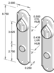
CS-A407ML-DC - Complete set with mortise lock, cylinders and spindle. - Double cylinder. - Non-egress. OR TS-A407ML-DC - Trim set only. No lock.
