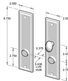
CS-420ML-PF – Complete set with mortise lock and spindle. – Patio function. – Shown with TPC-306. OR TS-420ML-PF – Trim set only. No lock.
