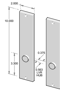
TS-951ML-FD - Trim set only. - Full dummy.
