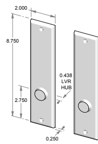
TS-407ML-FD - Trim set only. - Full dummy.
