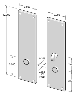
CS-957ML-PF – Complete set with mortise lock and spindle. – Patio function. OR TS-957ML-PF – Trim set only. No lock.
