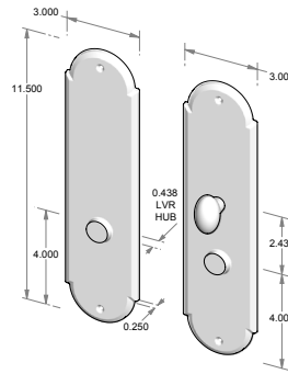
CS-A410ML-PF - Complete set with mortise lock and spindle. - Patio function. OR TS-A410ML-PF - Trim set only. No lock.
