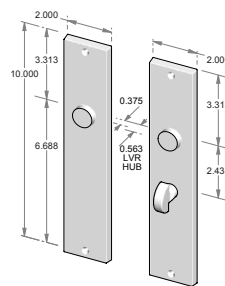
CS-F951ML-PF – Complete set with mortise lock and spindle. – Patio function. OR TS-F951ML-PF – Trim set only. No lock.
