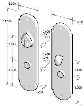
CS-A410ML - Complete set with mortise lock, cylinder and spindle. - Single cylinder. OR TS-A410ML - Trim set only. No lock.
