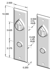
CS-409ML-DC – Complete set with mortise lock, cylinders and spindle. – Double cylinder. – Non-egress. OR TS-409ML-DC – Trim set only. No lock.
