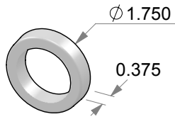
CC-400ML-C Round mortise cylinder collar.
