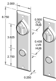
CS-407ML-DC - Complete set with mortise lock, cylinders and spindle. - Double cylinder. - Non-egress. OR TS-407ML-DC - Trim set only. No lock.
