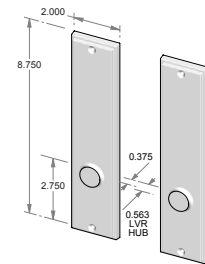
TS-2107ML-FD – Trim set only. – Full dummy.
