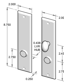
CS-407ML-PF - Complete set with mortise lock and spindle. - Patio function. OR TS-407ML-PF - Trim set only. No lock.
