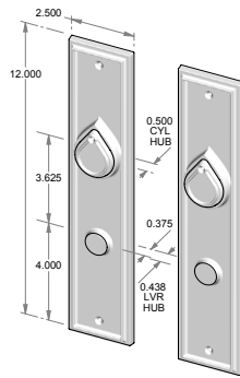
CS-423ML-DC – Complete set with mortise lock, cylinders and spindle. – Double cylinder. – Shown with KC-300. – Non-egress. OR TS-423ML-DC – Trim set only. No lock.
