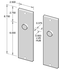
TS-F953ML-FD - Trim set only. - Full dummy.
