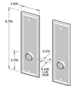
TS-421ML-FD – Trim set only. – Full dummy.
