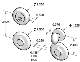
CS-RP402ML - Complete set with mortise lock, cylinder and spindle. - Single cylinder. - Shown with 504ML-C. OR TS-RP402ML - Trim set only. No lock.
