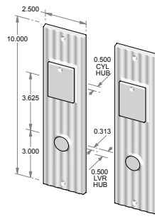
CS-1410ML-DC – Complete set with mortise lock, cylinders and spindle. – Double cylinder. – Non-egress. OR TS-1410ML-DC – Trim set only. No lock.
