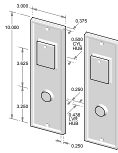
CS-1511ML-DC – Complete set with mortise lock, cylinders and spindle. – Double cylinder. – Non-egress. OR TS-1511ML-DC – Trim set only. No lock.
