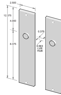
TS-F958ML-FD – Trim set only. – Full dummy.
