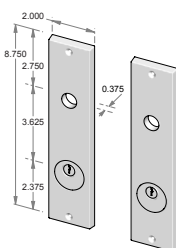
CS-F-N950ML-DC-NKC* – Complete set with mortise lock, cylinders and spindle. – Double cylinder. – Shown without key cover. Must be specified NKC. – Non-egress. OR TS-F-N950ML-DC-NKC – Trim set only. No lock.
