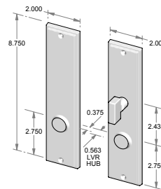
CS-2107ML-PF – Complete set with mortise lock and spindle. – Patio function. OR TS-2107ML-PF – Trim set only. No lock.
