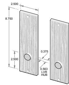
TS-1908ML-FD - Trim set only. - Full dummy.
