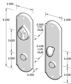
CS-A408ML - Complete set with mortise lock, cylinder and spindle. - Single cylinder. OR TS-A408ML - Trim set only. No lock.
