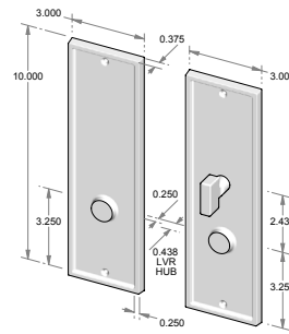
CS-1511ML-PF – Complete set with mortise lock and spindle. – Patio function. OR TS-1511ML-PF – Trim set only. No lock.
