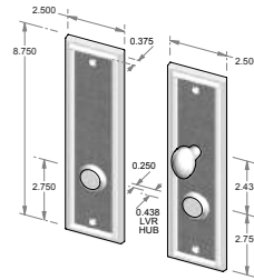
CS-2408ML-PF – Complete set with mortise lock and spindle. – Patio function. – Shown with TPC-306. OR TS-2408ML-PF – Trim set only. No lock.
