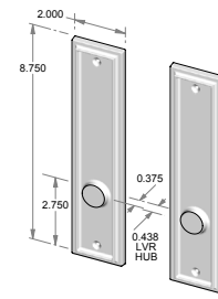
TS-420ML-FD – Trim set only. – Full dummy.
