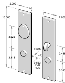
CS-951ML - Complete set with mortise lock, cylinder and spindle. - Single cylinder. OR TS-951ML - Trim set only. No lock.
