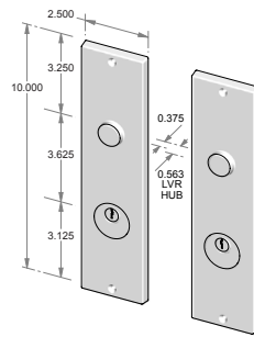
CS-F952ML-DC-NKC* – Complete set with mortise lock, cylinders and spindle. – Double cylinder. – Shown without key cover. Must be specified NKC. – Non-egress. OR TS-F952ML-DC-NKC – Trim set only. No lock.
