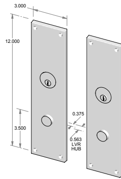
CS-957ML-DC-NKC* – Complete set with mortise lock, cylinders and spindle. – Double cylinder. – Shown without key cover. Must be specified NKC. – Non-egress. OR TS-957ML-DC-NKC – Trim set only. No lock.
