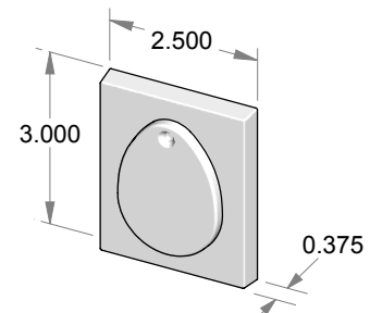
CC-9510ML-C Contemporary cylinder trim w/ key cover.
