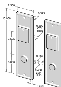
CS-1510ML-DC – Complete set with mortise lock, cylinders and spindle. – Double cylinder. – Non-egress. OR TS-1510ML-DC – Trim set only. No lock.
