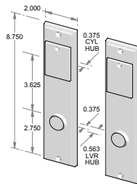
CS-2107ML-DC – Complete set with mortise lock, cylinders and spindle. – Double cylinder. – Non-egress. OR TS-2107ML-DC – Trim set only. No lock.
