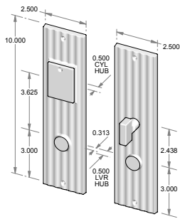
CS-1410ML – Complete set with mortise lock, cylinder and spindle. – Single cylinder. OR TS-1410ML – Trim set only. No lock.
