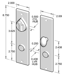
CS-E407ML – Complete set with mortise lock, cylinder and spindle. – Single cylinder. OR TS-E407ML – Trim set only. No lock.
