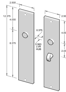
CS-F958ML-PF – Complete set with mortise lock and spindle. – Patio function. OR TS-F958ML-PF – Trim set only. No lock.
