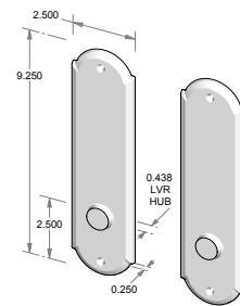
TS-A408ML-FD - Trim set only. - Full dummy.
