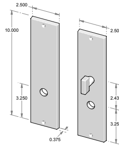
CS-N952ML-PF – Complete set with mortise lock and spindle. – Patio function. OR TS-N952ML-PF – Trim set only. No lock.
