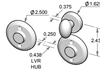
CS-RP402ML-PF - Complete set with mortise lock and spindle. - Patio function. OR TS-RP402ML-PF - Trim set only. No lock.
