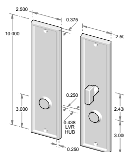
CS-1510ML-PF – Complete set with mortise lock and spindle. – Patio function. OR TS-1510ML-PF – Trim set only. No lock.
