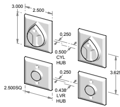
CS-402ML-DC - Complete set with mortise lock, cylinders and spindle. - Double cylinder. - Shown with 509ML-C. - Non-egress. OR TS-402ML-DC - Trim set only. No lock.
