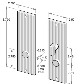
CS-1408ML-PF – Complete set with mortise lock and spindle. – Patio function. OR TS-1408ML-PF – Trim set only. No lock.
