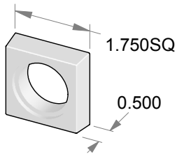
CC-405ML-C Square mortise cylinder collar.
