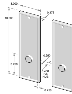
TS-1511ML-FD – Trim set only. – Full dummy.
