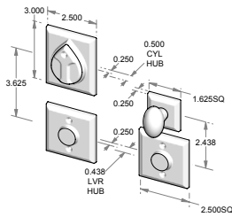
CS-402ML - Complete set with mortise lock, cylinder and spindle. - Single cylinder. - Shown with 509ML-C. OR TS-402ML - Trim set only. No lock.
