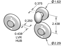
CS-RP225ML-PF – Complete set with mortise lock and spindle. – Patio function. OR TS-RP225ML-PF – Trim set only. No lock.
