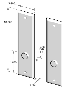
TS-409ML-FD – Trim set only. – Full dummy.
