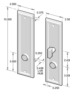
CS-2510ML-PF – Complete set with mortise lock and spindle. – Patio function. OR TS-2510ML-PF – Trim set only. No lock.
