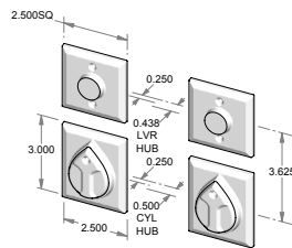
CS-F402ML-DC – Complete set with mortise lock, cylinders and spindle. – Double cylinder. – Shown with 509ML-C. OR TS-F402ML-DC – Trim set only. No lock.
