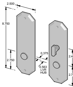
CS-2308ML-PF - Complete set with mortise lock and spindle. - Patio function. OR TS-2308ML-PF - Trim set only. No lock.
