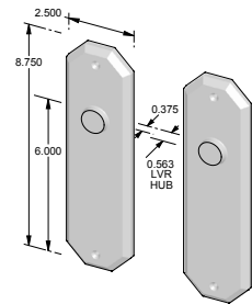
TS-F2308ML-FD – Trim set only. – Full dummy.
