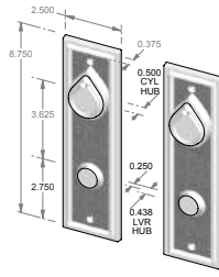
CS-2408ML-DC – Complete set with mortise lock, cylinders and spindle. – Double cylinder. – Shown with KC-300. – Non-egress. OR TS-2408ML-DC – Trim set only. No lock.
