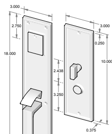
CS-1519 - Complete set with mortise lock, cylinder and spindle. - Single cylinder. - Shown w/std GH-983. OR TS-1519 - Trim set only. No lock.
