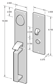
CS-901 - Complete set with mortise lock, cylinder and spindle. - Single cylinder. - Shown w/std GH-900. OR TS-901 - Trim set only. No lock.
