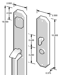
CS-2300 - Complete set with mortise lock, cylinder and spindle. - Single cylinder. - Shown w/std GH-9409. OR TS-2300 - Trim set only. No lock.
