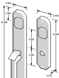
CS-2300DC - Complete set with mortise lock, cylinders and spindle. - Double cylinder. OR TS-2300DC - Trim set only. No lock.
