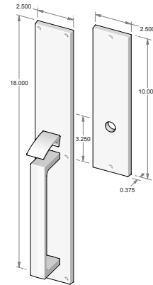
TS-N911FD – Trim set only. – Full dummy. – Also available without thumb piece.
