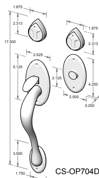
CS-OP704DC – Complete set with mortise lock, cylinders and spindle. – Double cylinder. OR TS-OP704DC – Trim set only. No lock.
