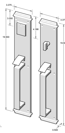
CS-741HH - Complete set with mortise lock and cylinder. - Single cylinder. - Double grip handle. OR TS-741HH - Trim set only. No lock.
