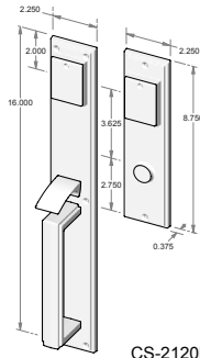
CS-2120DC - Complete set with mortise lock, cylinders and spindle. - Double cylinder. OR TS-2120DC - Trim set only. No lock.
