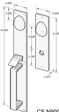
CS-N900DC – Complete set with mortise lock, cylinders and spindle. – Double cylinder. OR TS-N900DC – Trim set only. No lock.
