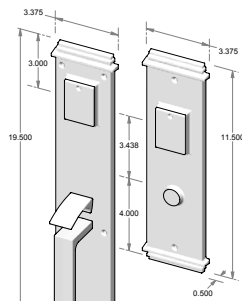
CS-741DC - Complete set with mortise lock, cylinders and spindle. - Double cylinder. OR TS-741DC - Trim set only. No lock.
