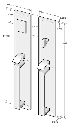
CS-1519HH - Complete set with mortise lock and cylinder. - Single cylinder. - Double grip handle. OR TS-1519HH - Trim set only. No lock.
