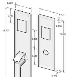
CS-1519DC - Complete set with mortise lock, cylinders and spindle. - Double cylinder. OR TS-1519DC - Trim set only. No lock.
