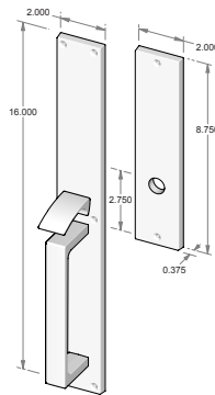
TS-N900FD – Trim set only. – Full dummy. – Also available without thumb piece.
