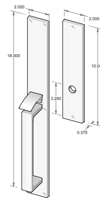
TS-N910FD – Trim set only. – Full dummy. – Also available without thumb piece.
