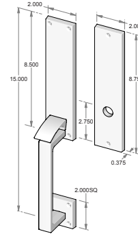
TS-N904FD – Trim set only. – Full dummy. – Also available without thumb piece.
