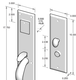
CS-701R - Complete set with mortise lock, cylinder and spindle. - Single cylinder. - Shown w/std GH-700. OR TS-701R - Trim set only. No lock.
