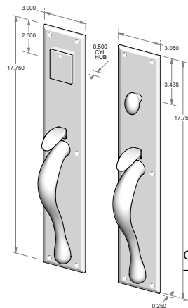
CS-701R - Complete set with mortise lock, cylinder and spindle. - Single cylinder. - Shown w/std GH-700. OR TS-701R - Trim set only. No lock.
