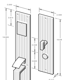
CS-1418 - Complete set with mortise lock, cylinder and spindle. - Single cylinder. - Shown w/std GH-983. OR TS-1418 - Trim set only. No lock.
