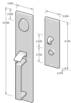
CS-902 - Complete set with mortise lock, cylinder and spindle. - Single cylinder. - Shown w/std GH-900. OR TS-902 - Trim set only. No lock.
