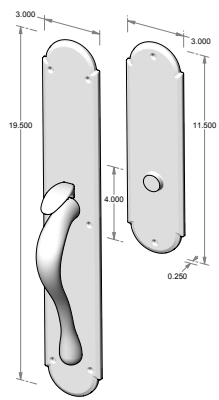
TS-A701FD - Trim set only. - Full dummy. - Also available w/o thumb piece.
