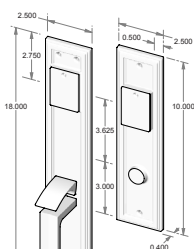
CS-2518DC - Complete set with mortise lock, cylinders and spindle. - Double cylinder. OR TS-2518DC - Trim set only. No lock.
