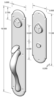
CS-A701DC - Complete set with mortise lock, cylinders and spindle. - Double cylinder. OR TS-A701DC - Trim set only. No lock.
