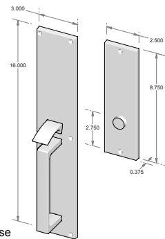
TS-902FD - Trim set only. - Full dummy. - Also available w/o thumb piece.
