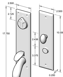
CS-700 – Complete set with mortise lock, cylinder and spindle. – Single cylinder. – Shown w/std GH-700. OR TS-700 – Trim set only. No lock.
