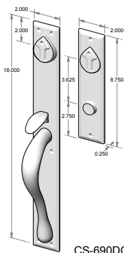
CS-690DC – Complete set with mortise lock, cylinders and spindle. – Double cylinder. OR TS-690DC – Trim set only. No lock.
