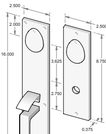
CS-N901DC – Complete set with mortise lock, cylinders and spindle. – Double cylinder. OR TS-N901DC – Trim set only. No lock.
