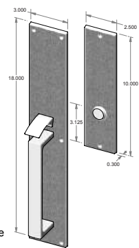
TS-2203FD - Trim set only. - Full dummy. - Also available w/o thumb piece.
