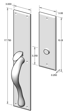
TS-701FD - Trim set only. - Full dummy. - Also available without thumb piece.
