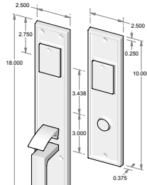
CS-1518DC – Complete set with mortise lock, cylinders and spindle. – Double cylinder. OR TS-1518DC – Trim set only. No lock.
