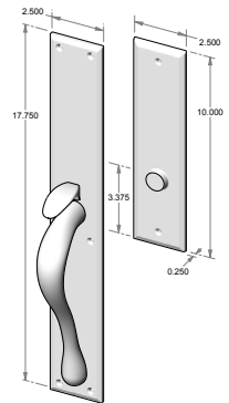
TS-700FD – Trim set only. – Full dummy. – Also available w/o thumb piece.
