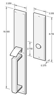
TS-2120FD - Trim set only. - Full dummy. - Also available w/o thumb piece.
