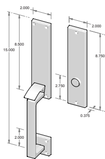
TS-904FD - Trim set only. - Full dummy. - Also available w/o thumb piece.
