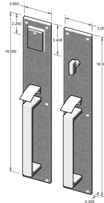
CS-2203HH - Complete set with mortise lock and cylinder. - Single cylinder. - Double grip handle. - Shown w/KC-2200. OR TS-2203HH - Trim set only. No lock.
