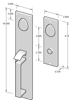
CS-902DC - Complete set with mortise lock, cylinders and spindle. - Double cylinder. OR TS-902DC - Trim set only. No lock.
