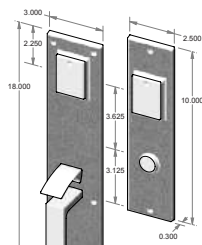
CS-2203DC - Complete set with mortise lock, cylinders and spindle. - Double cylinder. - Shown w/KC-700. OR TS-2203DC - Trim set only. No lock.
