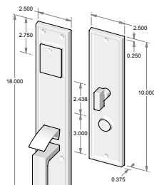
CS-1518 – Complete set with mortise lock, cylinder and spindle. – Single cylinder. – Shown w/std GH-983. OR TS-1518 – Trim set only. No lock.
