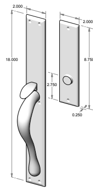
TS-690FD – Trim set only. – Full dummy. – Also available w/o thumb piece.
