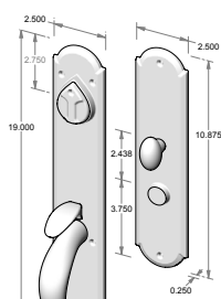
CS-A700 – Complete set with mortise lock, cylinder and spindle. – Single cylinder. – Shown w/std GH-700. OR TS-A700 – Trim set only. No lock.
