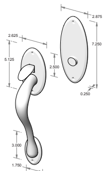
TS-OP704FD – Trim set only. – Full dummy. – Also available w/o thumb piece.
