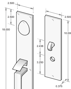
CS-N911 – Complete set with mortise lock, cylinder and spindle. – Single cylinder. – Shown w/std GH-983. OR TS-N911 – Trim set only. No lock.
