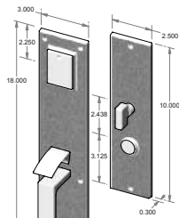
CS-2203 - Complete set with mortise lock, cylinder and spindle. - Single cylinder. - Shown w/KC-700. - Shown w/std GH-983. OR TS-2203 - Trim set only. No lock.
