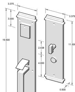
CS-741 - Complete set with mortise lock, cylinder and spindle. - Single cylinder. - Shown w/std GH-983. OR TS-741 - Trim set only. No lock.
