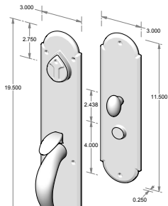
CS-A701 - Complete set with mortise lock, cylinder and spindle. - Single cylinder. - Shown w/std GH-700. OR TS-A701 - Trim set only. No lock.
