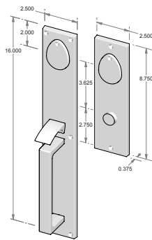
CS-901DC - Complete set with mortise lock, cylinders and spindle. - Double cylinder. OR TS-901DC - Trim set only. No lock.
