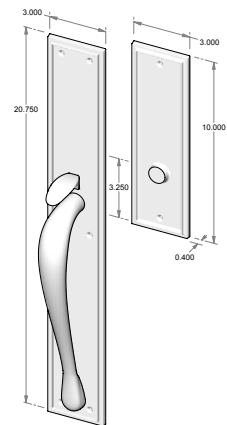
TS-722FD – Trim set only. – Full dummy. – Also available w/o thumb piece.
