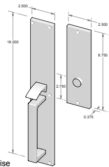
TS-901FD - Trim set only. - Full dummy. - Also available w/o thumb piece.
