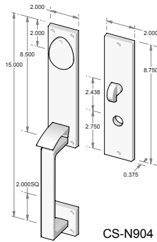
CS-N904 – Complete set with mortise lock, cylinder and spindle. – Single cylinder. – Shown w/std GH-900. OR TS-N904 – Trim set only. No lock.
