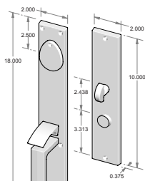
CS-910 – Complete set with mortise lock, cylinder and spindle. – Single cylinder. – Shown w/std GH-983. OR TS-910 – Trim set only. No lock.
