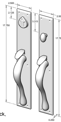
CS-700HH – Complete set with mortise lock and cylinder. – Single cylinder. – Double grip handle. OR TS-700HH – Trim set only. No lock.
