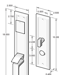
CS-2518 - Complete set with mortise lock, cylinder and spindle. - Single cylinder. - Shown w/std GH-983. OR TS-2518 - Trim set only. No lock.
