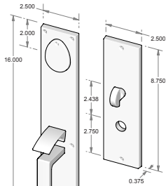
CS-N901 – Complete set with mortise lock, cylinder and spindle. – Single cylinder. – Shown w/std GH-900. OR TS-N901 – Trim set only. No lock.
