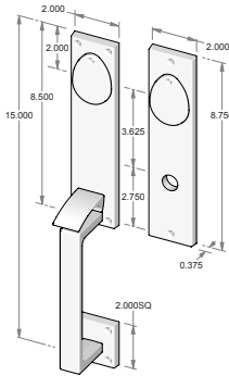
CS-N904DC – Complete set with mortise lock, cylinders and spindle. – Double cylinder. OR TS-N904DC – Trim set only. No lock.
