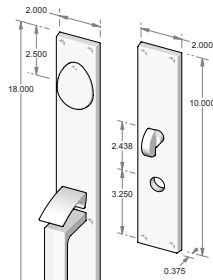
CS-N910 – Complete set with mortise lock, cylinder and spindle. – Single cylinder. – Shown w/std GH-983. OR TS-N910 – Trim set only. No lock.
