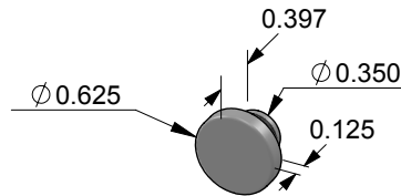
ER-12-PLUG Round screwless release cover.
