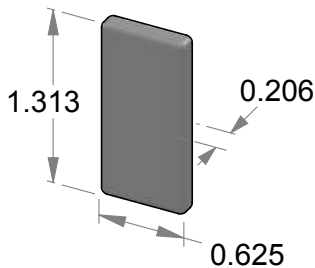
TPC-WTPC-SQ Flush pull turn piece.
