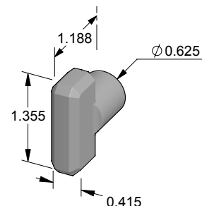
TPC-767 Gem turn piece.
