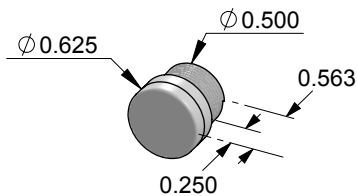
ER-12 Round screwless release cover w/HOUSING.
