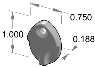
RC-4 Original teardrop release cover.
