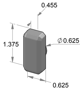
TPC-FP-JADA Jada flush pull turn piece.
