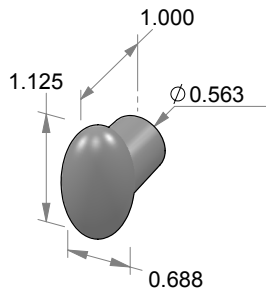
TPC-202 Oval turn piece.
