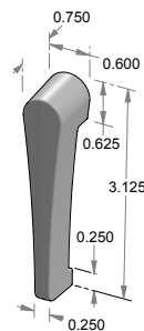
TPC-CW-ADA ADA flush pull turn piece.
