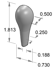
TPC-DT Slider turn piece.
