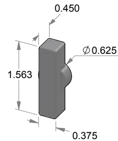
TPC-FP741 Flush pull turn piece.
