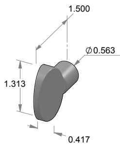
TPC-326 Swedge turn piece.
