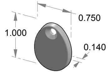
RC-9 Flat face teardrop release cover.
