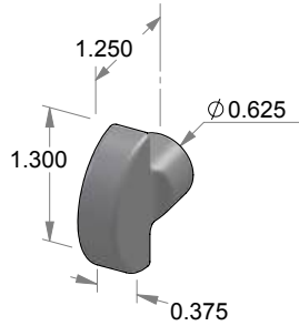
TPC-900 Contemporary turn piece.
