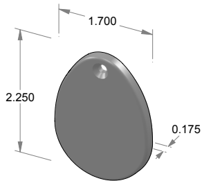
KC-900 Contemporary key cover.
