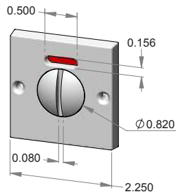
CR-1-INDICATOR Coin release w/ indicator. Shown w/P-925MB (NOT INCLUDED).
