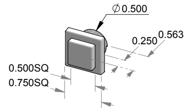
ER-13 Square screwless release cover w/HOUSING.
