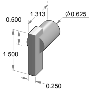
TPC-9102 Slider turn piece.
