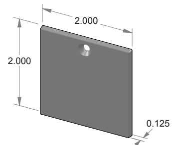
KC-1818 Contemporary square key cover.
