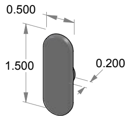
TPC-WTPC-NB Narrow bucket flush pull turn piece.
