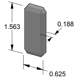
TPC-WTPC-Gem Gem flush pull turn piece.
