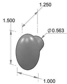
TPC-302 Oval turn piece.
