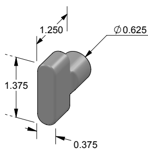
TPC-743 Contemporary Ergo turn piece.
