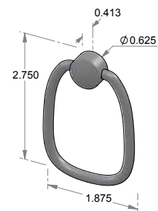
TPC-FR Flap ring flush pull turn piece.
