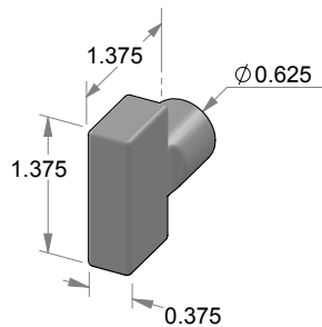
TPC-741 Contemporary turn piece.
