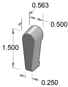
TPC-CW Slider turn piece.
