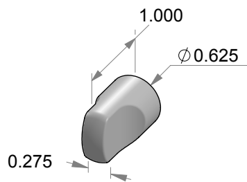
TPC-454 Cylindrical turn piece.
