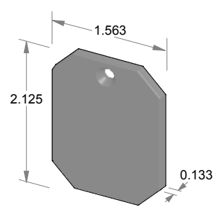
KC-2300 Gem key cover.
