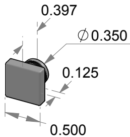
ER-13-PLUG Square screwless release cover.
