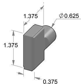
TPC-761 Deco turn piece.
