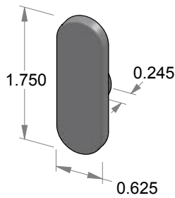
TPC-WTPC Flush pull turn piece.
