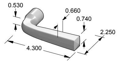
L-106 Square Lever
