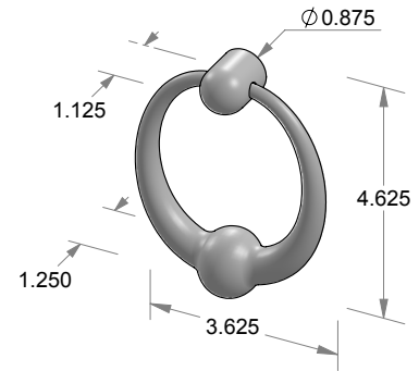
K-212 Ring Pull
