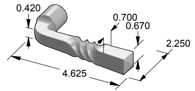
L-123 New Twist Lever
