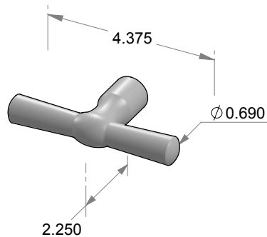
K-230T-H Horizontal Large T-Handle Knob (shown); K-230T-V Vertical Large T-Handle Knob; Specify
