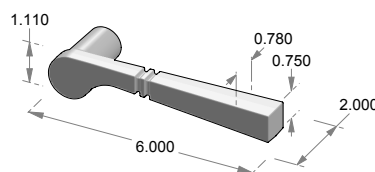
L-109-6 Ring Tail Lever
