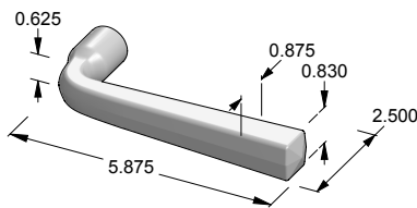
L-115 Large Square Lever
