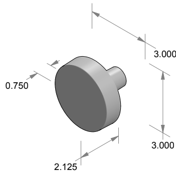
K-237 Large Flat Knob
