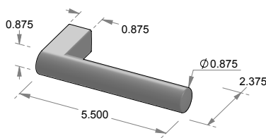
L-165SQ Pettit Lever* Square hub for use w/Novus escutcheon.
