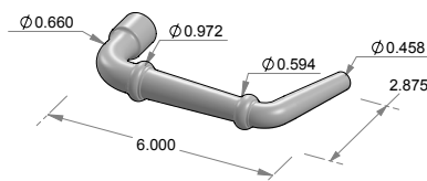
L-143R Harriman Lever w/Return
