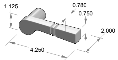
L-109 Ring Tail Lever
