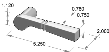
L-109-525 Ring Tail Lever
