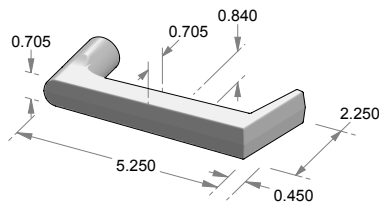
L-122R Metro Lever w/Return
