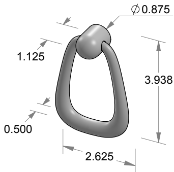
K-213 Ring Pull
