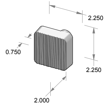
K-235 Corduroy Square Knob
