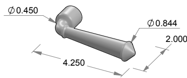
L-127LP Hailey Lever, Low Projection
