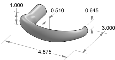
L-107 Large Hook Lever
