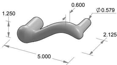
L-108R Chubba Lever w/Return
