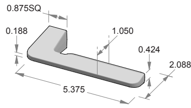
L-N254 Swedge Lever. Square hub for use w/Novus escutcheon.
