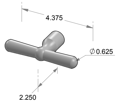
K-229T-H Horizontal Small T-Handle Knob (shown); K-229T-V Vertical Small T-Handle Knob; Specify
