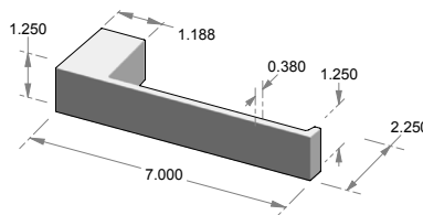
L-183SQ Chilco Lever* Square hub for use w/Novus escutcheon.
