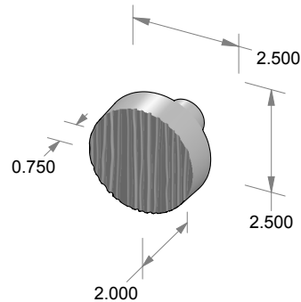
K-234 Large Corduroy Flat Knob
