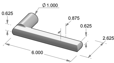
L-N178 Malad Lever* 1" Round hub for use w/Novus escutcheon.
