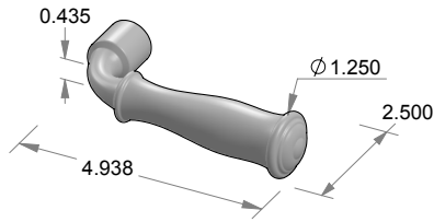
L-163LP Shoshone Lever, Low Projection
