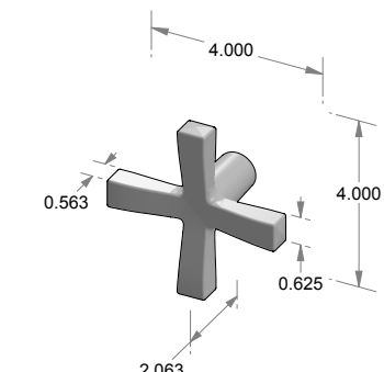
K-CROSS Cross Knob
