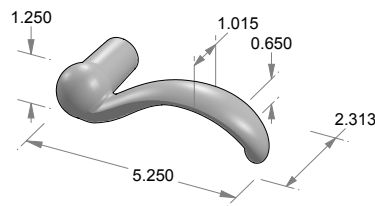
L-136 Snake River Lever
