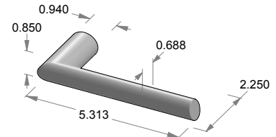
L-N252RH Clearwater Lever. 0.940" Round hub for use w/Novus escutcheon. Right hand shown.
