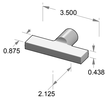
K-741T-H Horizontal T-Handle Knob (shown); K-741T-V Vertical T-Handle; Specify
