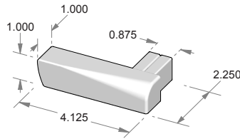
DEREUS-L-185SQ-LH De Reus collaboration Kyoto Kata I Lever* Square hub for use w/Novus escutcheon. Specify L-185SQ-RH (right hand) or L-185SQ-LH (left hand). Left hand shown.
