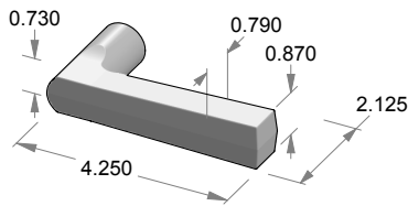
L-132 Little Metro Lever
