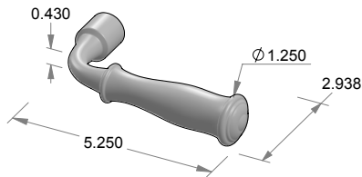
L-163 Shoshone Lever
