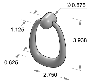
K-218 Ring Pull
