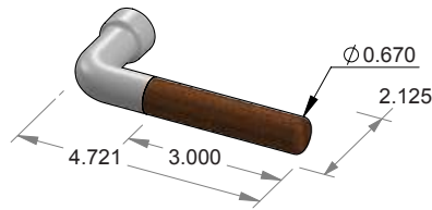
L-W201 Tube Wood Handle Lever
