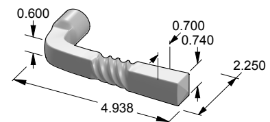
L-137 Extended Twist Lever
