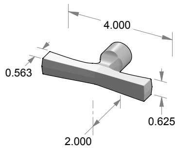
K-228T-H Horizontal Small T-Handle Knob (shown); K-228T-V Vertical Small T-Handle Knob; Specify
