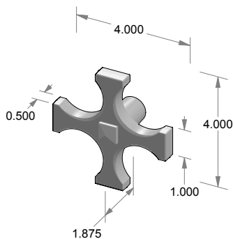
K-CROSS-FLT Flat Cross Knob
