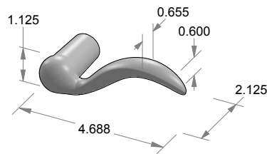
L-102 Squirrel Tail Lever
