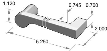
L-109R Ring Tail Lever w/Return
