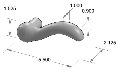
L-108 Chubba Lever
