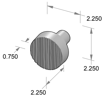
K-233 Small Corduroy Flat Knob
