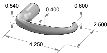
L-104 Small Hook Lever
