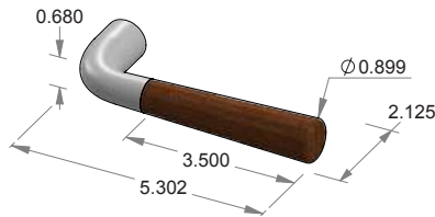
L-W200 Tapered Wood Handle Lever
