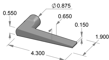
VICA-L-301 Vica by Annabelle Selldorf collaboration lever
