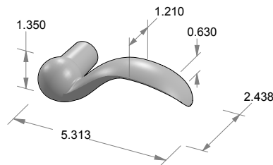
L-105 Beaver Tail Lever
