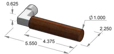
L-W206 Pioneer Wood Handle Lever
