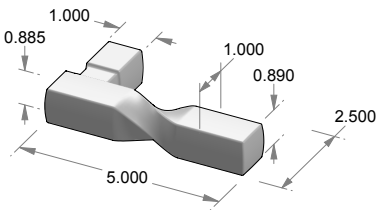
L-158SQ Trail Creek Lever* Square hub for use w/Novus escutcheon.
