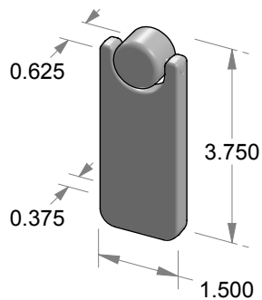
K-251 Flap Pull
