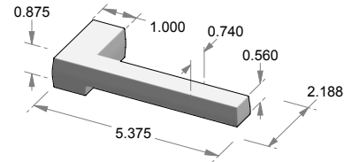
L-164SQ Bullion Lever* Square hub for use w/Novus escutcheon.
