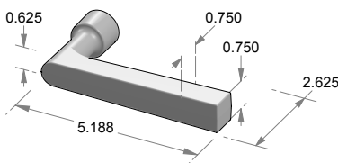
L-N181 Palouse Lever* 1" Round hub for use w/Novus escutcheon.
