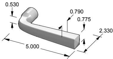
L-121 Medium Square Lever
