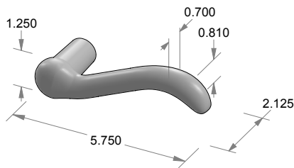
L-168 Fairfield Lever
