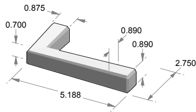
L-166SQ Mesa Lever* Square hub for use w/Novus escutcheon.
