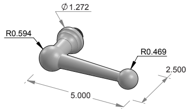
L-N253 Villa Lever. 0.940" Round hub for use w/Novus escutcheon.
