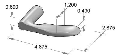
L-126 Silver Creek Lever
