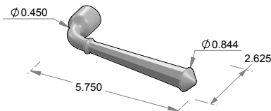
L-128.575 Stanley Lever
