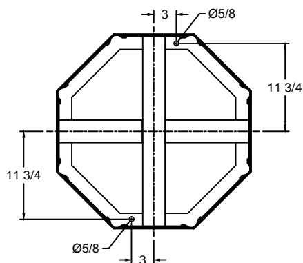
COVER REMOVED (ANCHOR HOLES IN BASE SHOWN)
