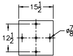
SURFACE MOUNT INSTALLATION WITH BASEPLATE
