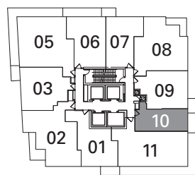
LEVELS 10-18/ 21-30/33-42/46-50 387 SQ. FT. BALCONY 52 SQ. FT. TYPICAL FLOOR
