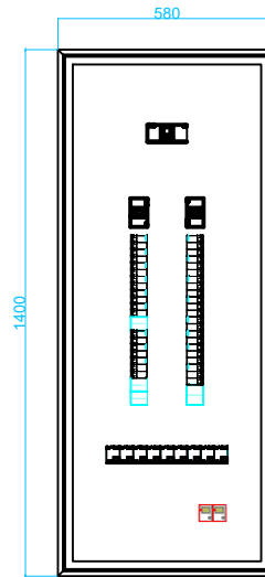
VISTA FRONTAL (SIN PUERTA EXTERIOR)
