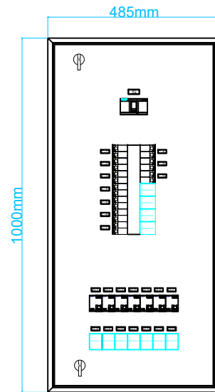
VISTA FRONTAL (SIN PUERTA EXTERIOR)
