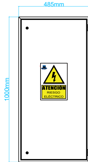
VISTA FRONTAL
