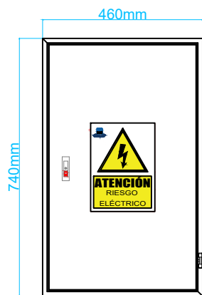
VISTA FRONTAL
