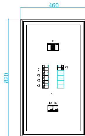
VISTA FRONTAL (SIN PUERTA EXTERIOR)
