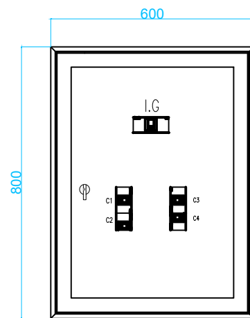
VISTA FRONTAL (SIN PUERTA EXTERIOR)
