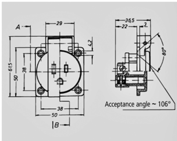
Drawing 1 MB 421
