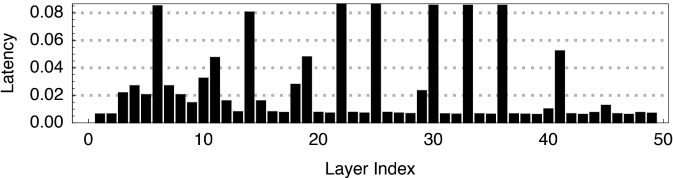
Emotion-FerPlus running on TITAN_V using batch size 4
