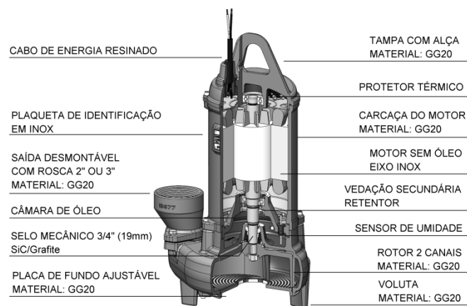
FBS-NG 400, 500, 600, 700, 800 e 900
