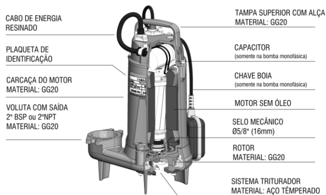
FBS-NG-JAC 300
