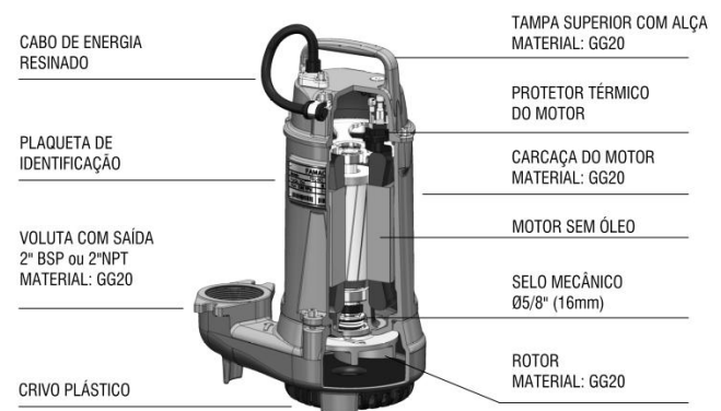
FBS-NG 250 e 300
