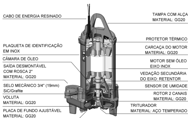
FBS-NG-JAC 400, 500 e 600
