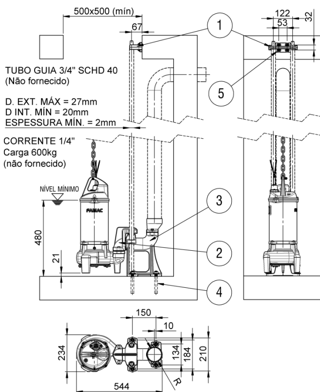
FBS-NG 400, 500, 600, 700, 800 e 900
