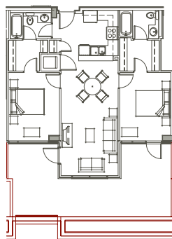
FLOOR 2: ≈ 913 sq ft
