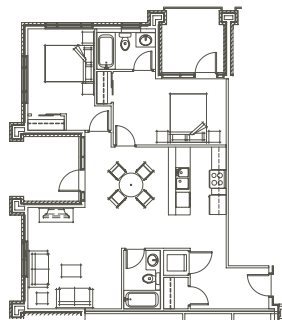
GROUND FLOOR C-1G: ≈ 1,057 sq ft
