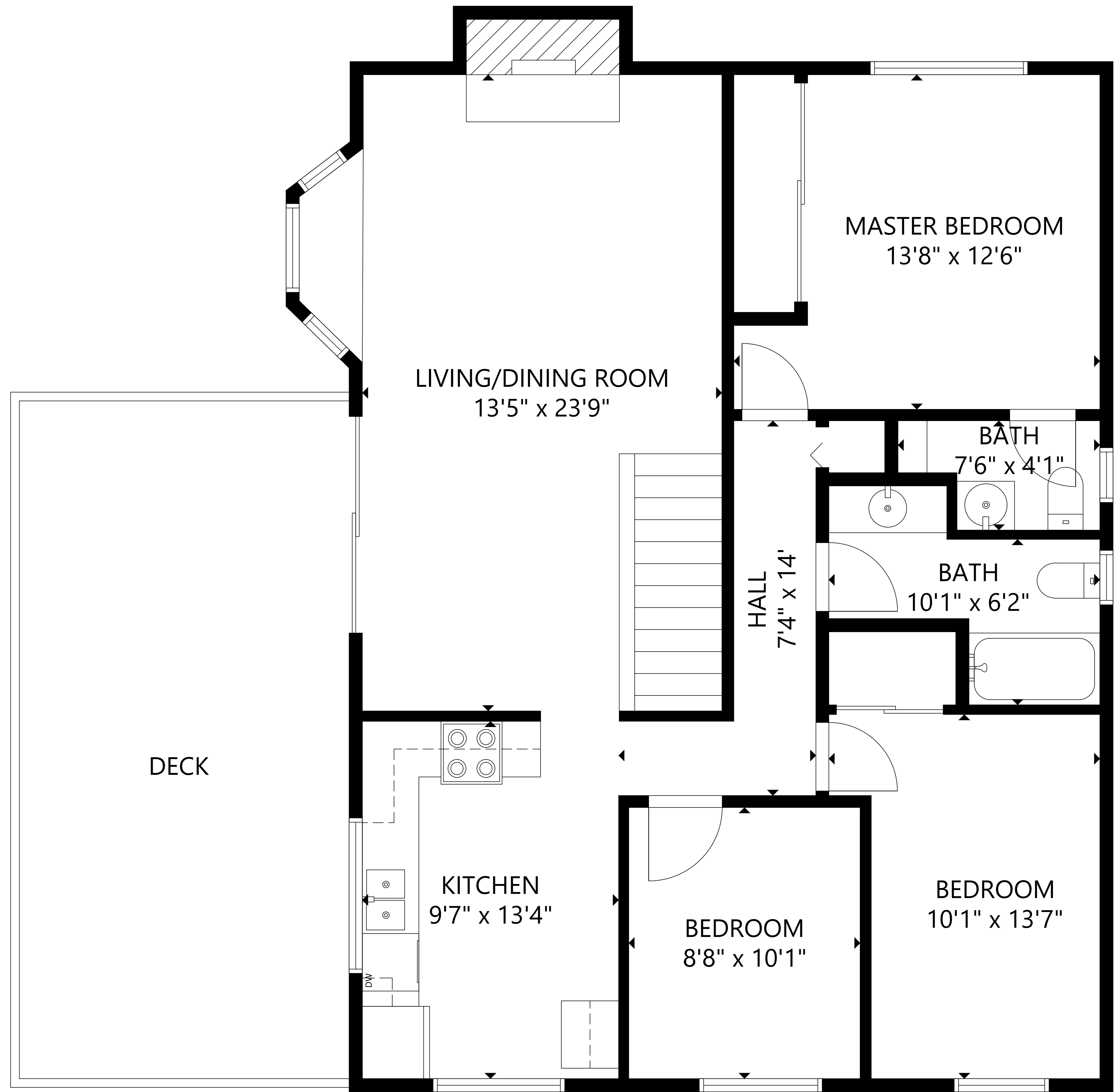
UPPER FLOOR
