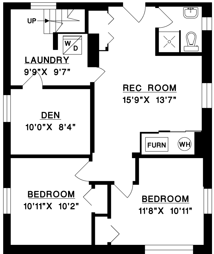
LOWER FLOOR
