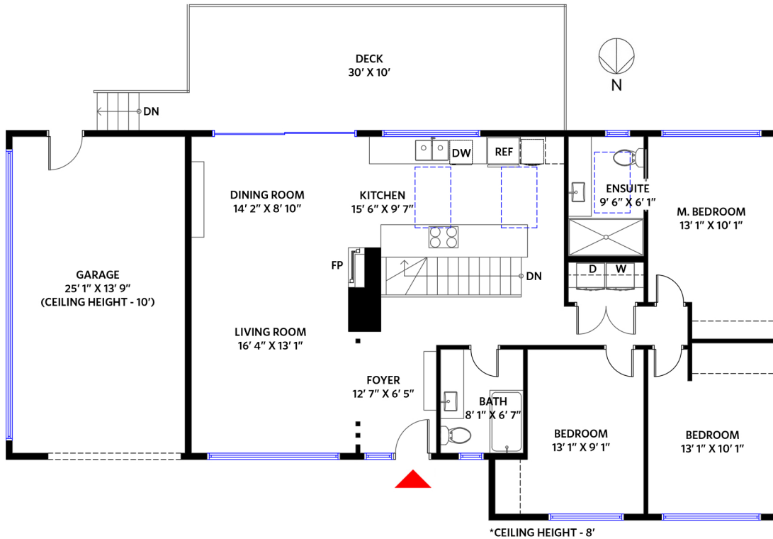
MAIN FLOOR 1,362 SQ.FT.
