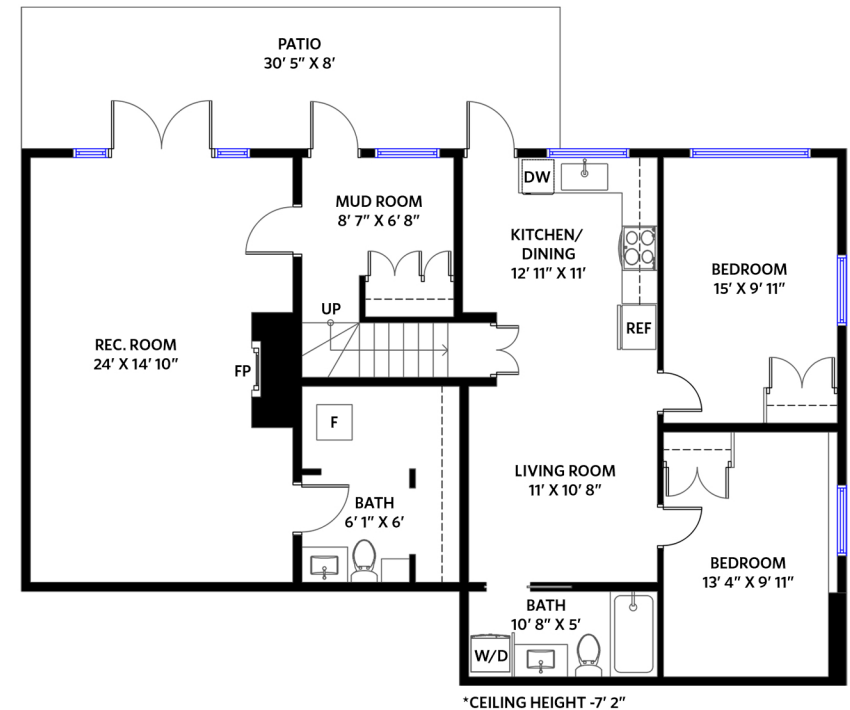
LOWER FLOOR 1,362 SQ.FT.
