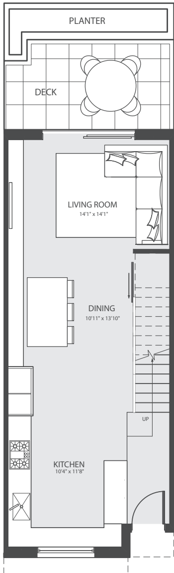
First Level 534 sf / Deck 133 sf
