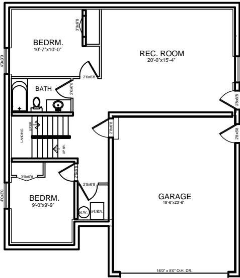
BASEMENT = 890 SQ. FT.
