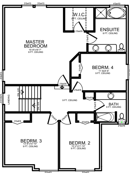
UPPER FLOOR = 1190 SQ. FT.
